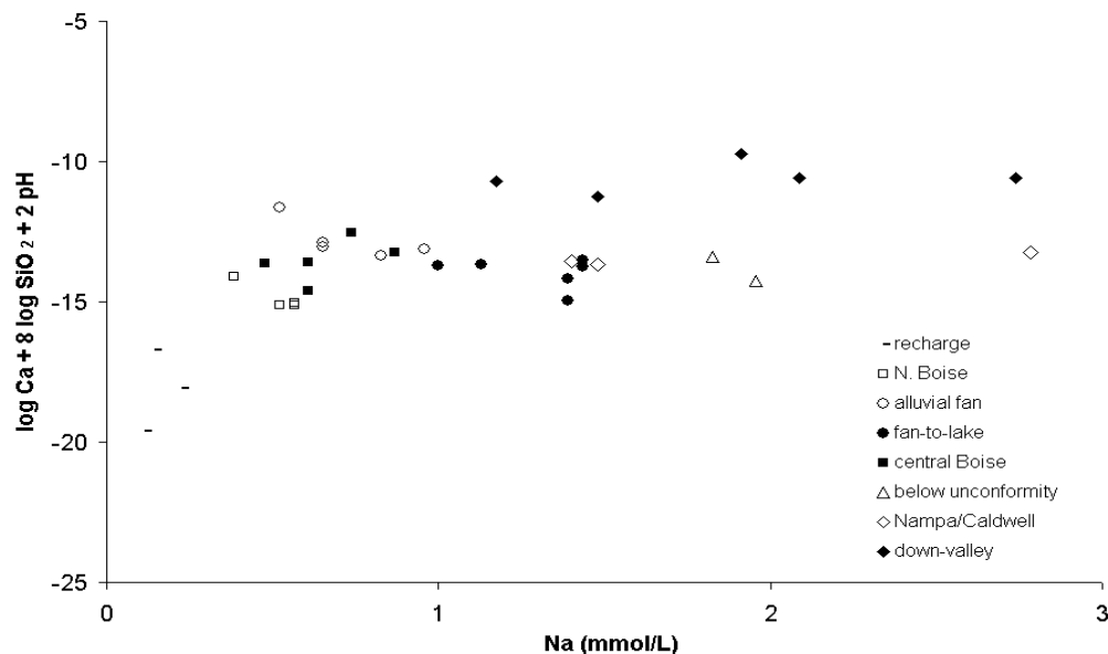
Figure 12. Changes in the kaolinite-smectite reaction quotient for regional ground waters in the Treasure Valley. After Garrels (1967).
