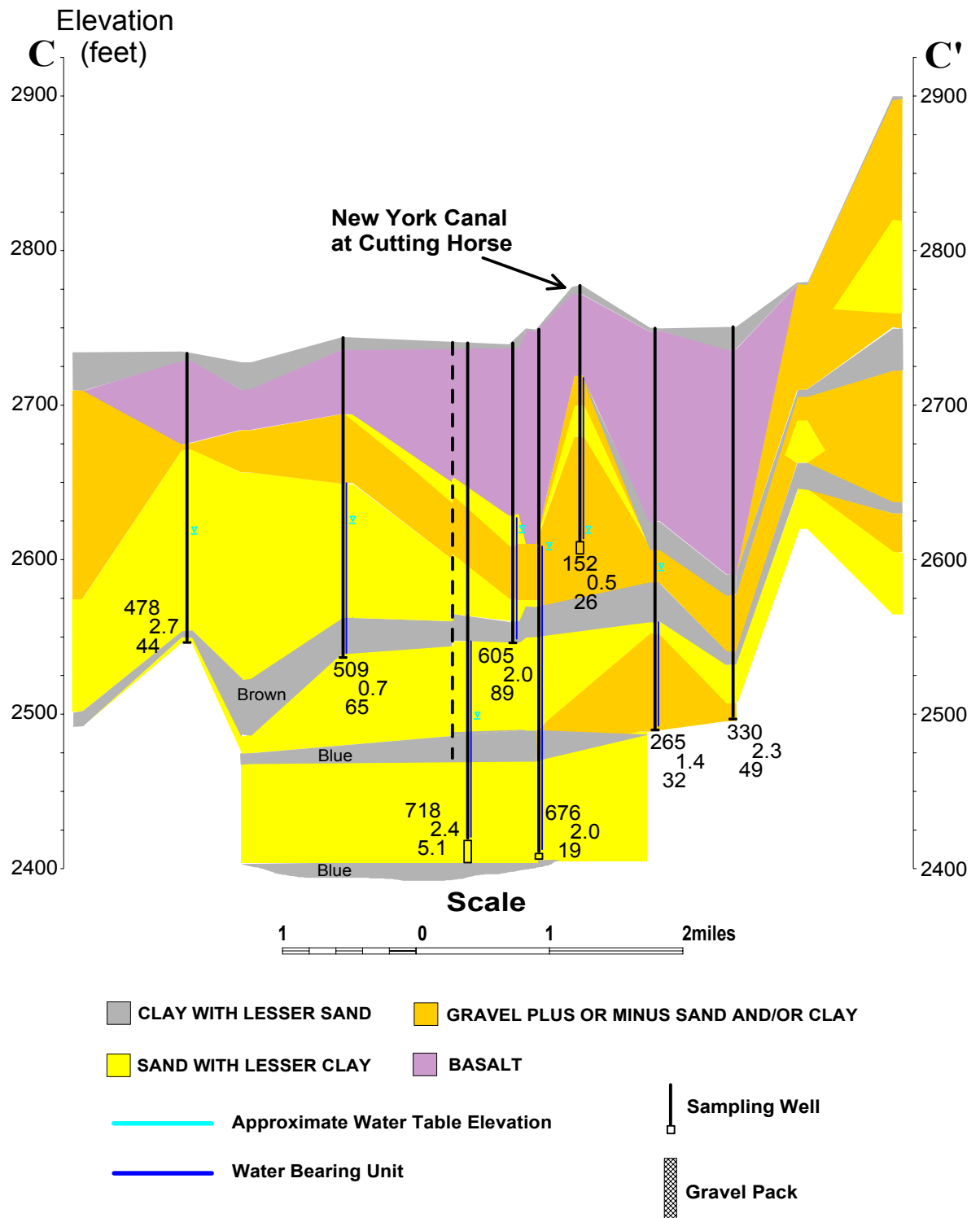
Figure 8. Ground water chemistry and aquifer stratigraphy near the NYC at Cutting Horse Road. The geologic cross-section C-C' is shown in Figure 2. Names and locations of sampling wells are shown in Figure 1.
