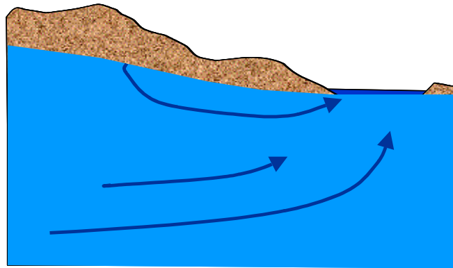
Figure 4: Schematic diagram showing recharge in a regional discharge area.
