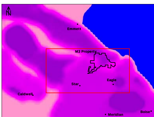
(C) Model 2 Layers 5-6 K (ft/d)
