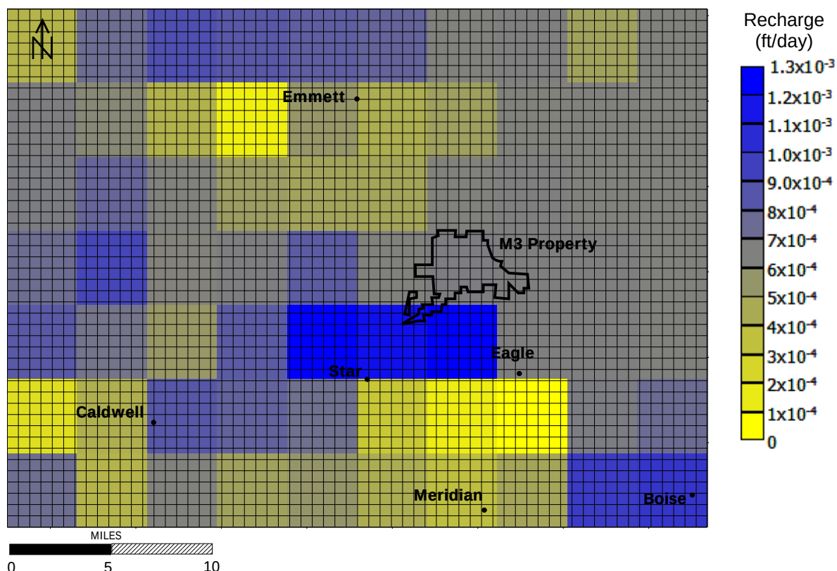
Figure 25. Shaded cell map of total estimated recharge within the model domain from all sources.
