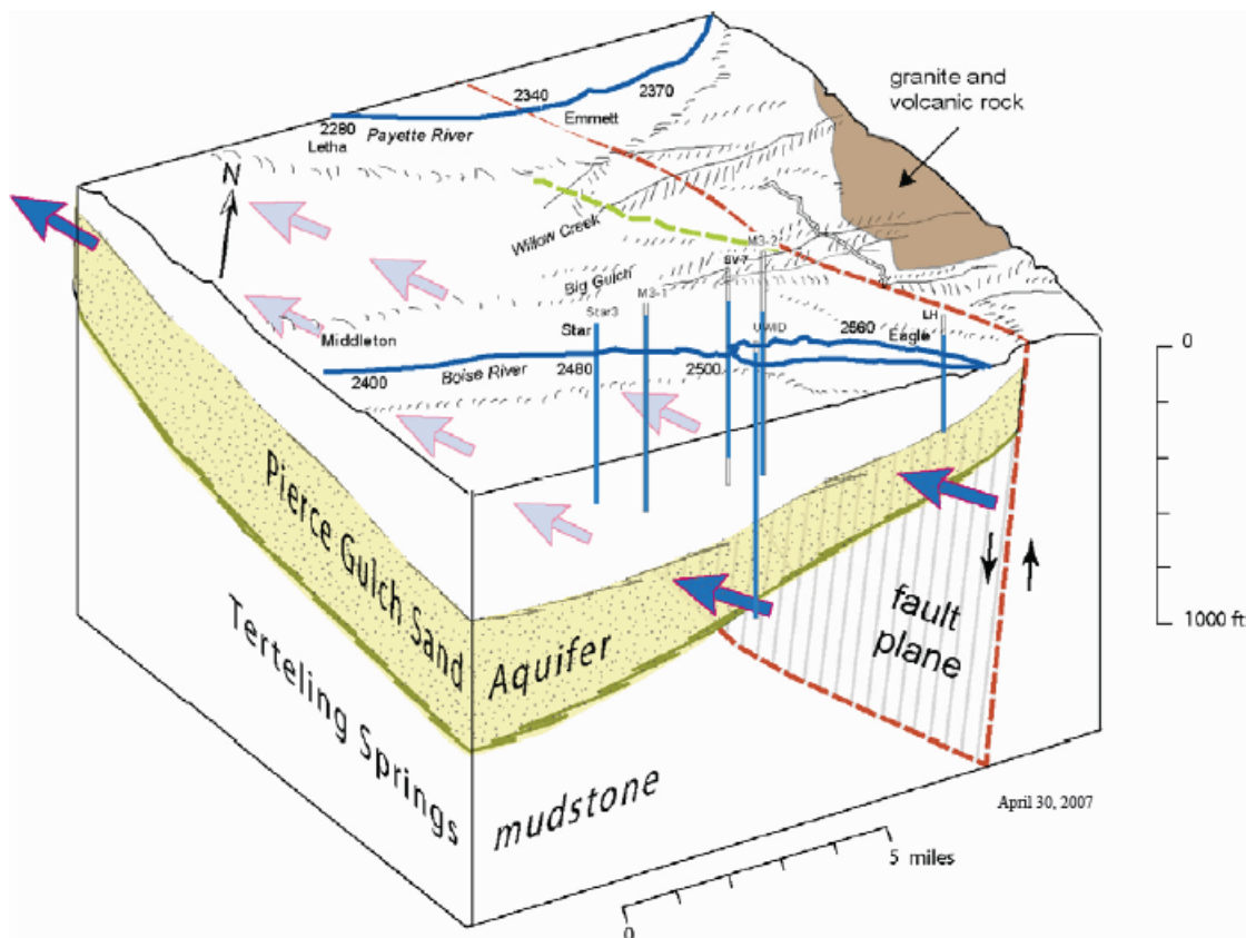
Figure 6. Three-dimensional block diagram displaying the sub-surface geologic features between the Boise River Basin and the Payette River Basin. Figure is Figure 4 from Squires et al. (2007).
