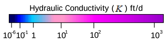
(C) Model 2 Layers 5-6 K (ft/d)
