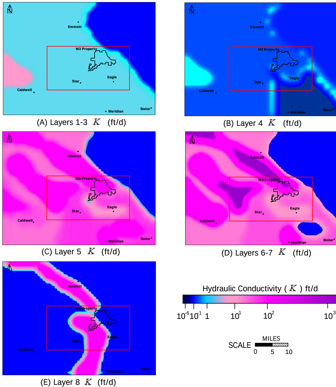
Figure 28. Hydraulic conductivity distributions assigned within the model domain by layer for the steady-state and the final quasi-steady-state model. (A) Calibrated K for Layers 1, 2, and 3. (B) Calibrated K for Layer 4. (C) Calibrated K for Layer 5. (D) Calibrated K for Layers 6 and 7. (E) Calibrated K for Layer 8. confined aquifers, the storativity is on the order of 0.005 or less (Fetter, 1998).
