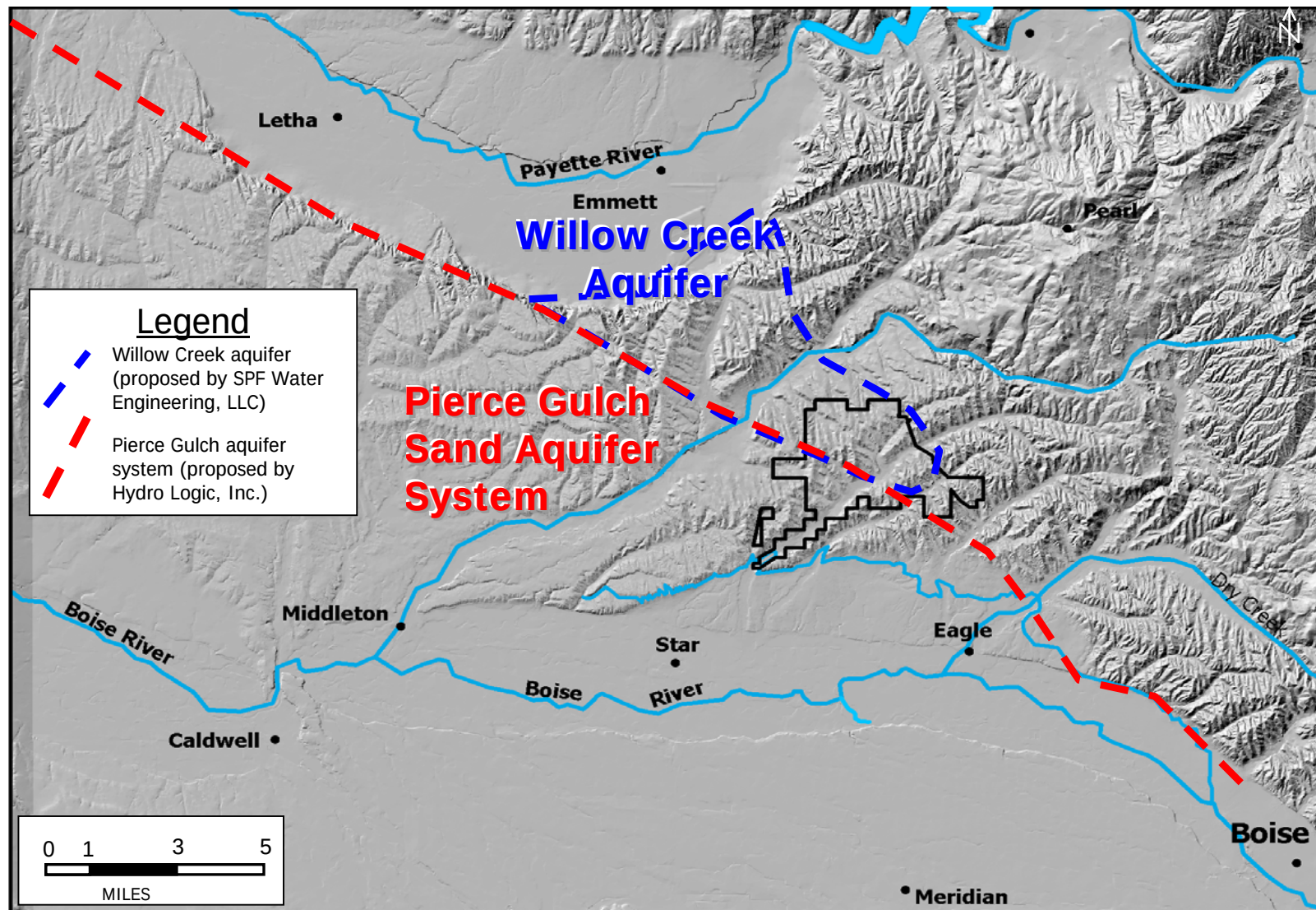
Figure 11. Map of the main aquifers within the model domain. The Pierce Gulch Sand aquifer system is located under the southwestern half of the M3 Eagle property and dips to the southwest. The Willow Creek Aquifer is located under the northeastern half of the M3 Eagle property. The lateral extent of both aquifers to the northwest is relatively unknown. NED map (National Elevation Dataset map) adapted from U.S. Geological Survey (2006).
