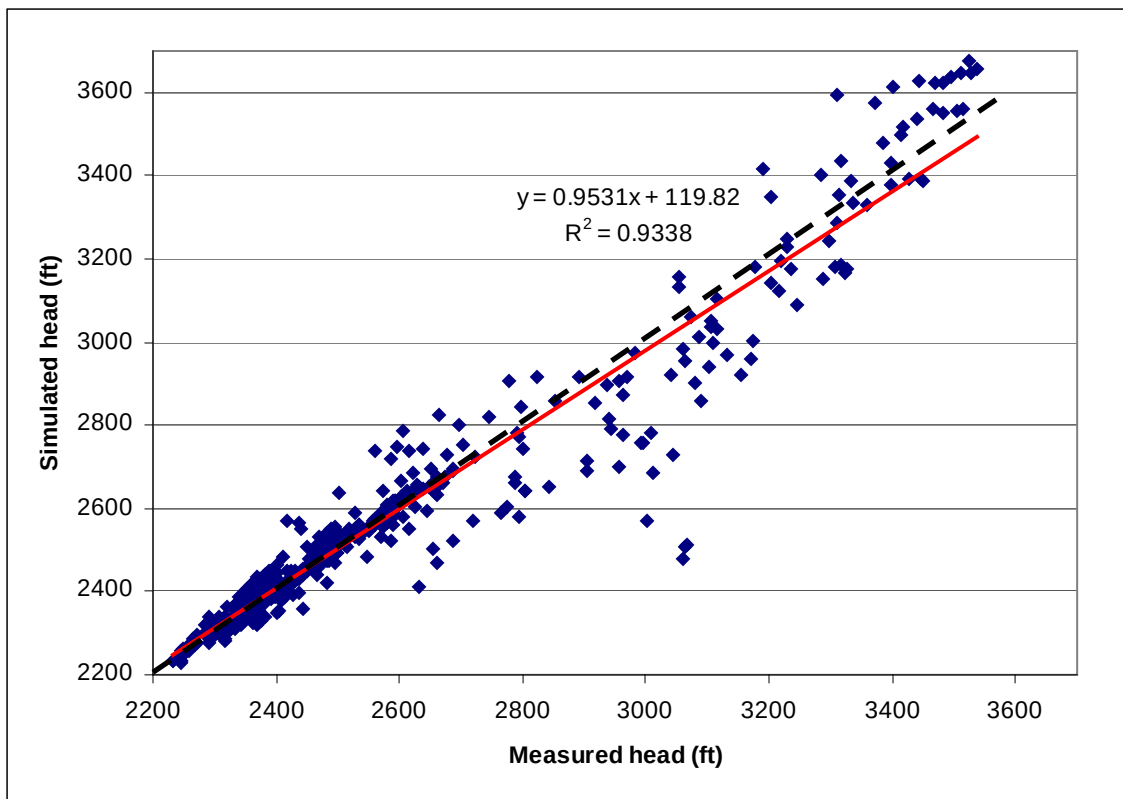
Figure 45. Arithmetic plot of simulated water levels for Model 6 versus water levels measured in 2006.
