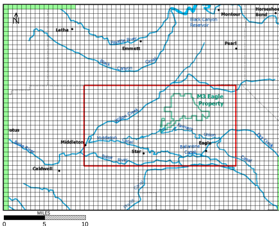
Figure 23. General-head boundaries in the quasi-steady-state model grid Layer 6. The green cells represent the general heads.
