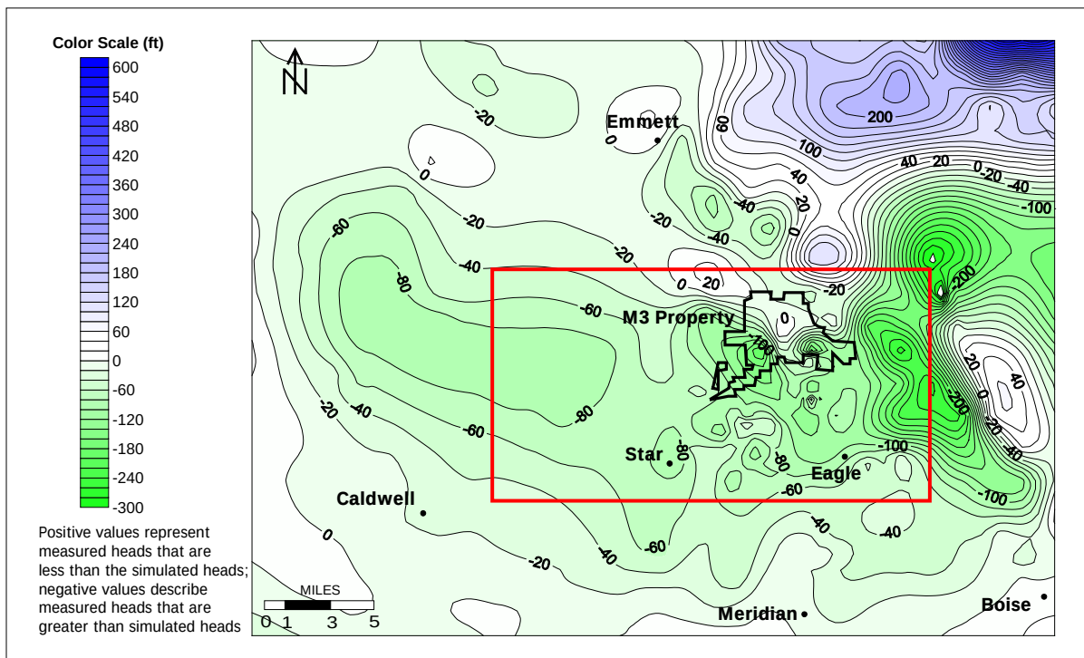
(H) Residuals detailing the difference between simulated and measured head values for Quasi-Steady-State Model 5d.
