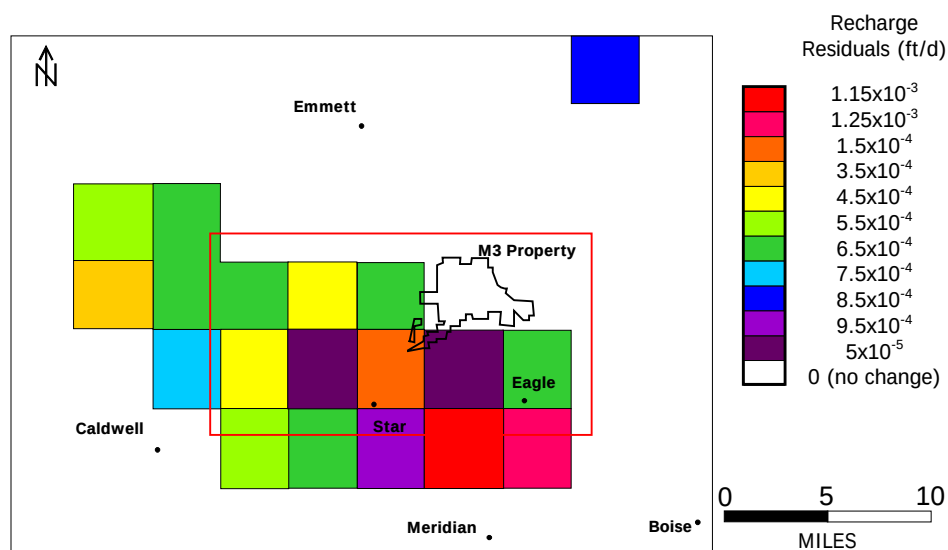
Figure 38. Changes in recharge within the model domain between Models 2 and 3 plotted as numerical differences (residuals).
