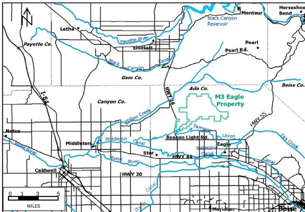
Figure 7. Map of the M3 Eagle Big Gulch Ground Water Flow Model domain showing the location of the M3 Eagle property. The future development, M3 Eagle, is outlined in green in the central area of the map.
