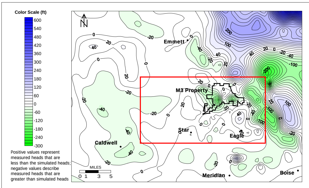
(D) Residuals detailing the difference between simulated and measured head values for Quasi-Steady-State Model 4.
