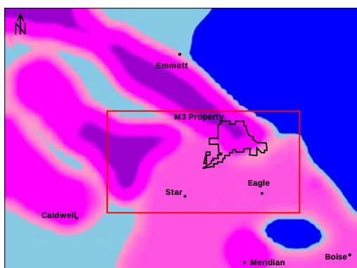
(C) Model 3 Layers 5-6 K (ft/d)
