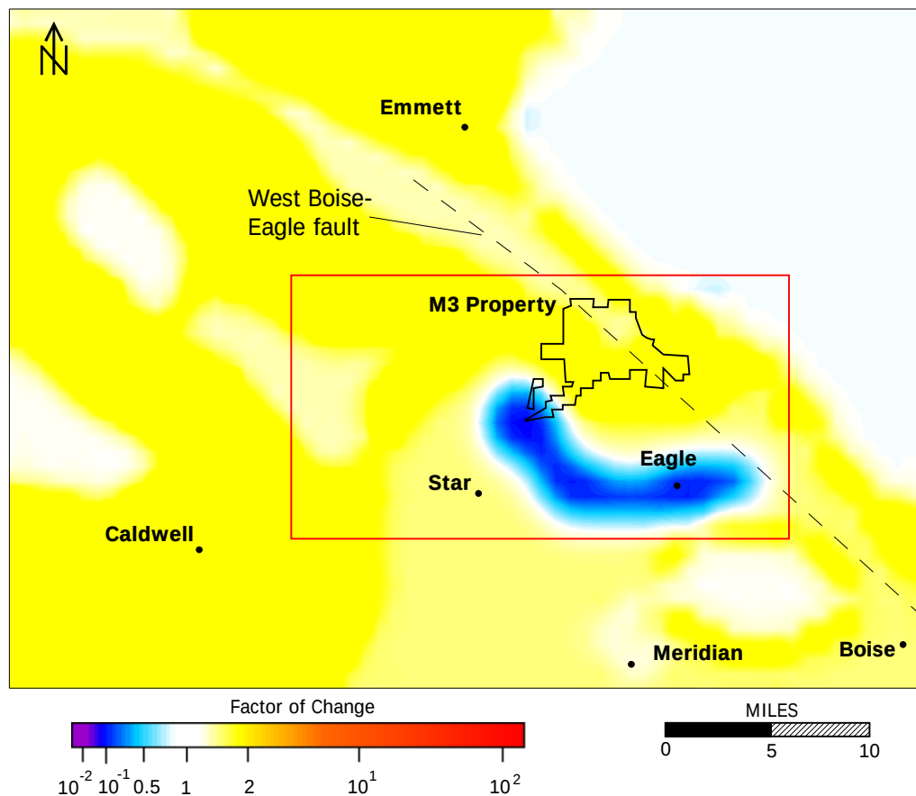
Figure 42. Spatial distribution of changes in K between Model 4 and Model 5. The color scale represents the factor required to multiply the K values for Model 4 to generate the K values in Model 5. Values <1 represent decreases in K . Values >1 represent increases in K .
