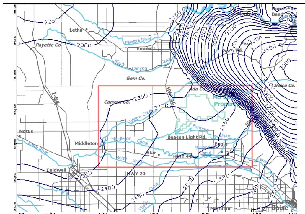
(E) Quasi-Steady-State-Model 5a potentiometric surface for layer 6
