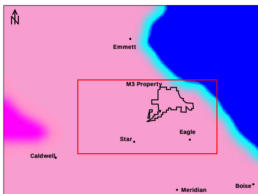
(A) Model 3 Layers 1-3 K (ft/d)
