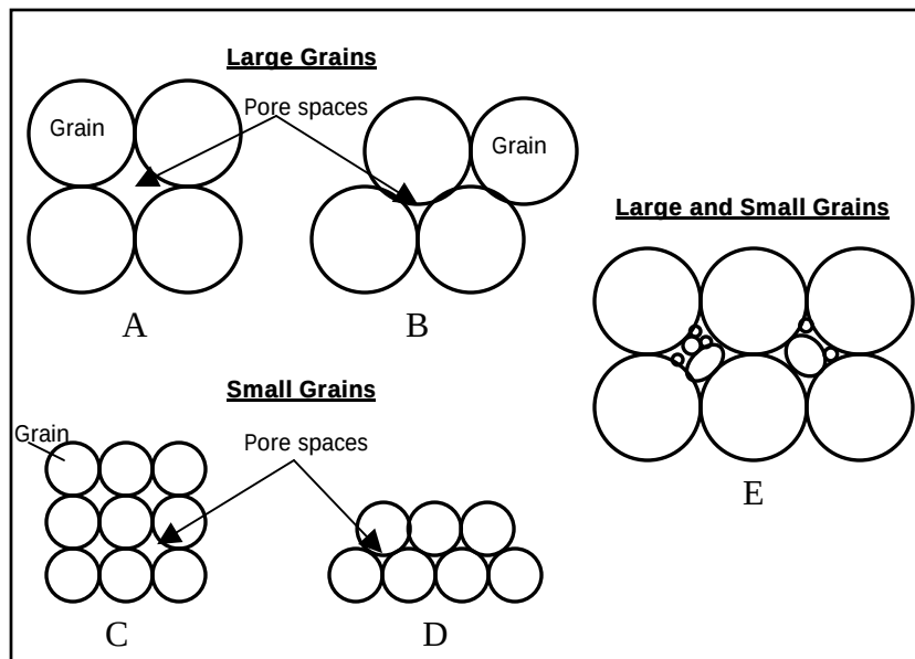
Figure 12. Grain sizes and pore spaces. (A) Large grains in cubic packing with large pore spaces. (B) Large grains in rhombohedral packing with small pore spaces relative to the grains in (A). (C) Small grains in cubic packing with large pore spaces. (D) Small grains in rhombohedral packing with small pore spaces relative to (C). (E) Large grains in cubic packing with smaller grains filling in the pore spaces.
