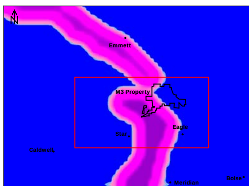
(C) Model 1 Layer 7 K (ft/d)
