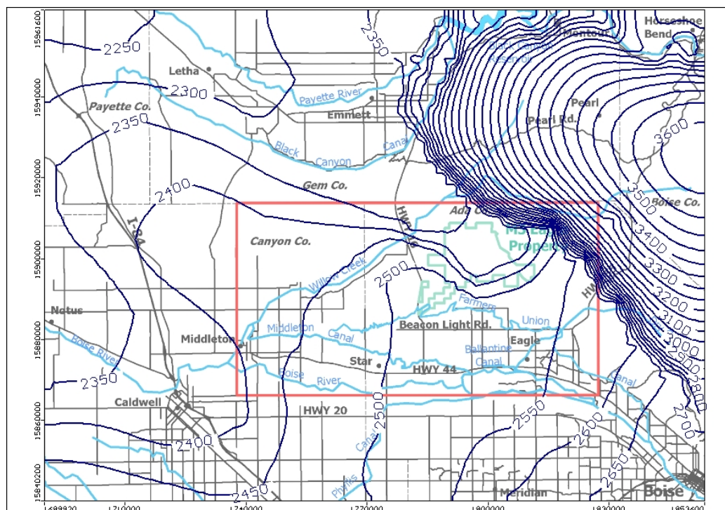
(A) Quasi-Steady-State-Model 1 potentiometric surface for layer 5
