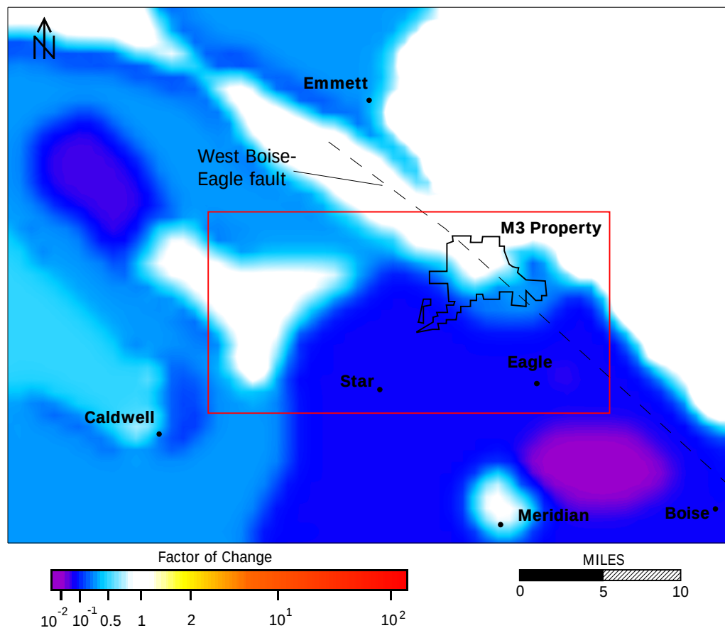
Figure 36. Spatial distribution of changes in K between Model 2 and Model 3. The color scale represents the factor required to multiply the K values for Model 2 to generate the K values in Model 3. Values <1 represent decreases in K . Values >1 represent increases in K .
