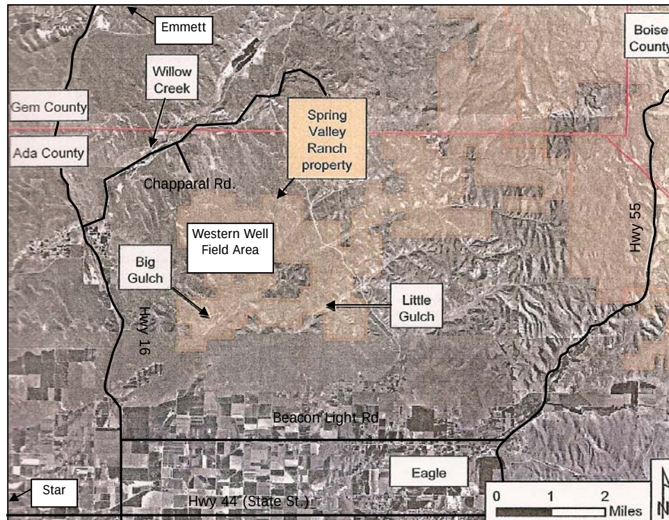
Figure 5. Study area of the SPF investigation for SunCor. Adapted from Figure 1 of SPF Water Engineering, LLC (2004).
