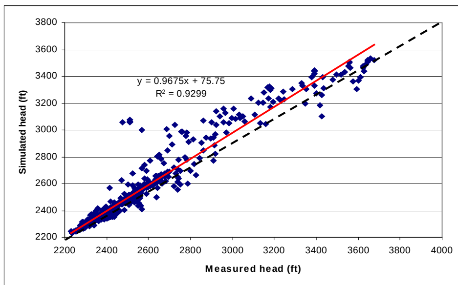
(F) Quasi-Steady-State Model 5b
