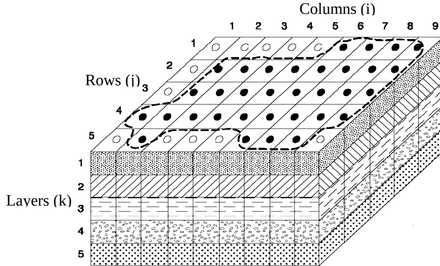
Figure 18. Example three-dimensional finite difference grid used in MODFLOW (Adapted from McDonald and Harbaugh, 1988).
