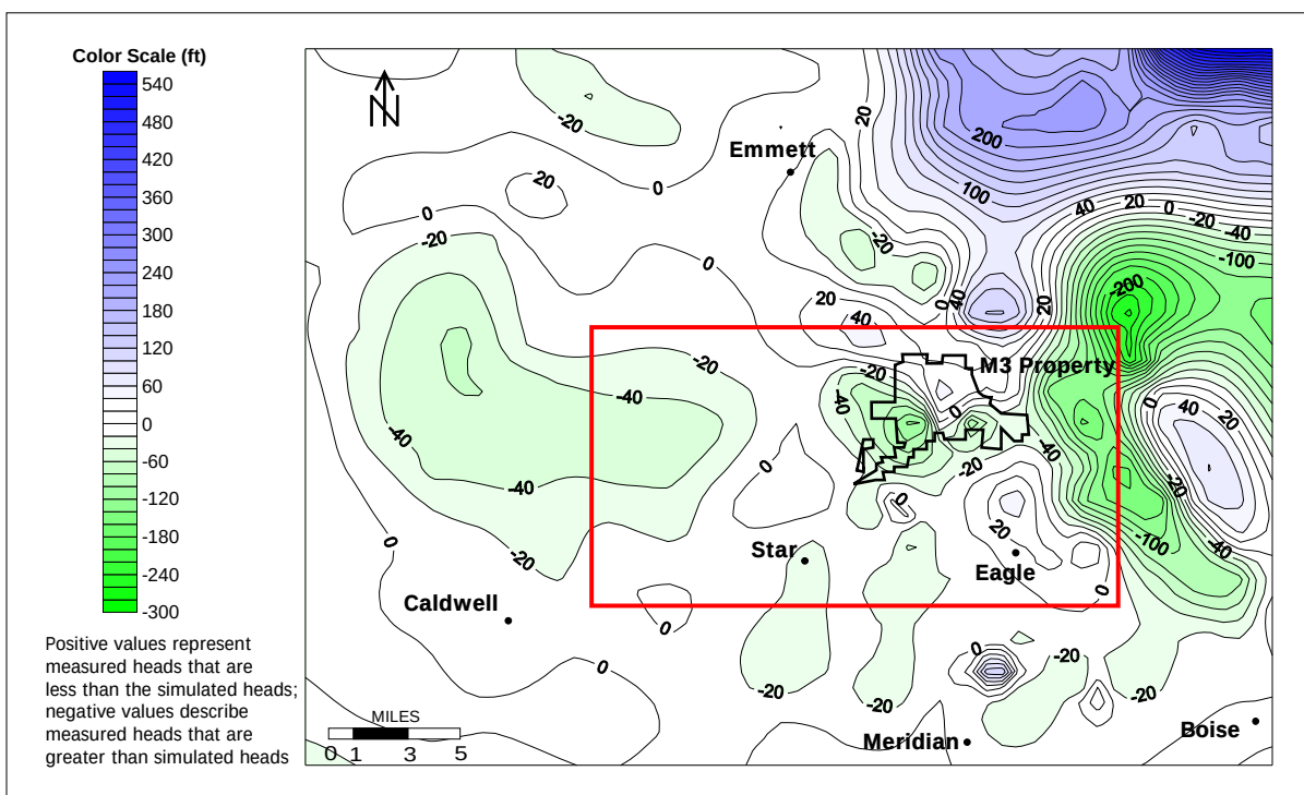
(I) Residuals detailing the difference between simulated and measured head values for Quasi-Steady-State Model 6.
