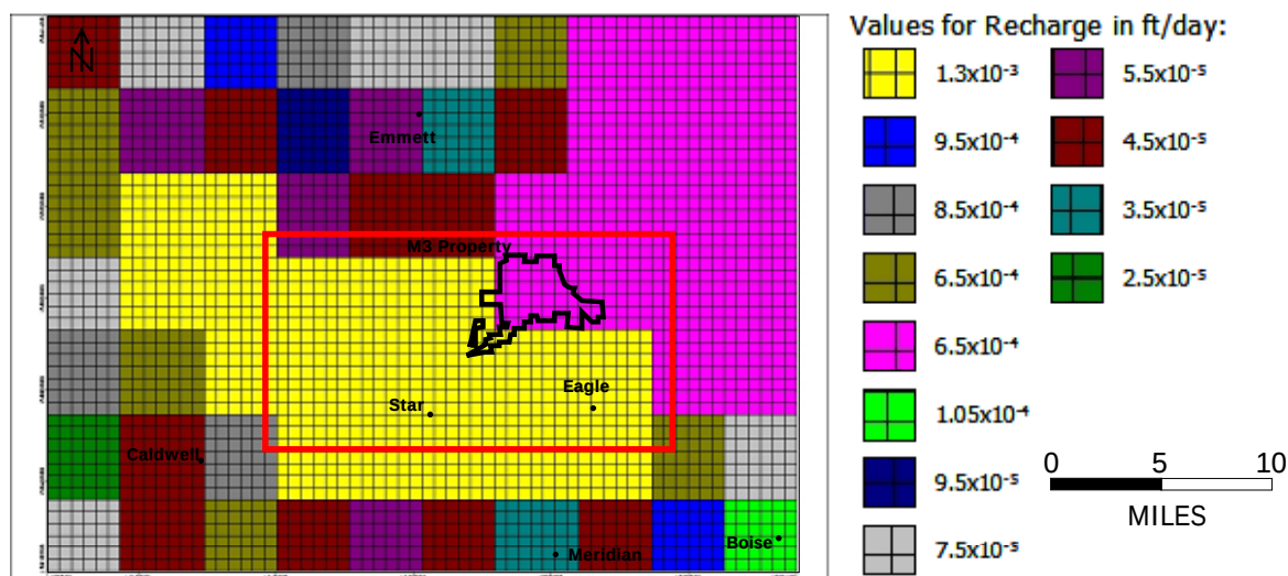
Figure 30. Recharge within the model domain. Each color represents a different rate of recharge. The zone with greatest rate of recharge is the yellow zone ( 1.3 \times 10^{-3} ft/d), and the zone with lowest rate of recharge is the dark green zone ( 2.5 \times 10^{-5} ft/d).
