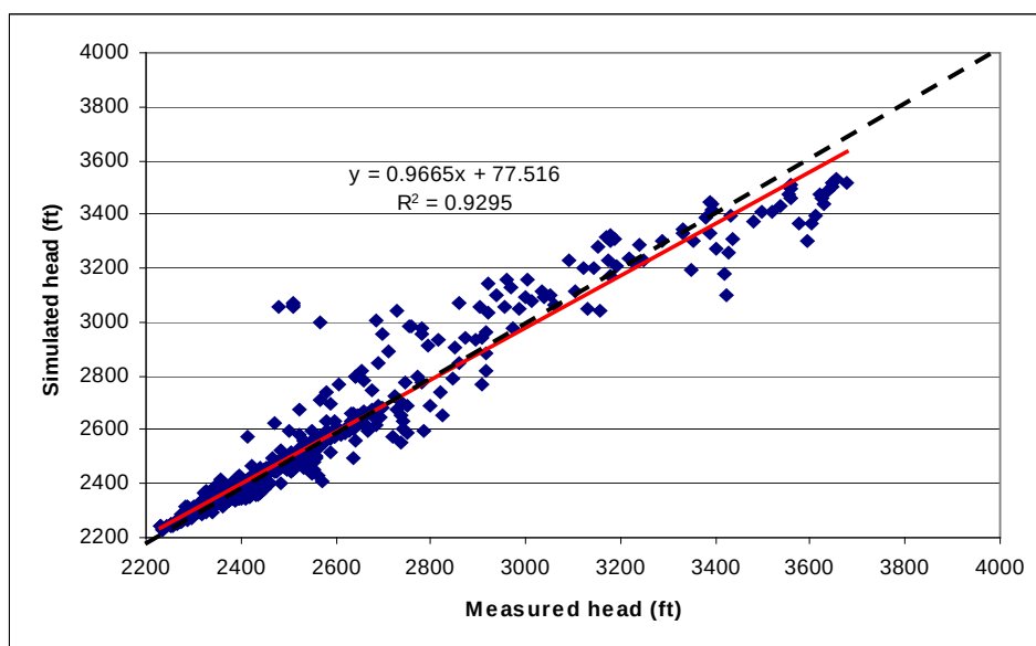
(G) Quasi-Steady-State Model 5c
