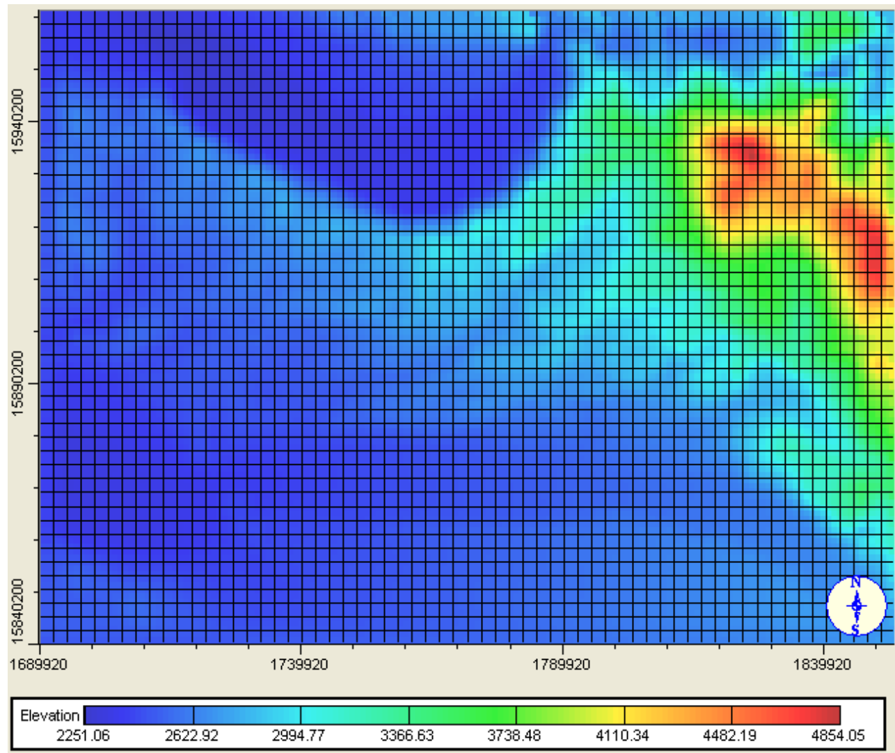
Figure 20. Distribution of elevation within the model domain. Each cell is assigned a value of elevation. The highest elevations (dark red) exist on the eastern side of the model domain in the Boise foothills while the lowest elevations (dark blue) exist in the Payette River valley.
