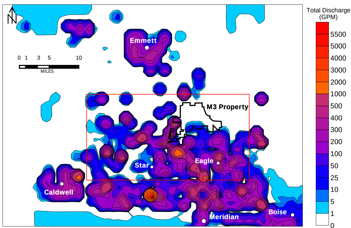
Figure 15. Map of groundwater withdrawal rates from wells within the model domain.
