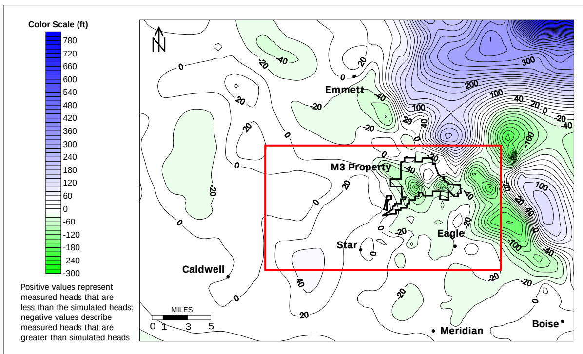
(A) Residuals detailing the difference between simulated and measured head values for Quasi-Steady-State Model 1.
