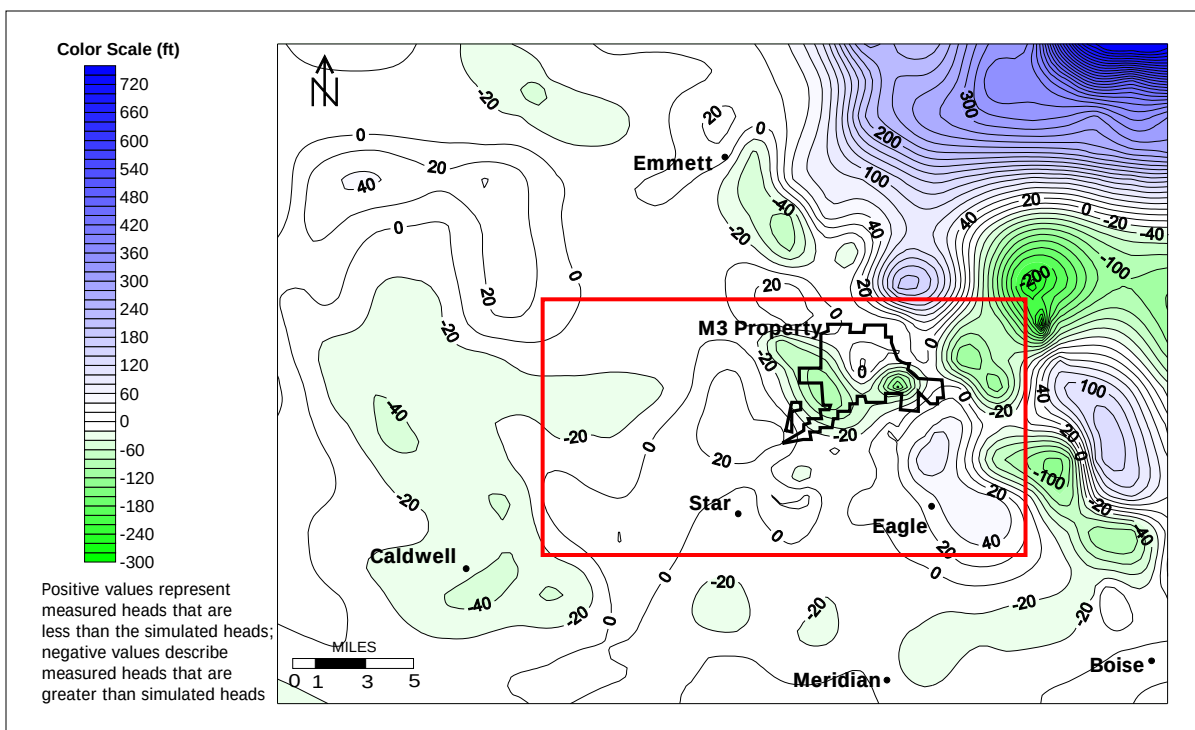
(C) Residuals detailing the difference between simulated and measured head values for Quasi-Steady-State Model 3.
