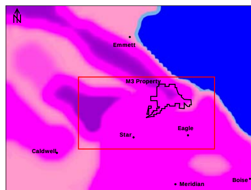
(B) Model 1 Layers 4-6 K (ft/d)
