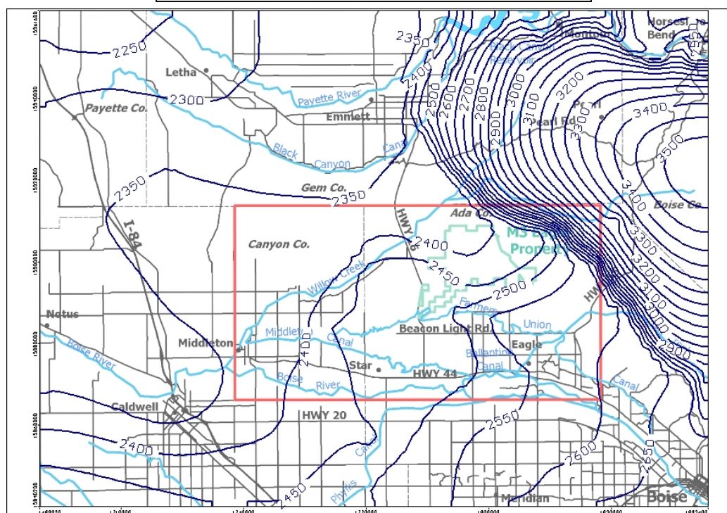
(F) Quasi-Steady-State-Model 5b potentiometric surface for layer 6
