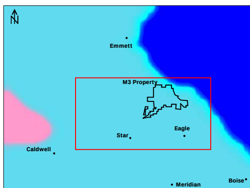
(A) Models 5a-d & 6 Layers 1-3 K (ft/d)
