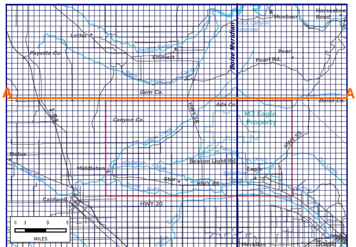
Figure 19. Model grid over the model domain as seen in Visual MODFLOW™ Pro 4.2. The grid is oriented north and south, and is aligned with the Boise Meridian and Beacon Light Road. The grid consists of 62 columns and 46 rows for a total of 2,852 cells per layer. A-A' shows the location of the cross-section presented in Figure 21.
