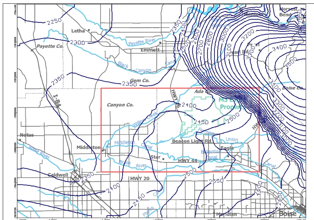
(G) Quasi-Steady-State-Model 5c potentiometric surface for layer 6
