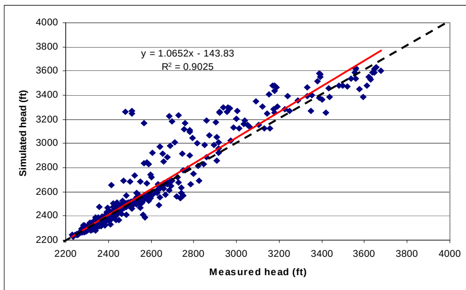
(A) Quasi-Steady-State Model 1
