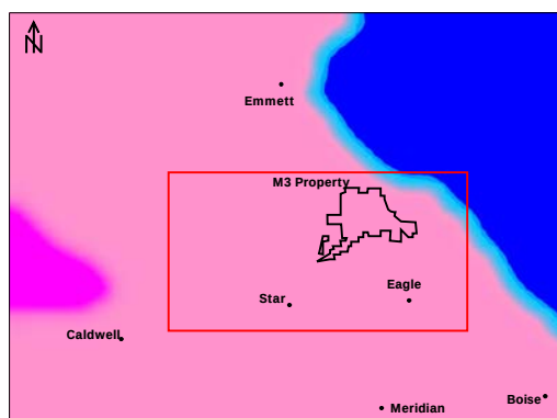
(A) Model 1 Layers 1-3 K (ft/d)
