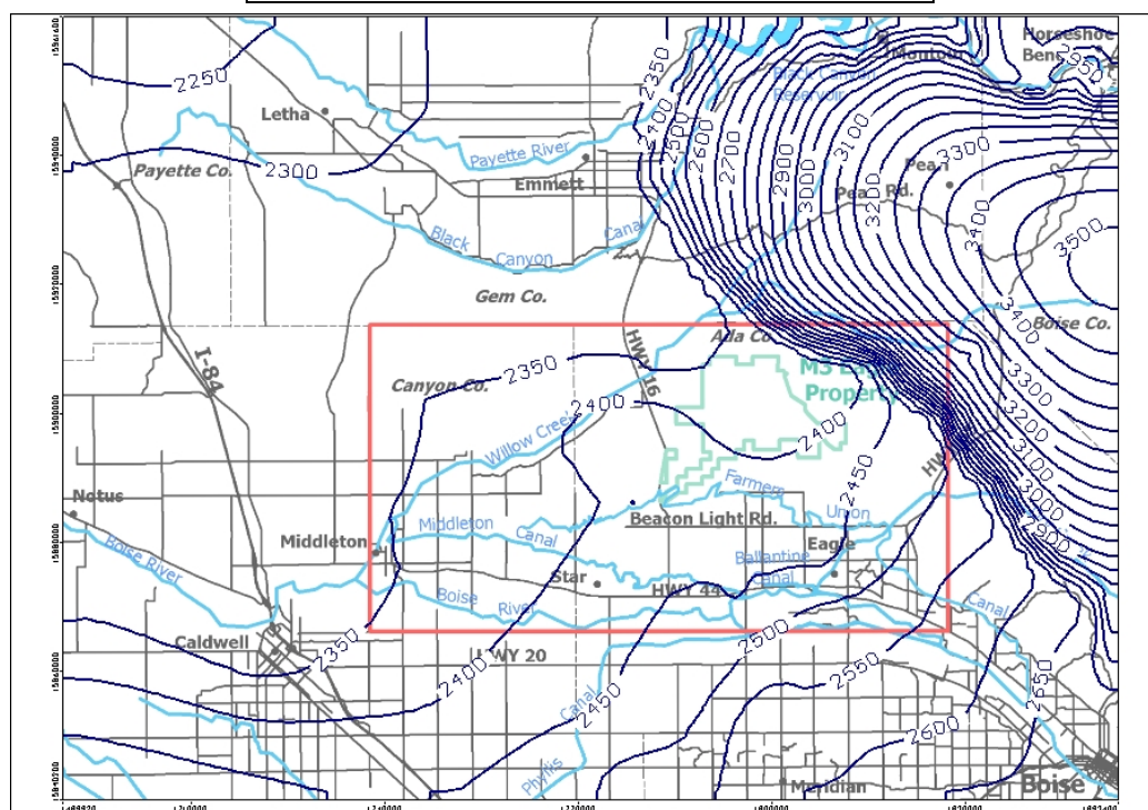
(H) Quasi-Steady-State-Model 5d potentiometric surface for layer 6
