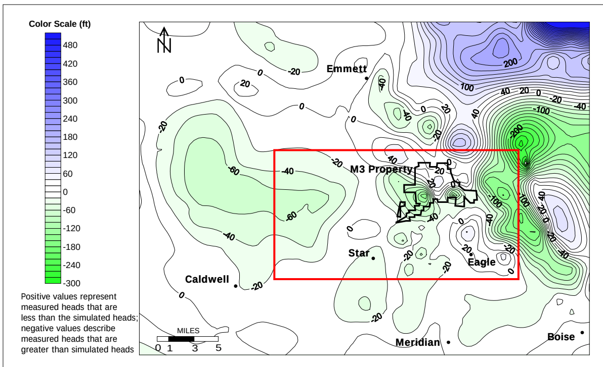
(F) Residuals detailing the difference between simulated and measured head values for Quasi-Steady-State Model 5b.
