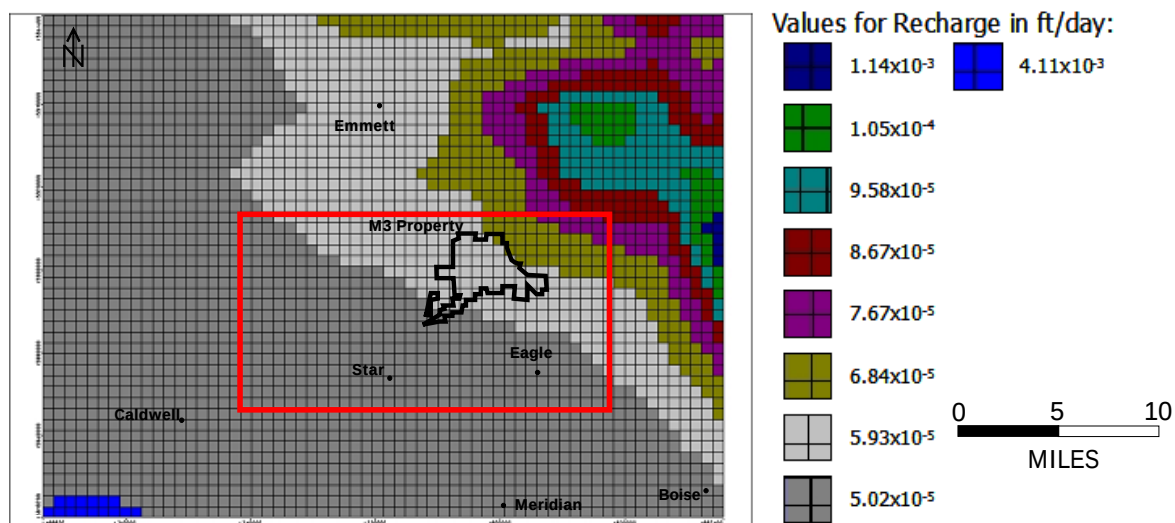
Figure 43. Distribution of Recharge within the model domain for the Steady-State Model.
