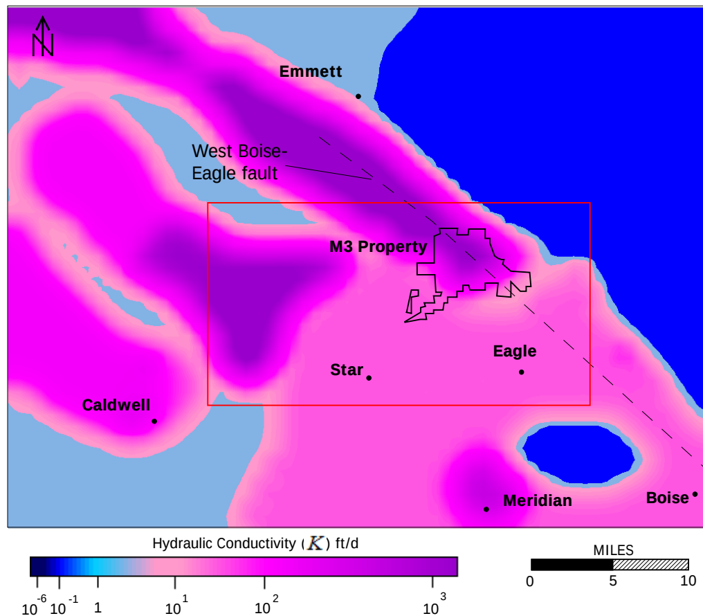
Figure 39. Hydraulic conductivity ( K ) distribution for the Pierce Gulch Sand aquifer system (Layers 6 and 7) in Model 4.
