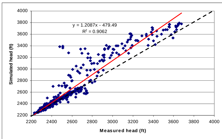
(B) Quasi-Steady-State Model 2
