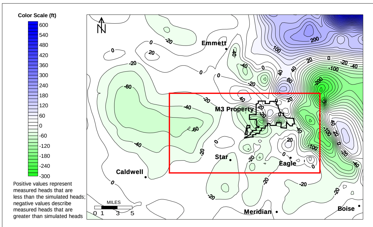
(G) Residuals detailing the difference between simulated and measured head values for Quasi-Steady-State Model 5c.
