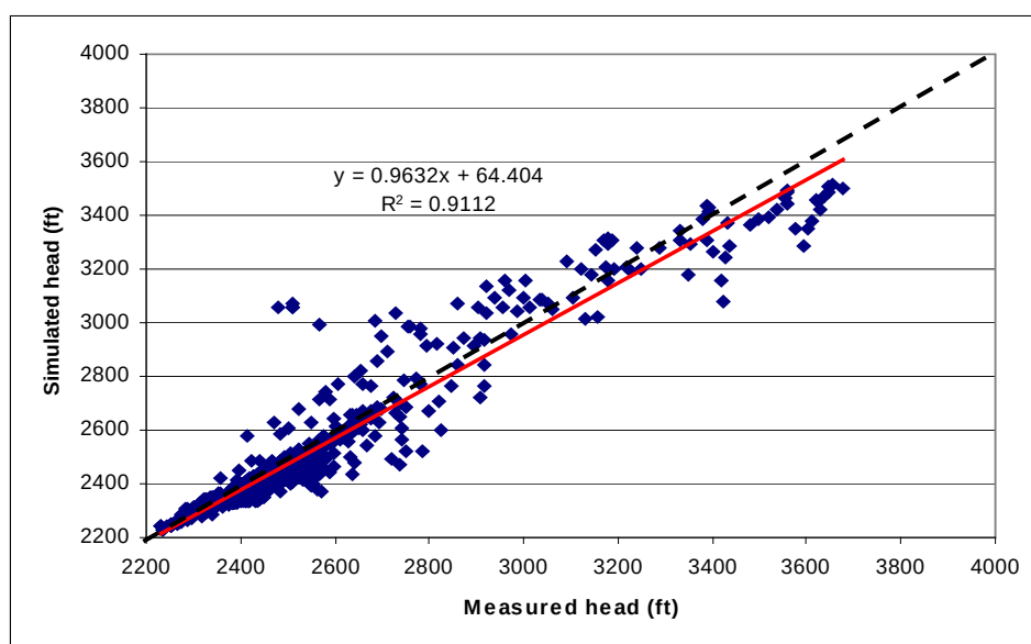
(H) Quasi-Steady-State Model 5d
