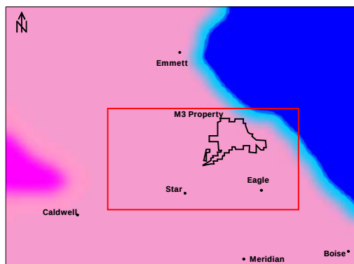
(A) Model 4 Layers 1-3 K (ft/d)
