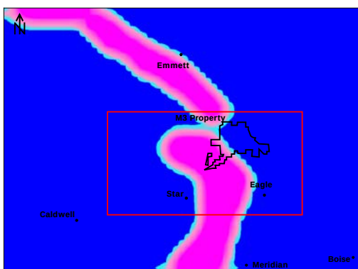
(E) Models 5a-d & 6 Layer 8 K (ft/d)
