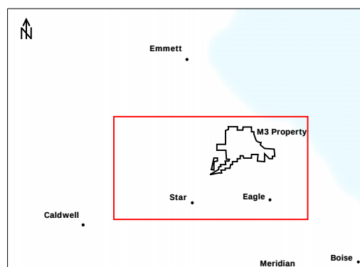
(B) Layers 4 (Model 3) and Layer 5 (Model 4)
