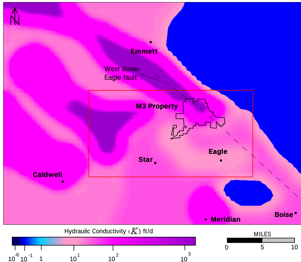
Figure 41. Hydraulic conductivity ( K ) distribution for the Pierce Gulch Sand aquifer system (Layers 6 and 7) in Model 5 and Model 6.
