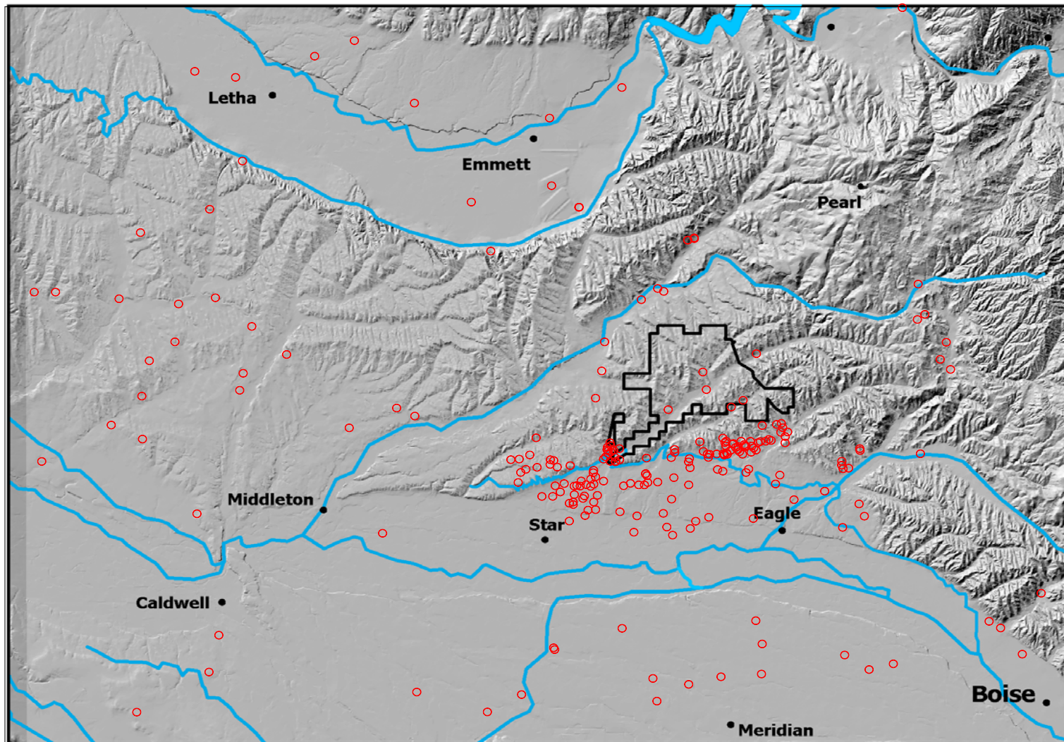
Figure 16. Map of wells used in the model. Most of the wells are in the vicinity of the M3 Eagle Development property, Star, and Eagle. Some of the measurements were acquired from the IDWR Online Ground Water Level Database.
