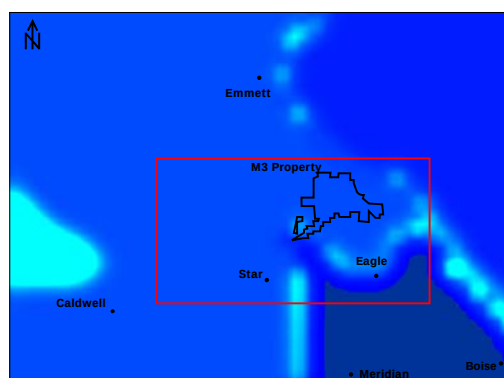
(B) Models 5a-d & 6 Layer 4 K (ft/d)
