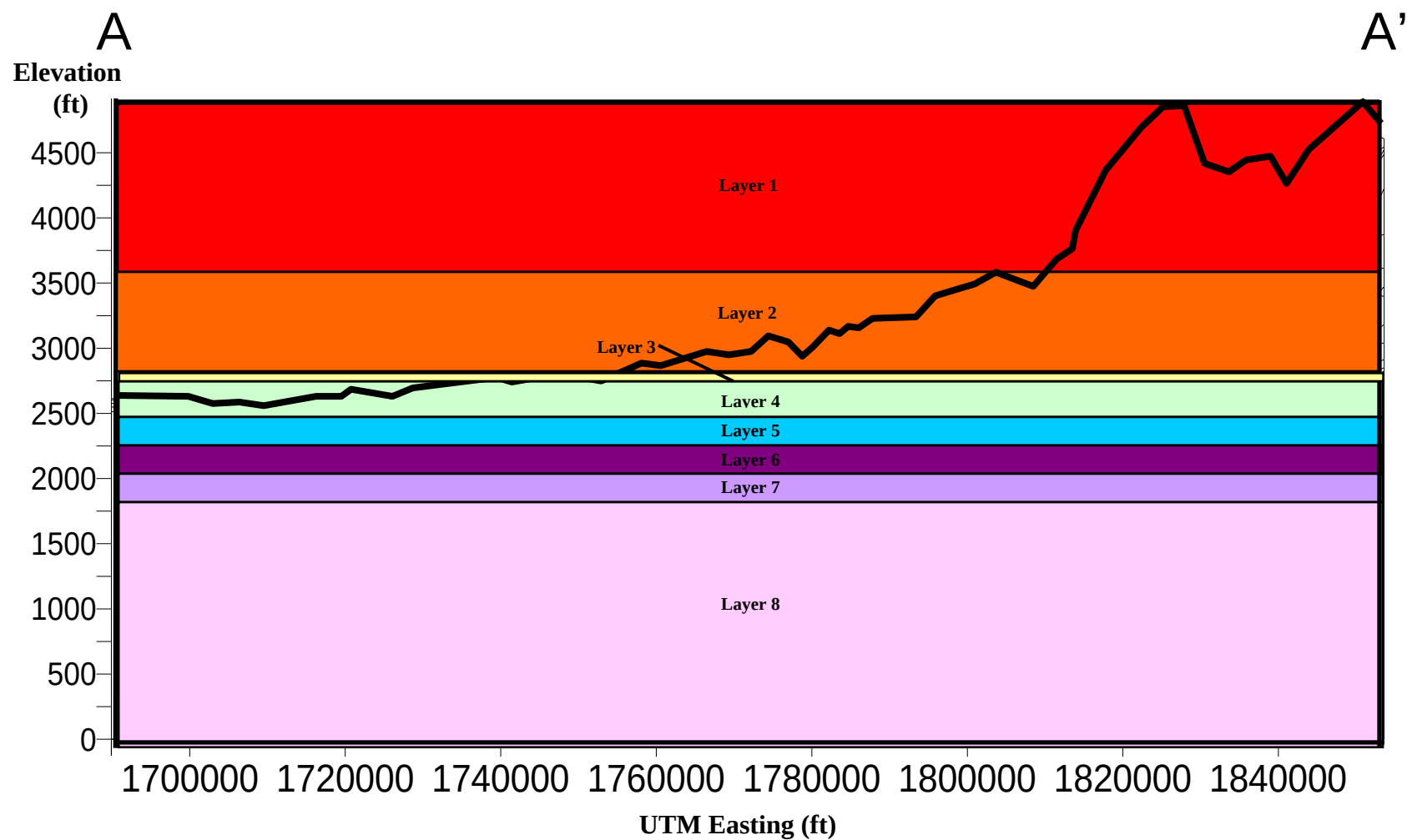
Figure 21. A-A' cross-section across the model domain. The cross-section is taken approximately one mile north of the M3 Eagle Development property as shown in Figure 19. The model contains eight layers. Layer(s) 5 and/or 6 represent the Pierce Gulch Sand aquifer system depending on location within the model domain.
