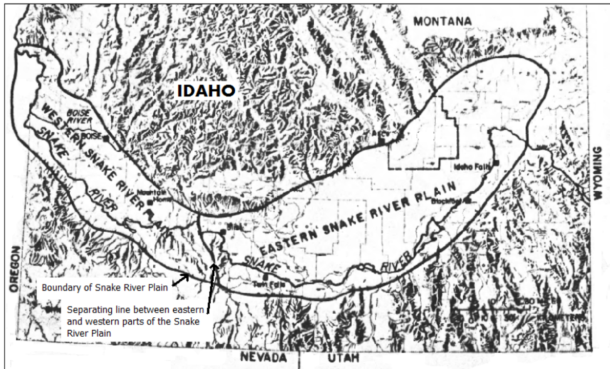
Figure 2. Study area of Lindholm (1981) showing the Western and Eastern Snake River plains. Adapted from Figure 1 of Lindholm (1981).
