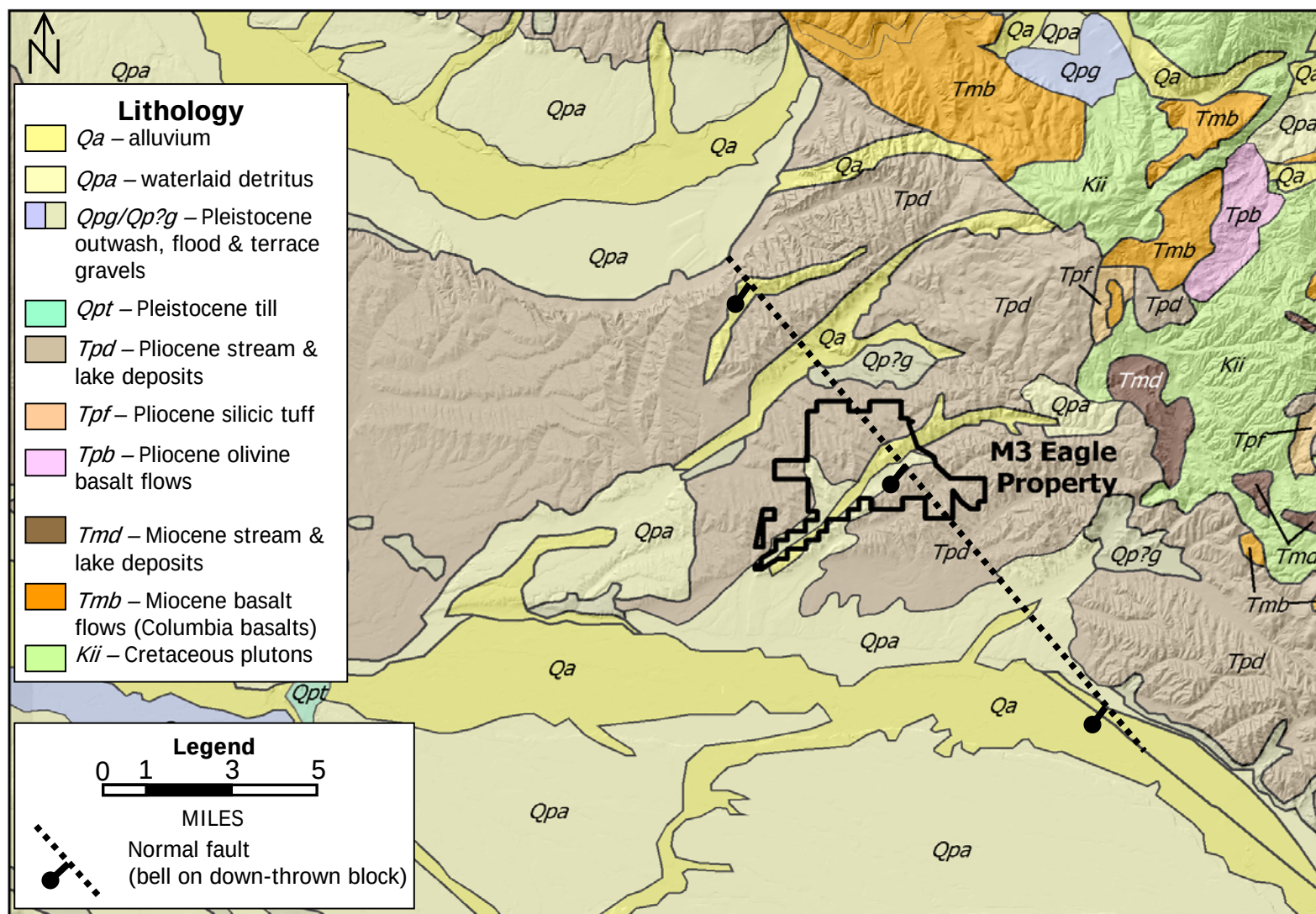
Figure 9. Surface geology of the M3 Eagle Big Gulch Model domain. The black dashed line represents the West Boise-Eagle fault. The source for the geological map is the U.S. Geological Survey (2006). The fault was inferred from topographic maps provided by HLI and maps in Wood and Clemens (2002).
