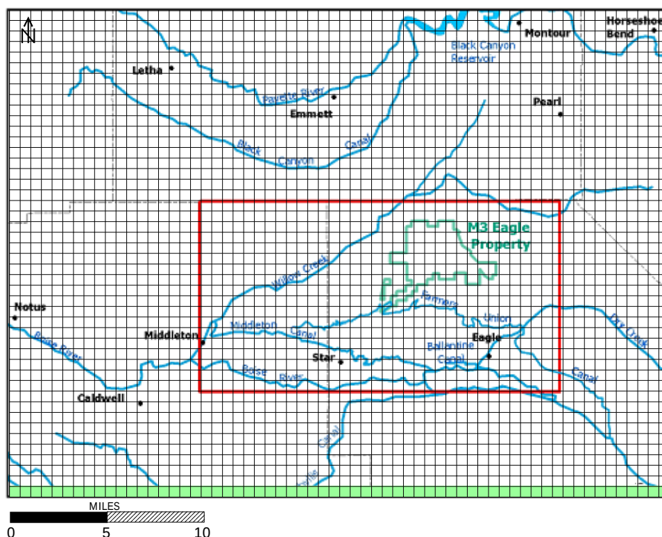
Figure 24. General-head boundaries in the quasi-steady-state model grid Layer 7. The green cells represent the general heads.
