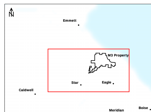
(C) Layers 5-6 (Model 3) and Layers 6-7 (Model 4)
