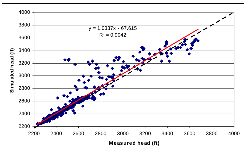
(C) Quasi-Steady-State Model 3
