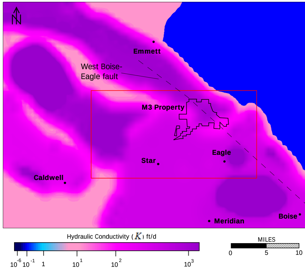
Figure 33. Hydraulic conductivity ( K ) distribution for the Pierce Gulch Sand aquifer system (Layers 5 and 6) in Model 2.
