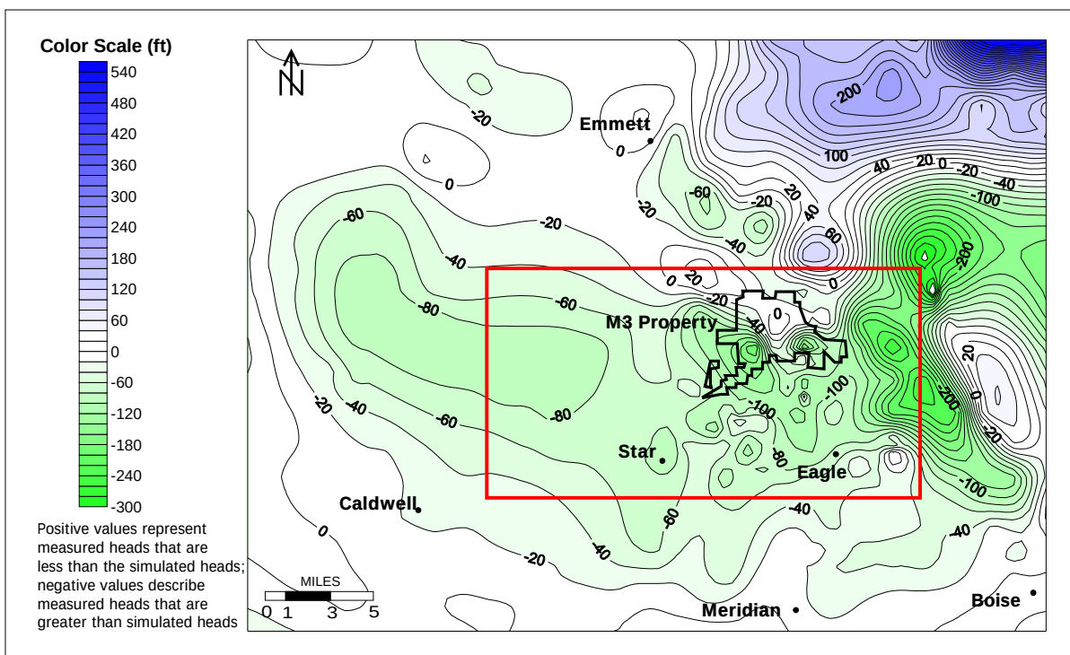
(E) Residuals detailing the difference between simulated and measured head values for Quasi-Steady-State Model 5a.
