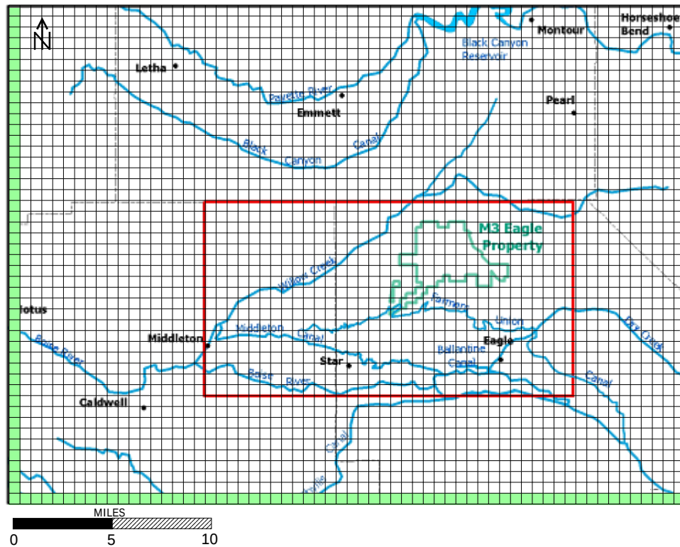
Figure 22. General-head cells in the steady-state model grid Layer 8. The general-heads cells are shown in green.
