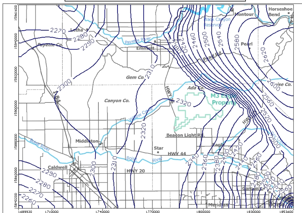
(J) Steady-State Model potentiometric surface for layer 6
