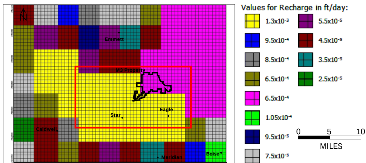
Figure 37. Recharge rates for Models 3, 4, and 6. Each color represents a different rate of recharge. The zone with greatest rate of recharge is the yellow zone ( 1.3 \times 10^{-3} ft/d), and the zone with lowest rate of recharge is the dark green zone ( 2.5 \times 10^{-5} ft/d).
