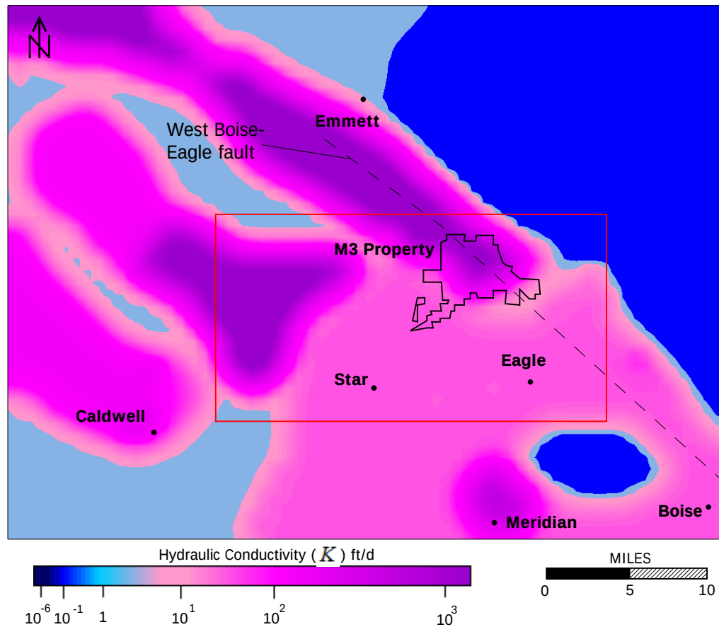
Figure 35. Hydraulic conductivity ( K ) distribution for the Pierce Gulch Sand aquifer system (Layers 5 and 6) in Model 3.
