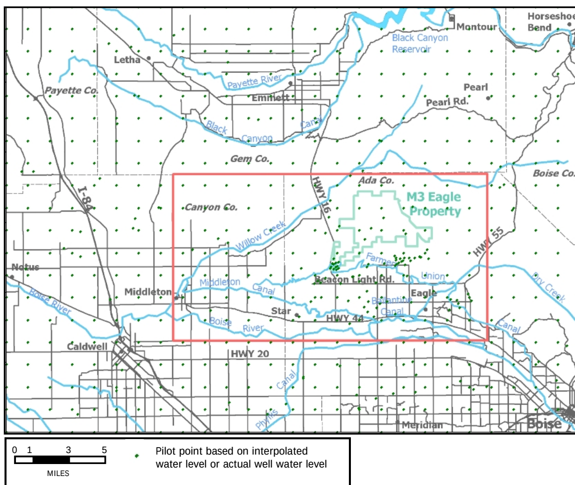
Figure 29. Map of the water level calibration points used in the model. The green points are pilot points that identify real wells plus points selected off the water level contour map (Figure 17); water levels for 540 points were interpolated from the water level contour map, and water levels for 137 points were measured in real wells.
