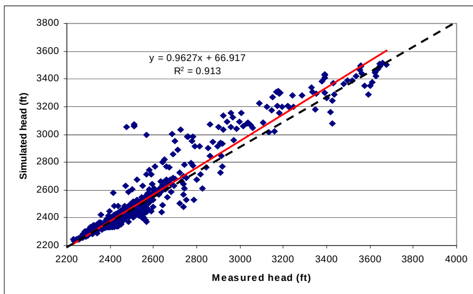
(E) Quasi-Steady-State Model 5a
