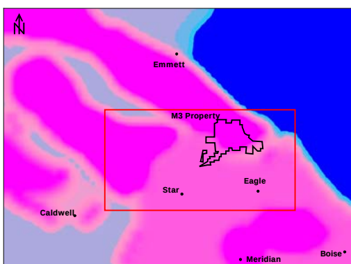
(C) Model 4 Layer 5 K (ft/d)
