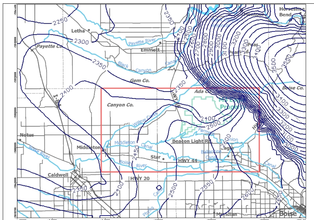
(C) Quasi-Steady-State-Model 3 potentiometric surface for layer 5
