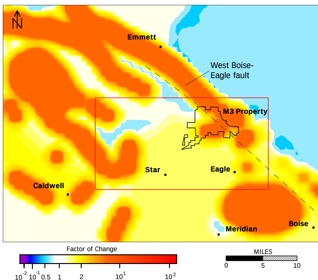
Figure 34. Spatial distribution of changes in K between Model 1 and Model 2. The color scale represents the factor required to multiply the K values for Model 1 to generate the K values in Model 2. Values <1 represent decreases in K . Values >1 represent increases in K .
