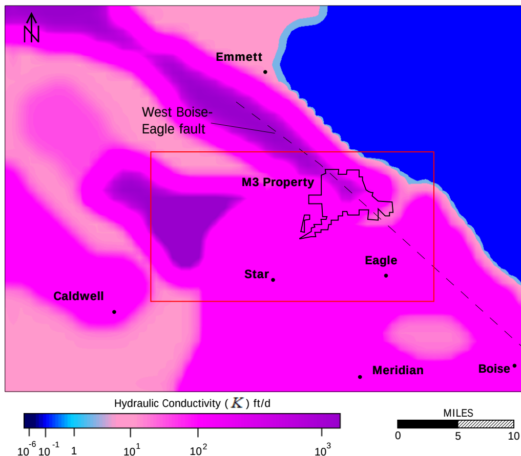
Figure 31. Hydraulic conductivity ( K ) distribution for the Pierce Gulch Sand aquifer system (Layer 5) in Model 1.
