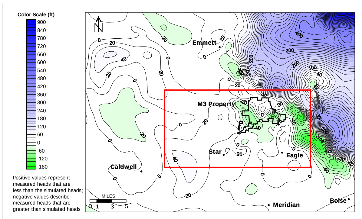
(B) Residuals detailing the difference between simulated and measured head values for Quasi-Steady-State Model 2.
