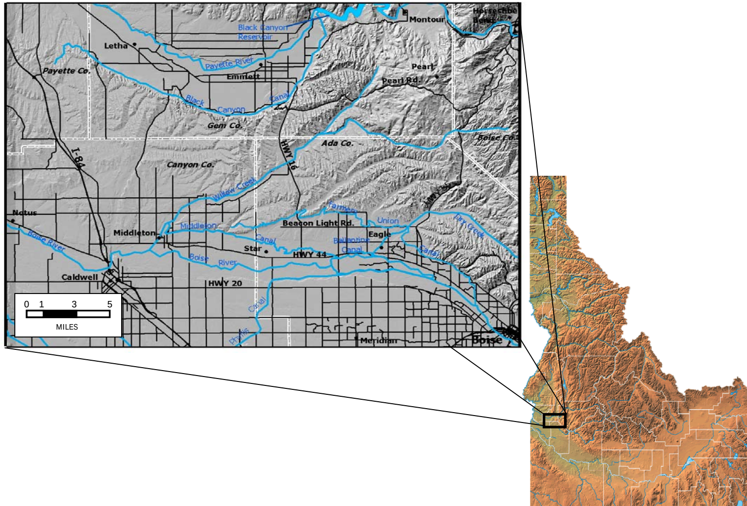
Figure 1. Map detailing the location of the M3 Eagle Big Gulch Model domain. The model domain is located in southwestern Idaho along the northern fringe of the Western Snake River Plain. Adapted from the U.S. Geological Survey (2006) and Geology.com.
