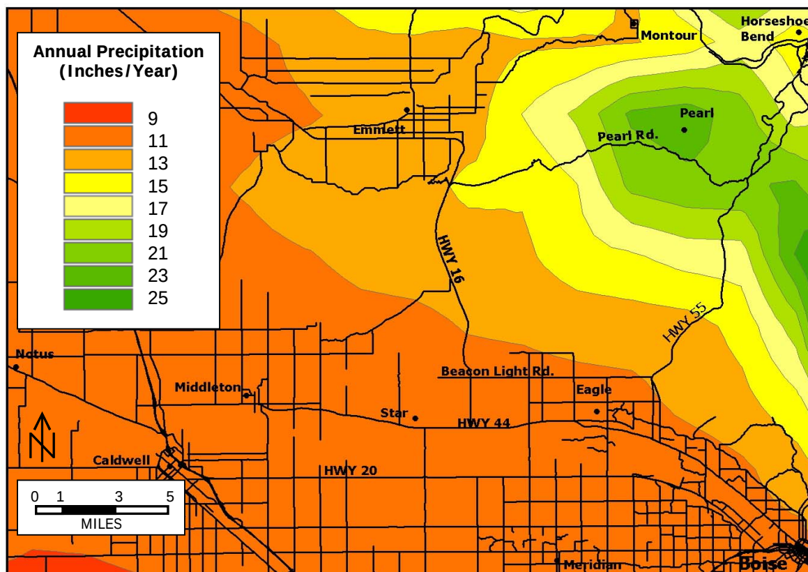
Figure 13. Map of the precipitation distribution within the model domain. More precipitation occurs over the Idaho batholith in the Boise Foothills and less occurs in the Boise River valley. Adapted from Idaho Department of Water Resources GIS data ( http://www.idwr.state.id.us/ftp/gisdata/spatial ).
