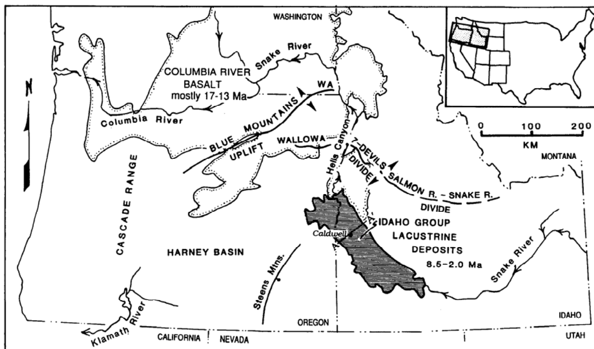
Figure 8. Map detailing the location of the Idaho Group lacustrine deposits in the Western Snake River Plain. Adapted from Figure 2 of Wood (1994).
