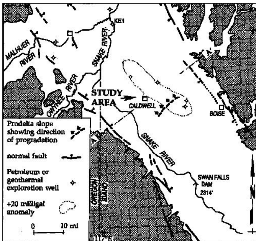
Figure 10. Map of the position and progradation direction of the lacustrine delta system near Caldwell. The dashed line shows the position and progradation direction of the lacustrine delta system during the Pliocene interpreted from a study by Wood (1994) and from a previous study by Wood and Anderson (1981). Adapted from Figure 2 of Wood (1994).
