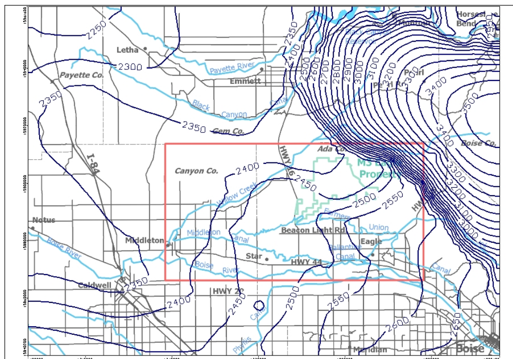
(I) Quasi-Steady-State-Model 6 potentiometric surface for layer 6
