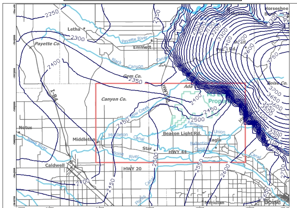
(B) Quasi-Steady-State-Model 2 potentiometric surface for layer 5
