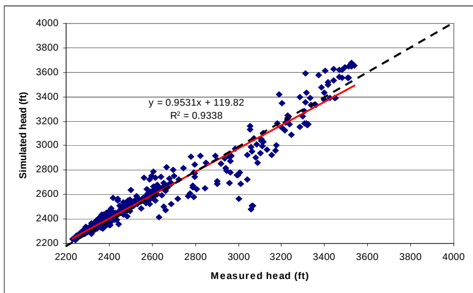
(I) Quasi-Steady-State Model 6
