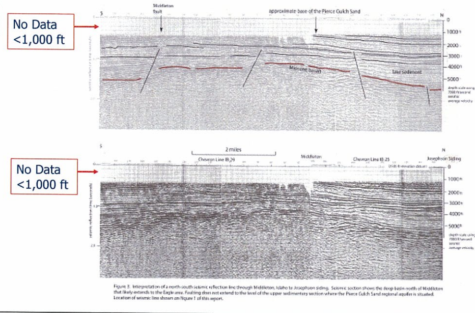
Figure 2. Subsurface Seismic Reflection Profiles (from Wood)
