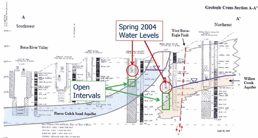
Figure 5. Geologic Cross-Section through the M3 Eagle Site
