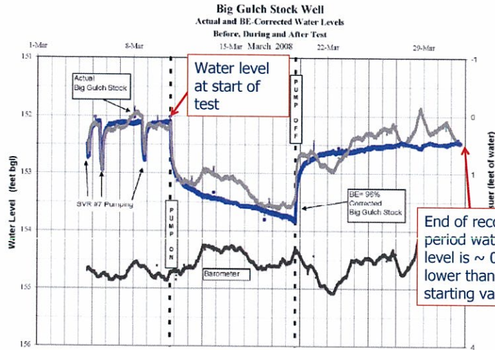
Figure C-3. Actual and BE-Corrected Water Levels for Big Gulch Stock Well
