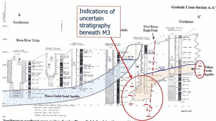
Figure 5. Geologic Cross-Section through the M3 Eagle Site
