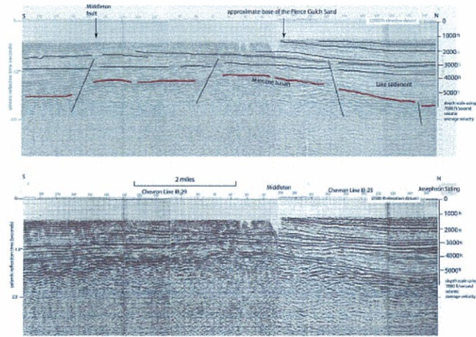
Figure 3. Interpretation of a north-south seismic reflection line through Middleton, Idaho to Josephine siding. Seismic section shows the deep basin north of Middleton that likely extends to the Bagby area. Faulting does not extend to the level of the upper sedimentary section where the Pierce Gulch Sand regional aquifer is situated. Location of seismic line shown on Figure 1 of this report.
