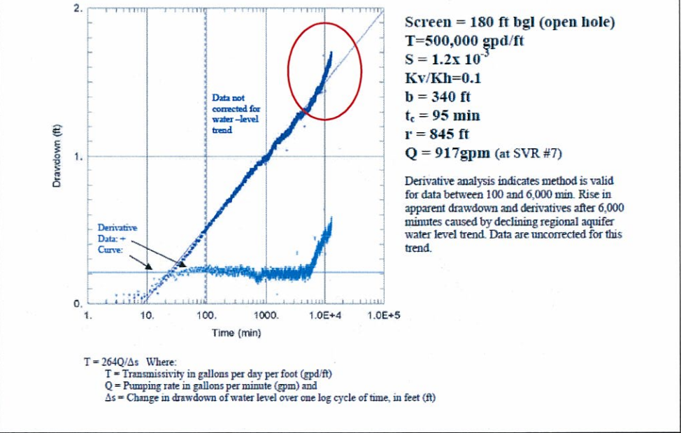
Figure 24 Figure 24. Cooper-Jacob Analysis for the Big Gulch Stock Well
