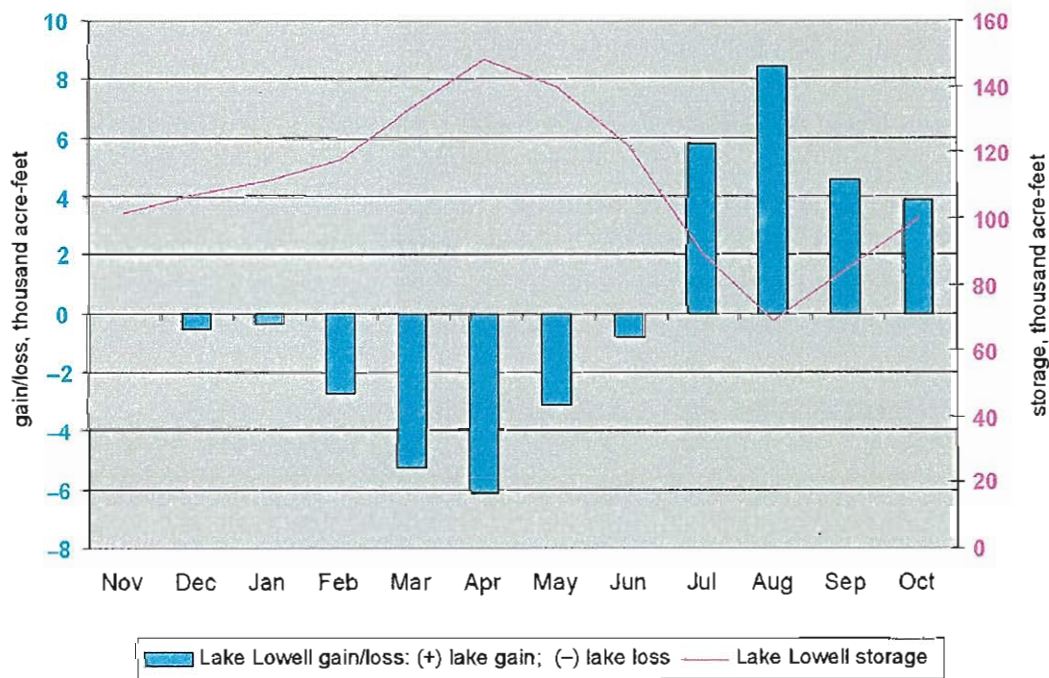
Figure 3-5. Average monthly reservoir level and gain-or-loss from Lake Lowell.
