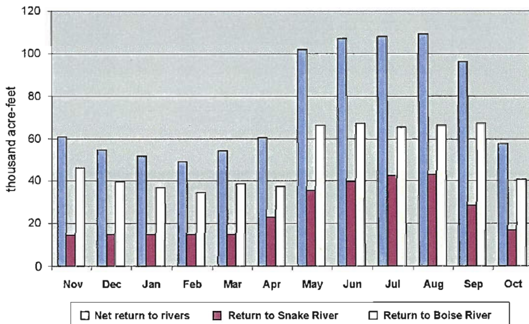
Figure 2-16. Average monthly drain return to Boise River and Snake River.
