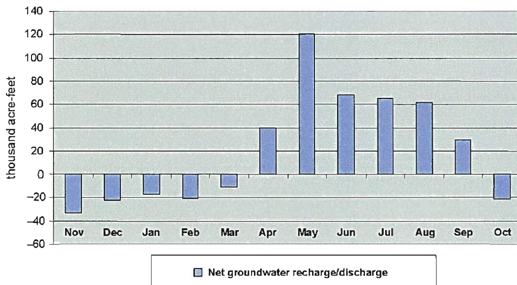
Figure 2-18. Average monthly net groundwater recharge-discharge on irrigated agricultural land.
