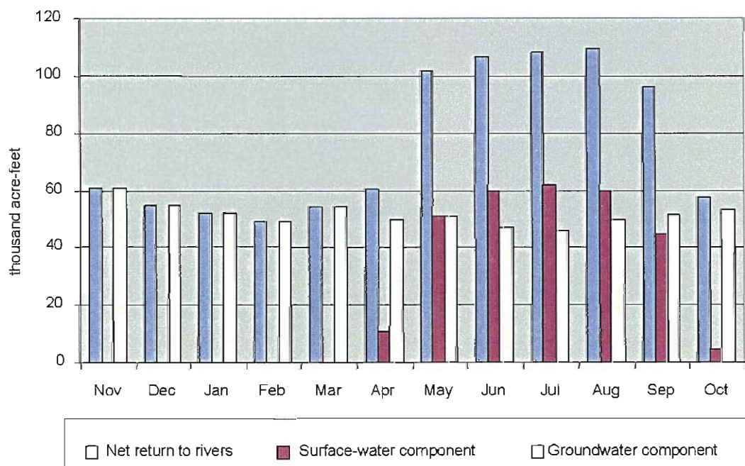
Figure 2-15. Average monthly surface-water and groundwater components of drain return.
