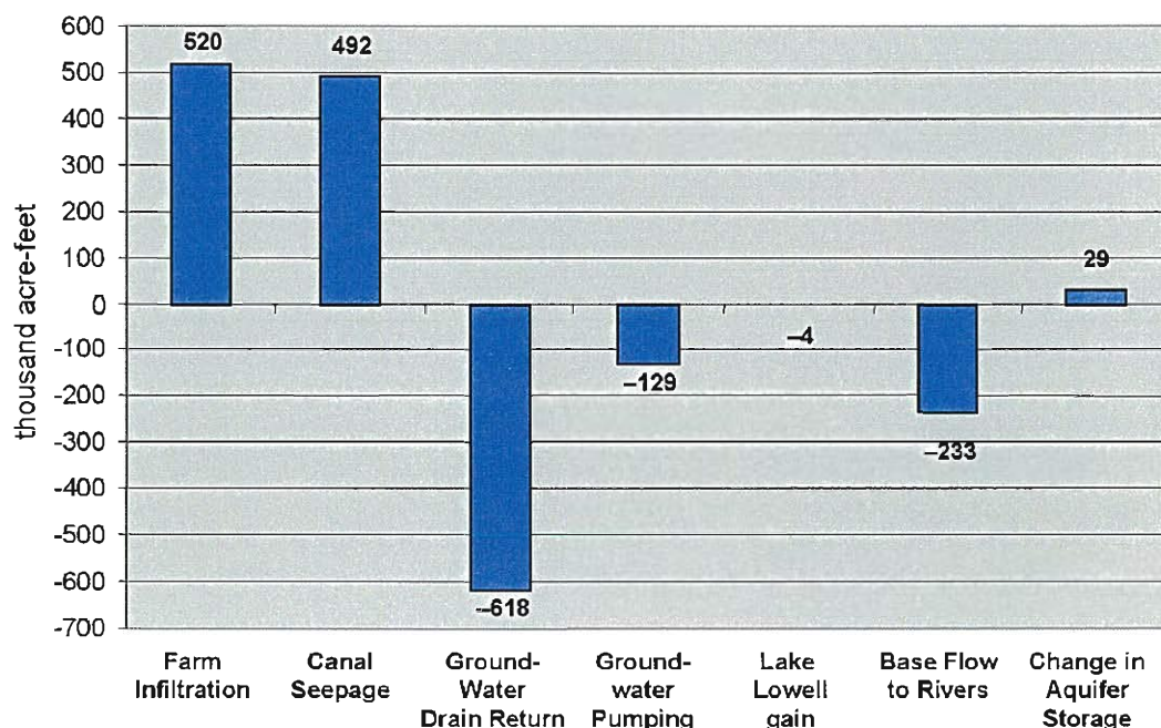
Figure 2-8. Average annual groundwater budget for irrigated agricultural lands.
