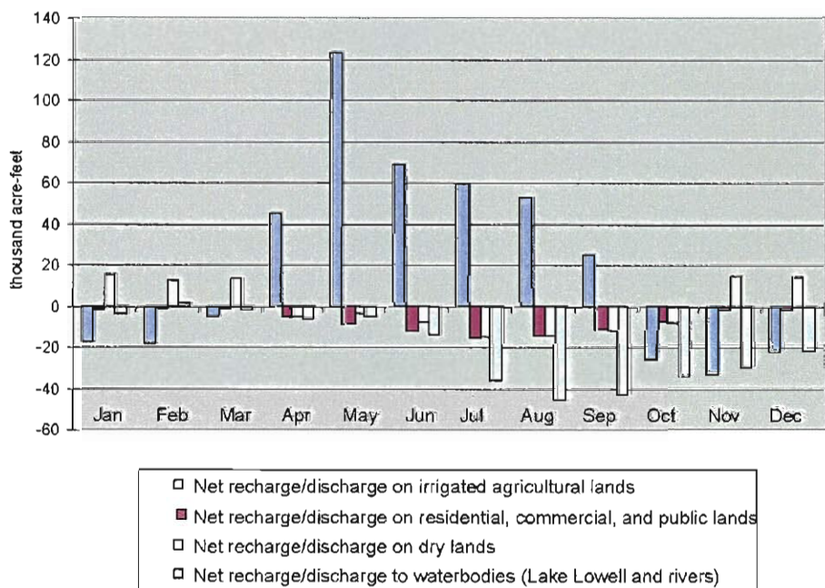
Figure 5–7. Average monthly net groundwater recharge-discharge on lands in all three budget categories.
