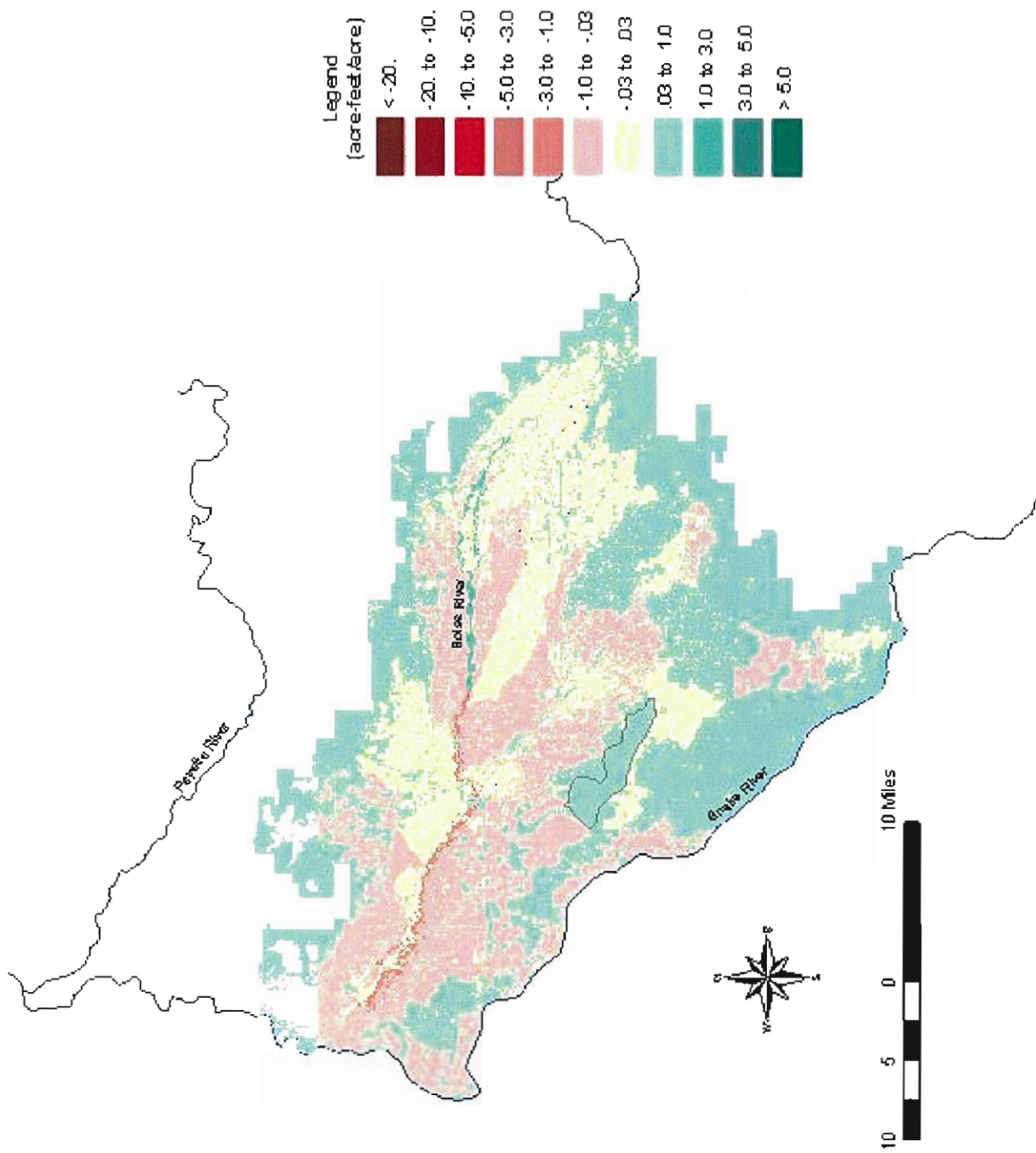
Figure 5-19. January, monthly distribution of groundwater recharge-discharge
