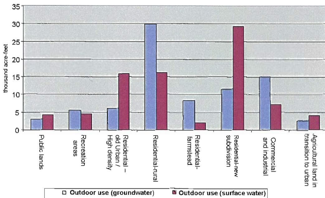
Figure 4–8. Outdoor surface-water and groundwater use by land-class.
