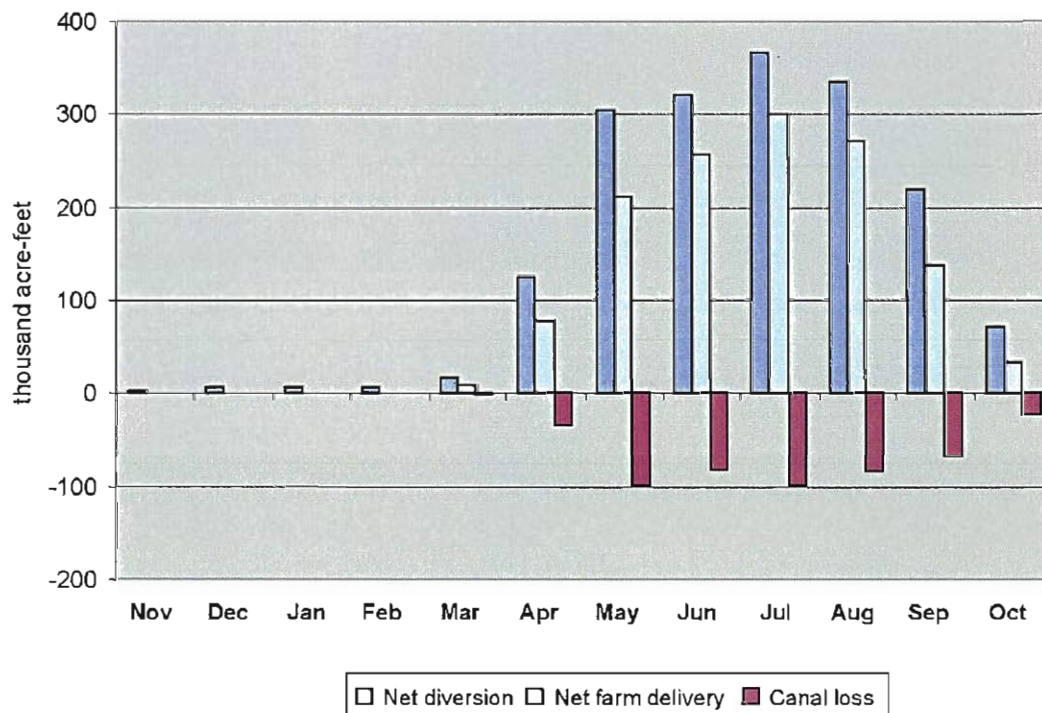
Figure 2-10. Average monthly diversion, farm delivery, and canal loss.
