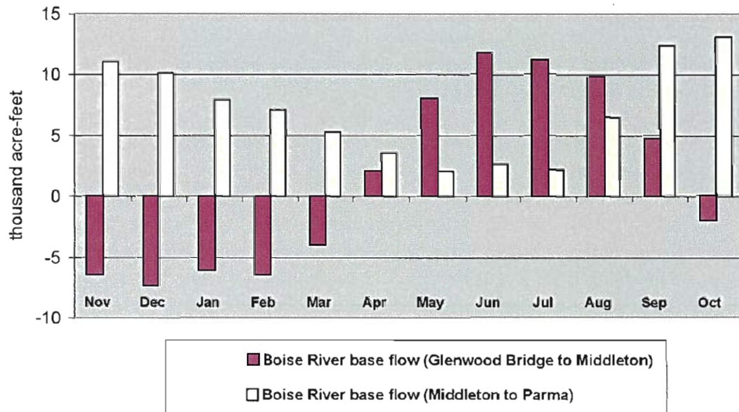
Figure 3–3. Average monthly base flow to the Boise River, Glenwood Bridge to Parma.
