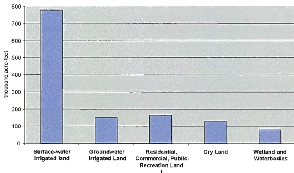
Figure 5–1. Composite distribution of ET and outdoor consumptive use.
