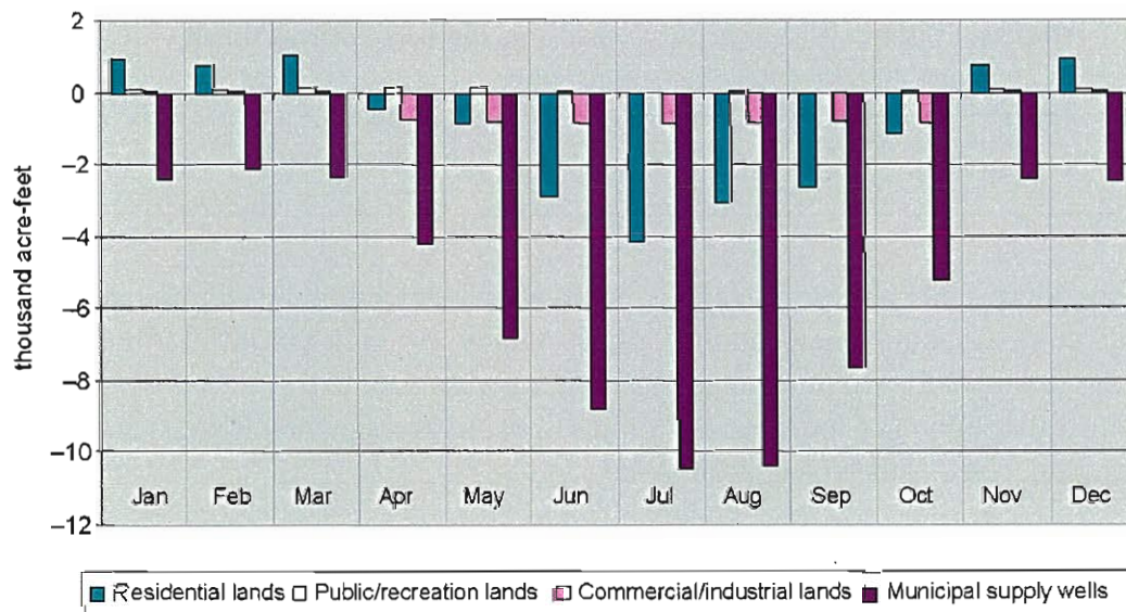
Figure 4–10. Monthly distribution of net groundwater recharge-discharge on all residential, commercial, and public-recreation lands.
