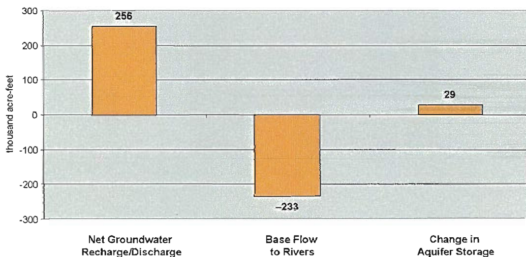
Figure 2-9. Average annual net groundwater recharge-discharge.
