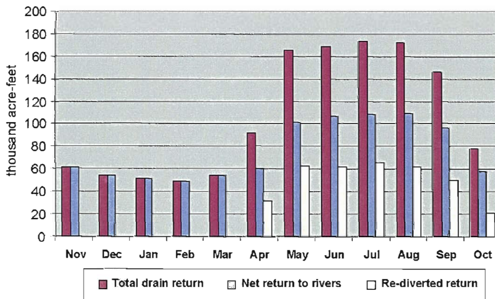
Figure 2-14. Average monthly drain return, net return to rivers, and re-diverted return.
