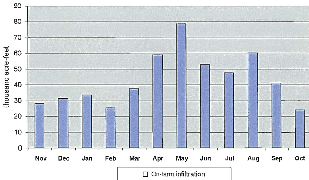
Figure 2-17. Average monthly on-farm infiltration.
