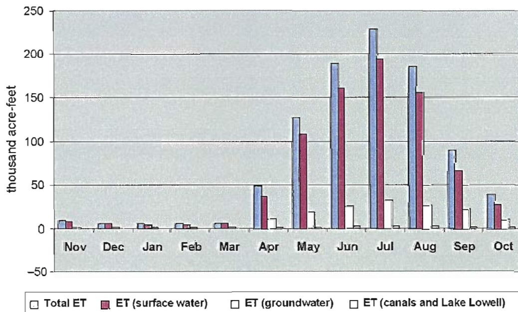
Figure 2-13. Average monthly ET on surface-water and groundwater irrigated lands.
