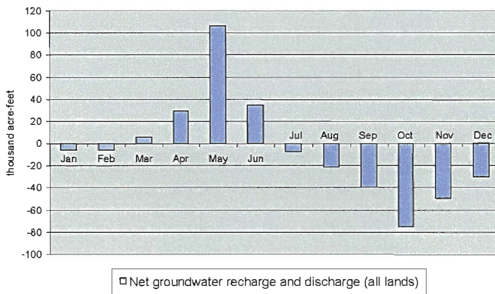
Figure 5–8. Average monthly net groundwater recharge-discharge, all lands.
