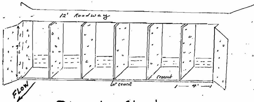
Diversion Structure
