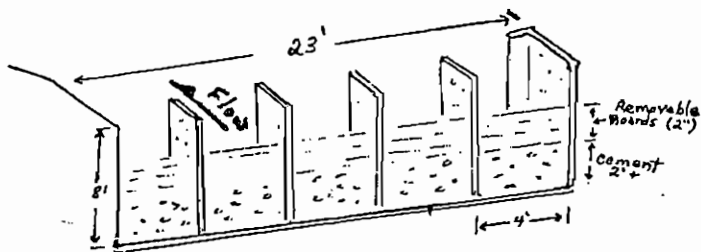
Control Structure.
