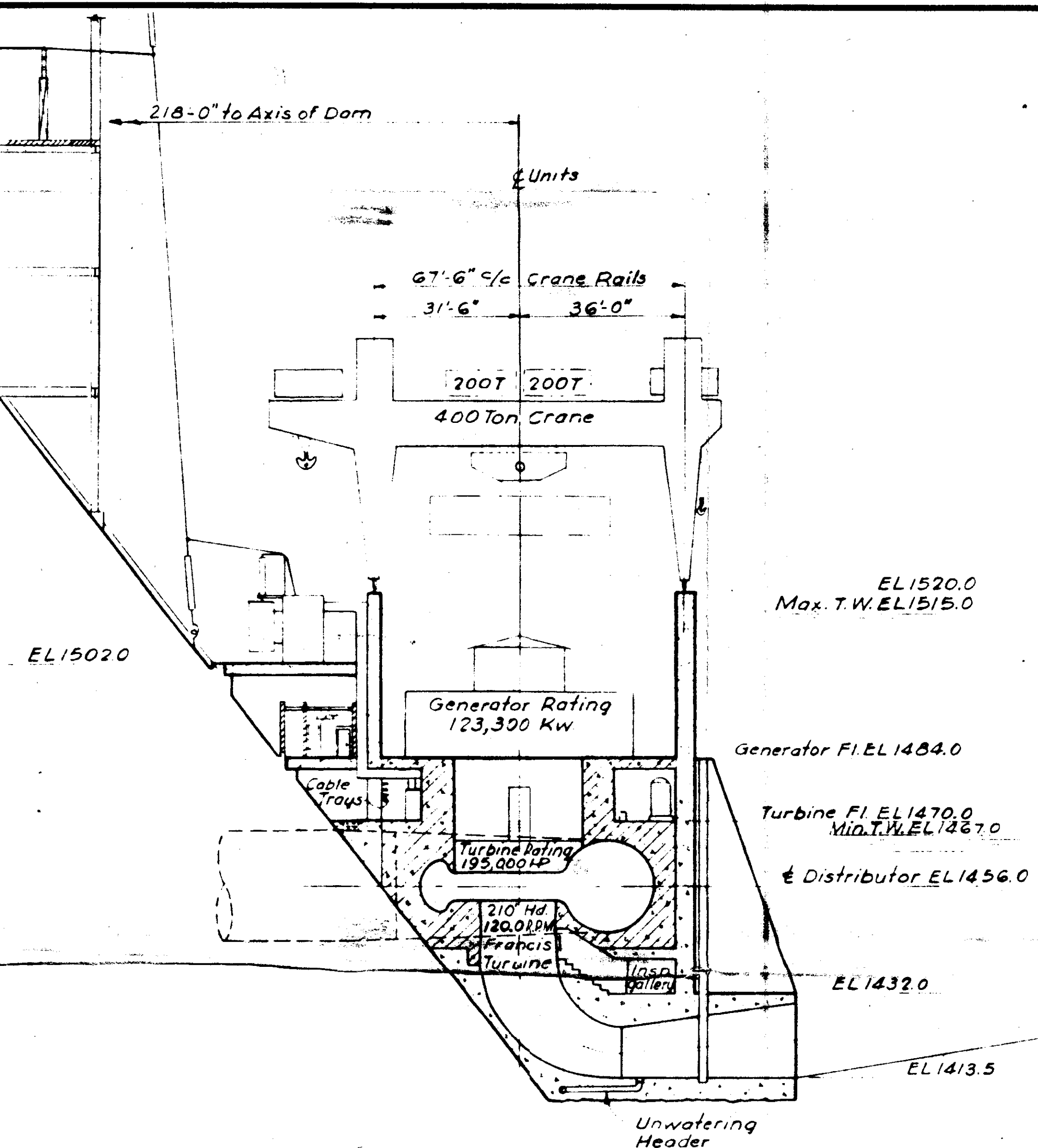
TRANSVERSE SECTION THROUGH E OF UNIT NO. 1 A-A
