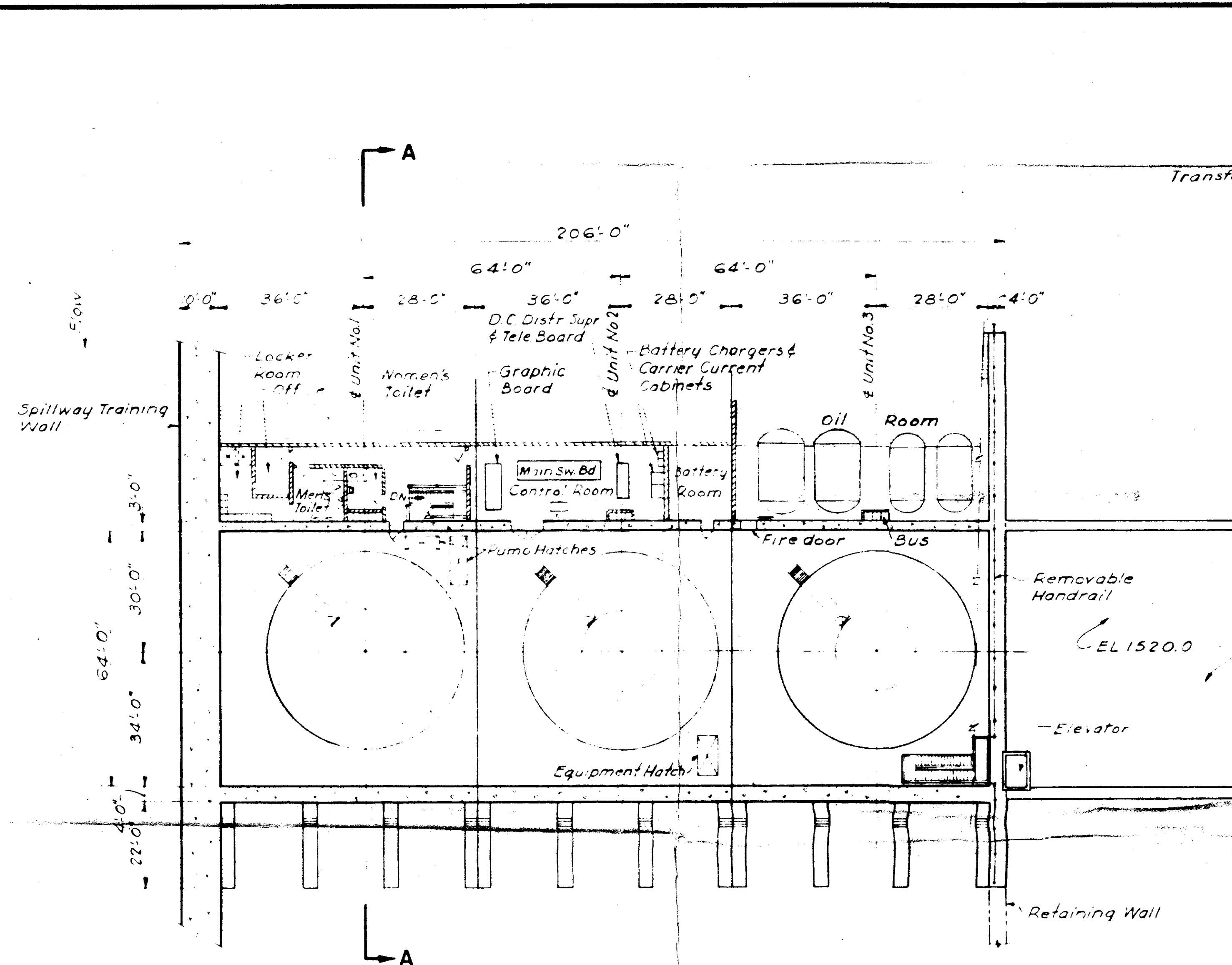
PLAN GENERATOR FLOOR EL1484.0
