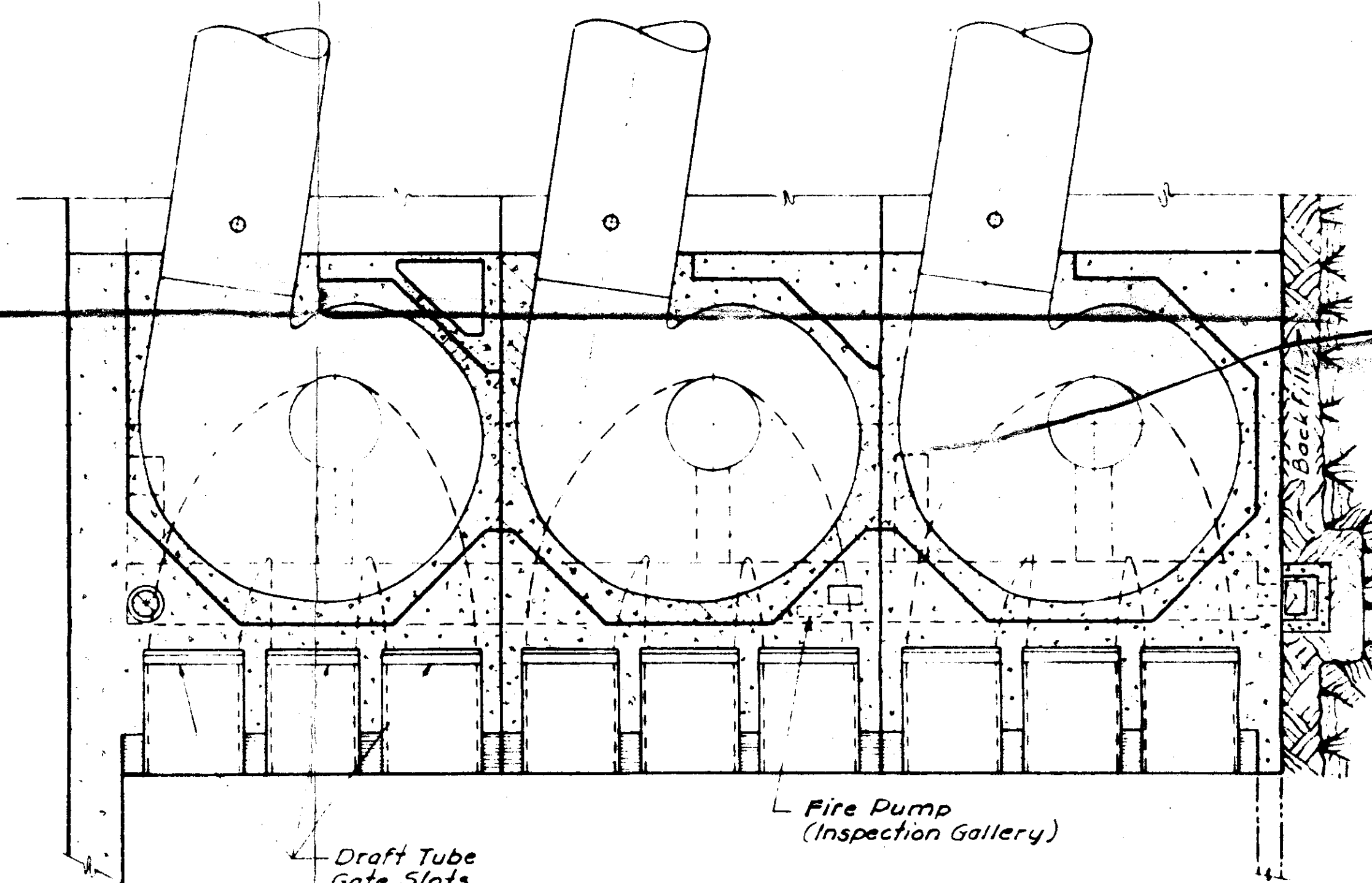
PLAN DISTRIBUTOR EL1456.0
