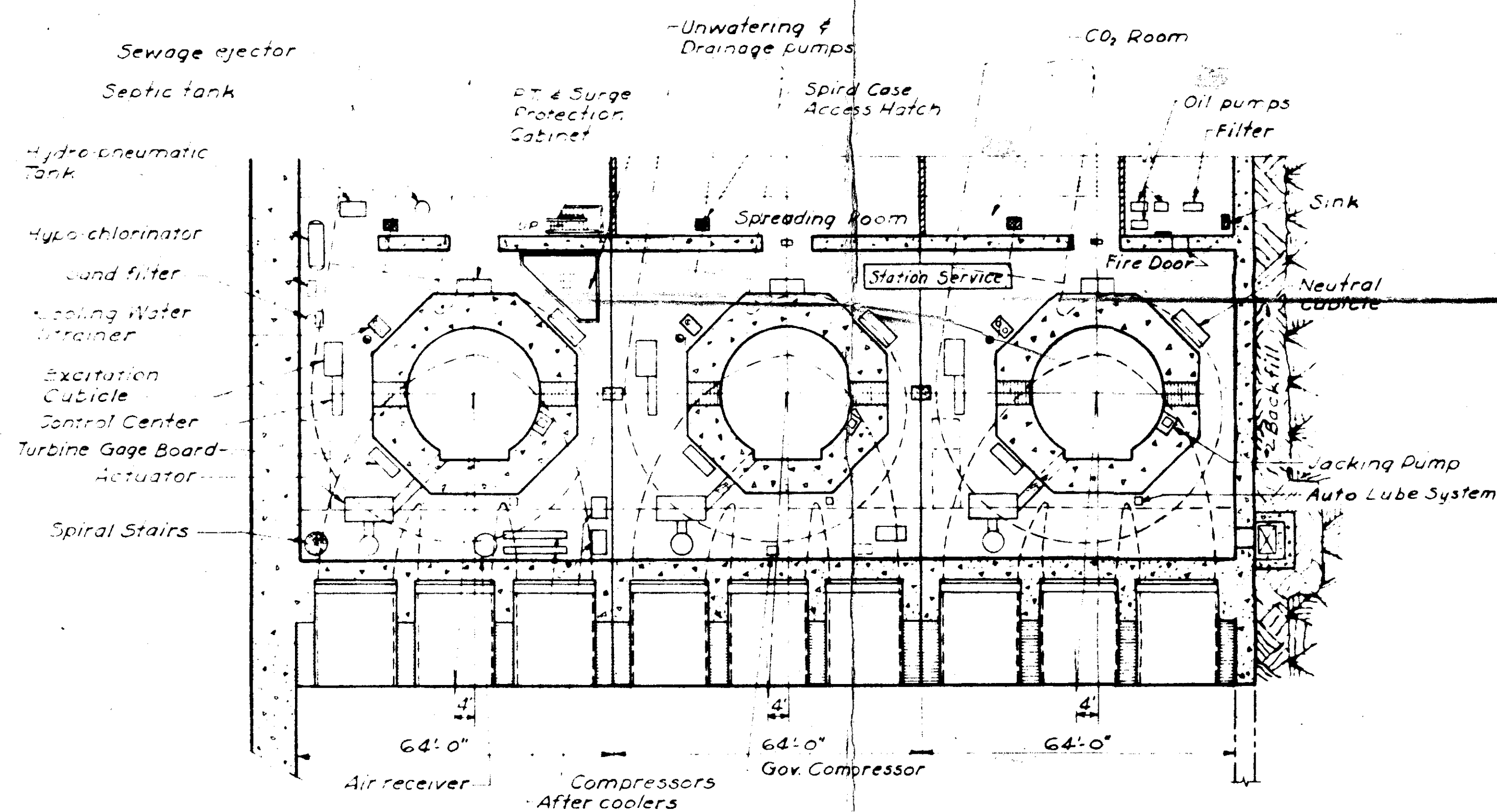
PLAN TURBINE FLOOR EL1470.0
