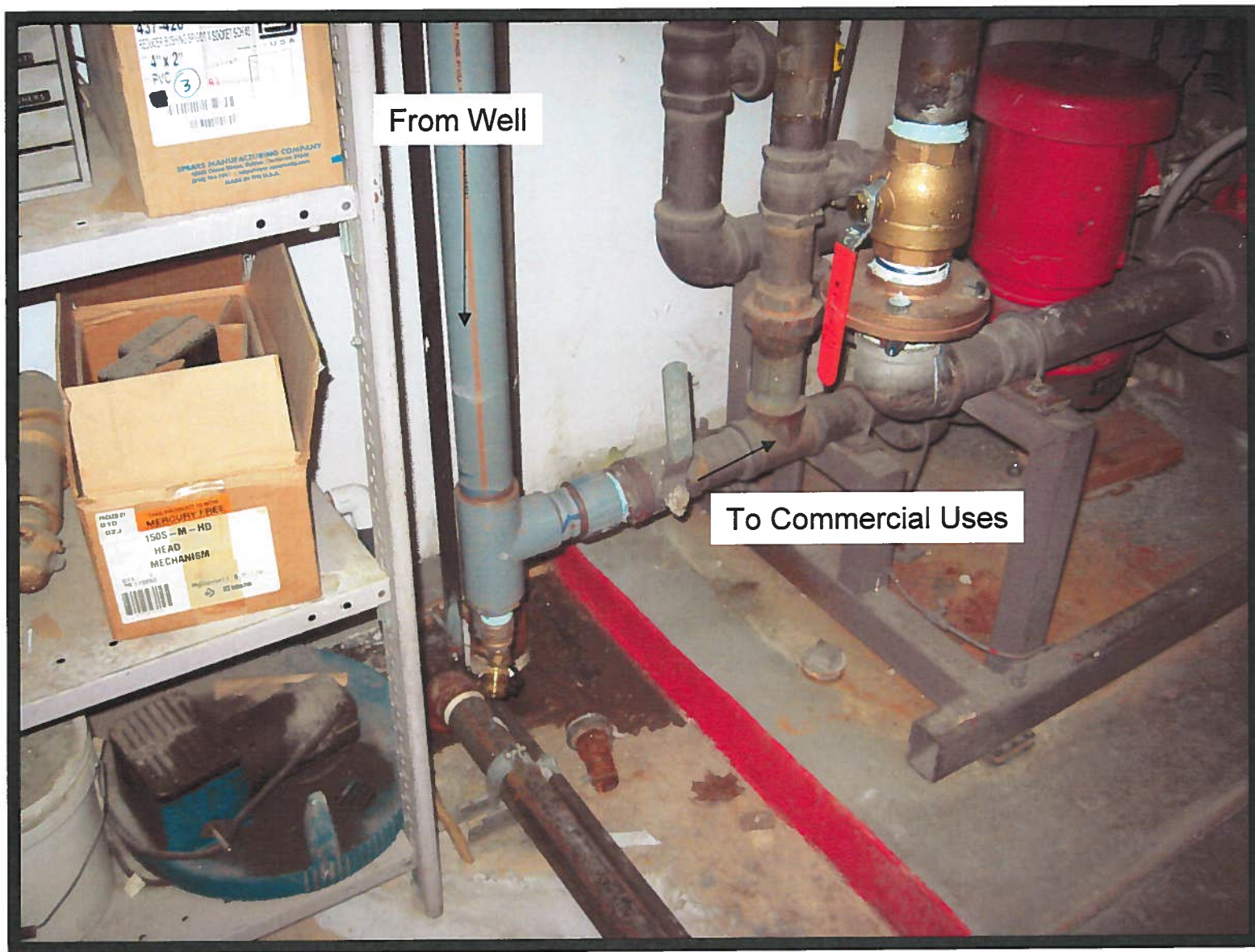
Ground Water Commercial Supply Line Connection
