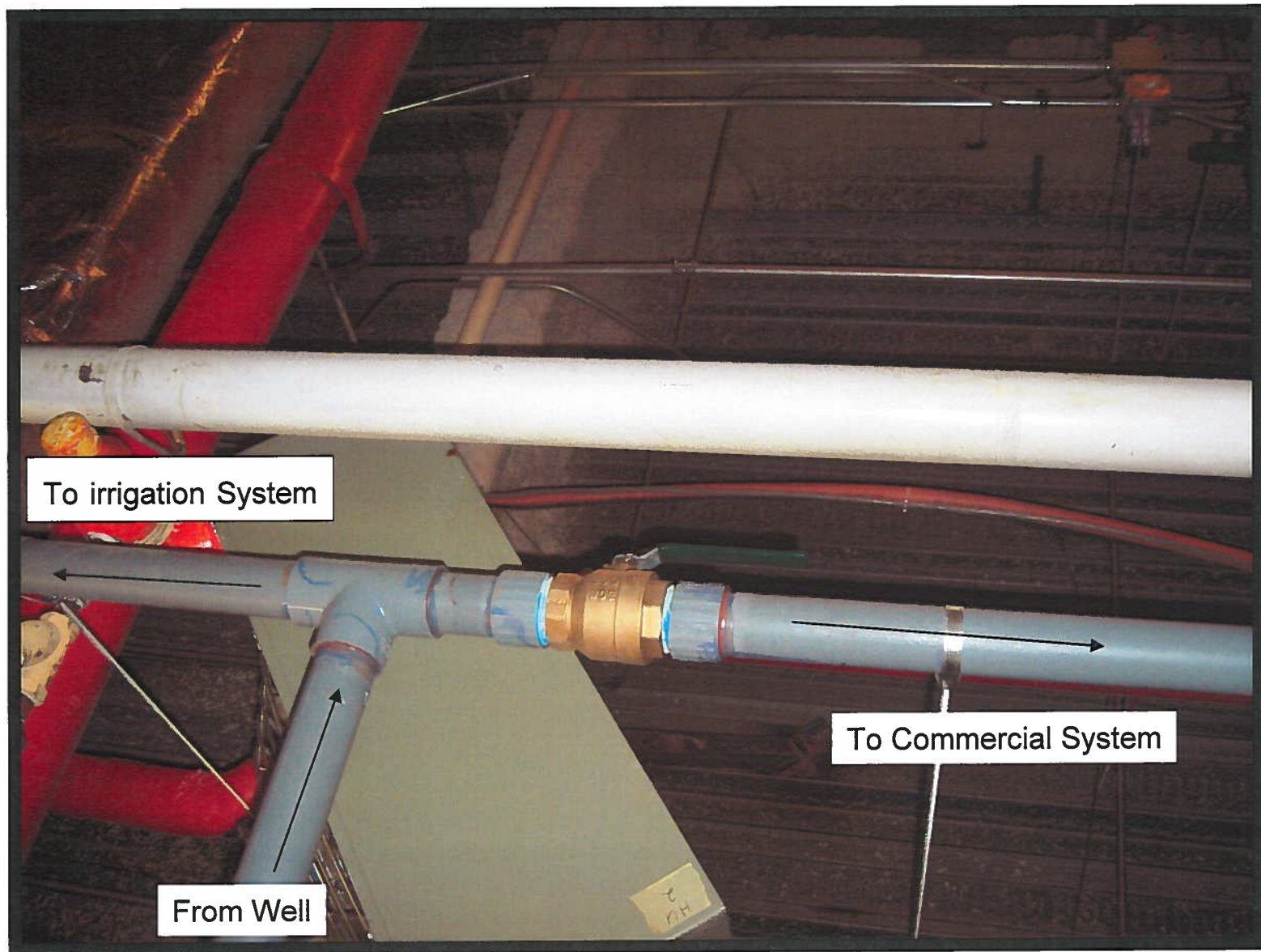
Ground Water Direction Control Valve
