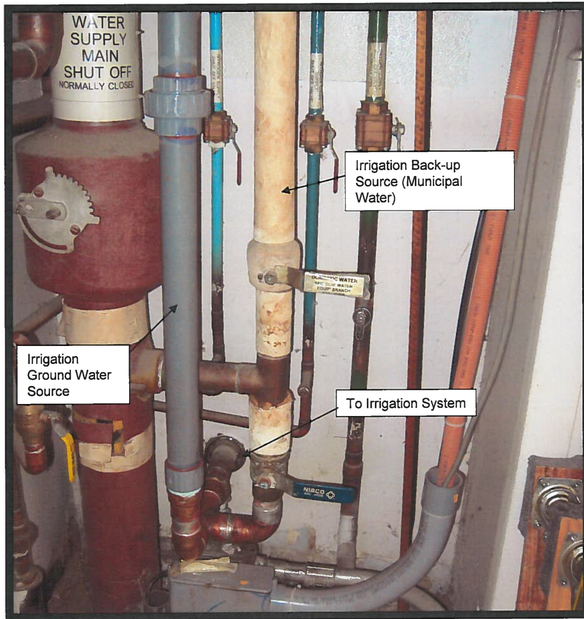
Ground Water Irrigation System Connection
