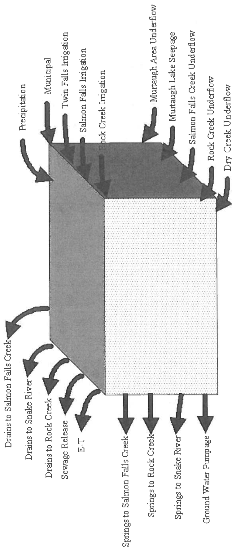
Figure 5. Water Budget Conceptual Model.
