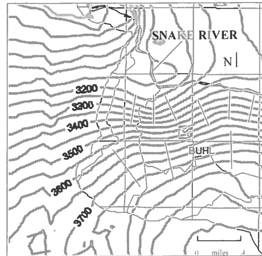
Figure 4. Ground water flow map of Buhl area showing direction of ground water flow (arrows) and equipotential lines (feet above sea level).
