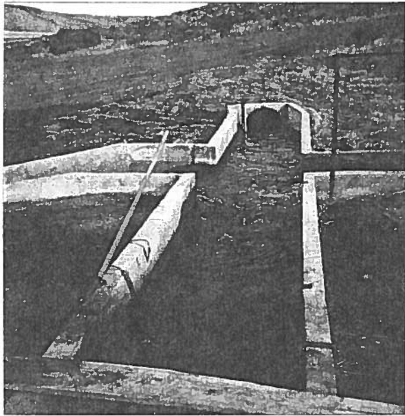
Inlet Works
