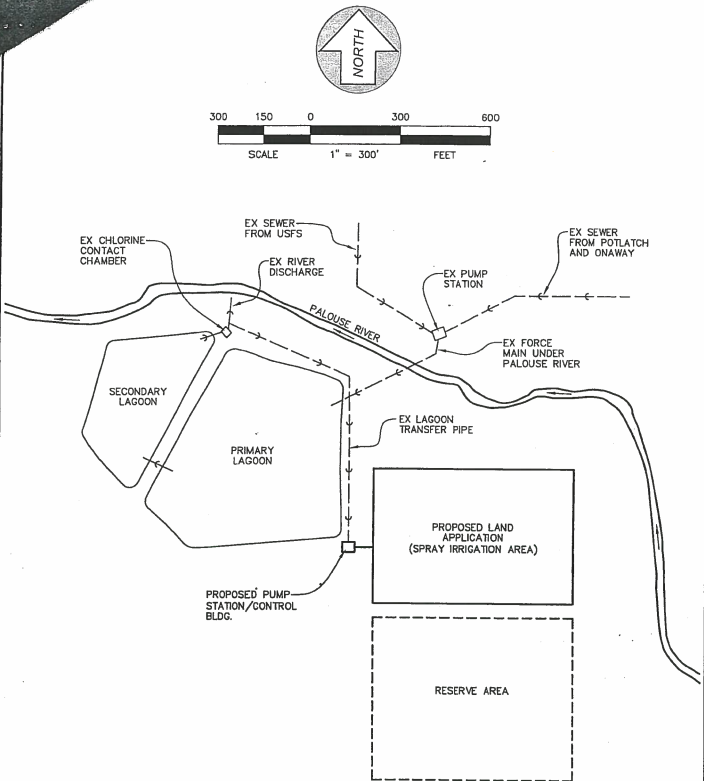
FIGURE 5 DESIGN SCHEMATIC ALTERNATIVE B RIVER DISCHARGE PLUS LAND APPLICATION ON SOUTH SIDE OF PALOUSE RIVER
