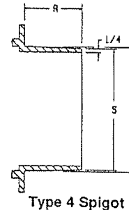
Corrugated Pipe Attached to Spigot Back Frame
