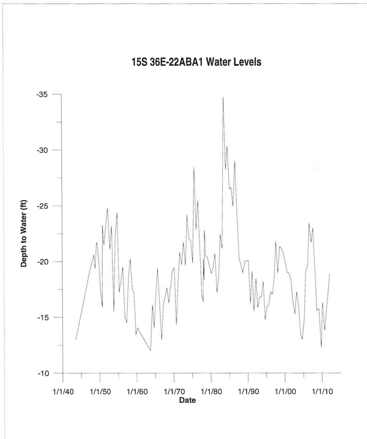
Figure 3. Water levels in well 15S 36E-22ABA1. Note that negative depths indicate that the water level is above land surface.
