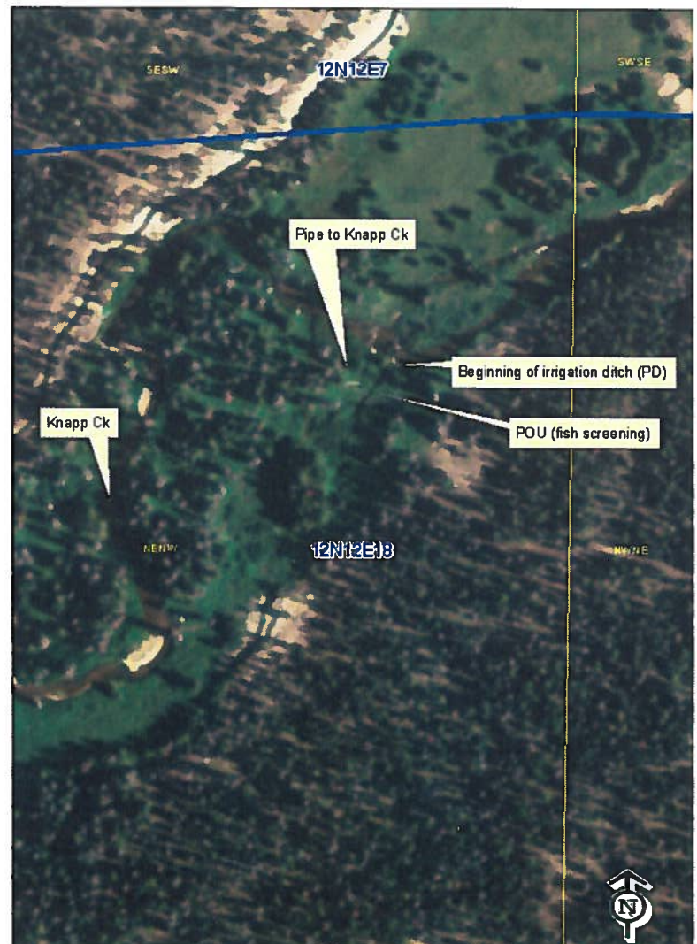
Spatial System Diagram of 77-7317
