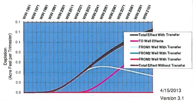
Hydrologic Response-- Malad to Bancroft Customer Name: Kitsos Transfer No:
