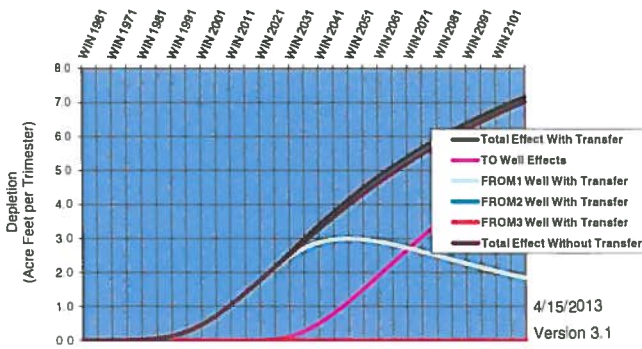
Hydrologic Response--Devil's Washbowl to Buhl Customer Name: Kitsos Transfer No:
