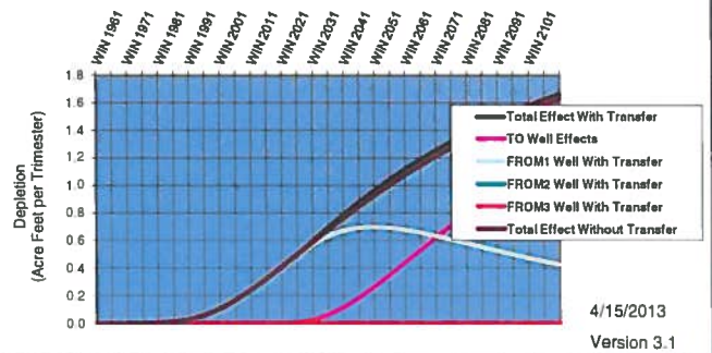
Hydrologic Response-- Malad to Bancroft Customer Name: Kitsos Transfer No:
