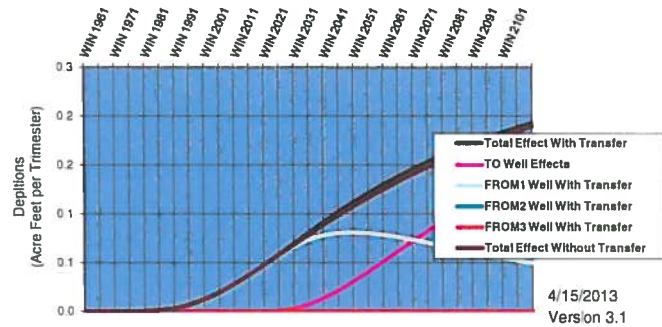
Hydrologic Response-- Malad Customer Name: Kitsos Transfer No:
