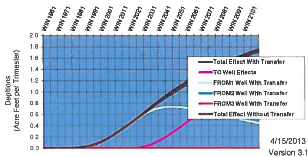
Hydrologic Response--Thousand Springs Customer Name: Kitsos Transfer No:
