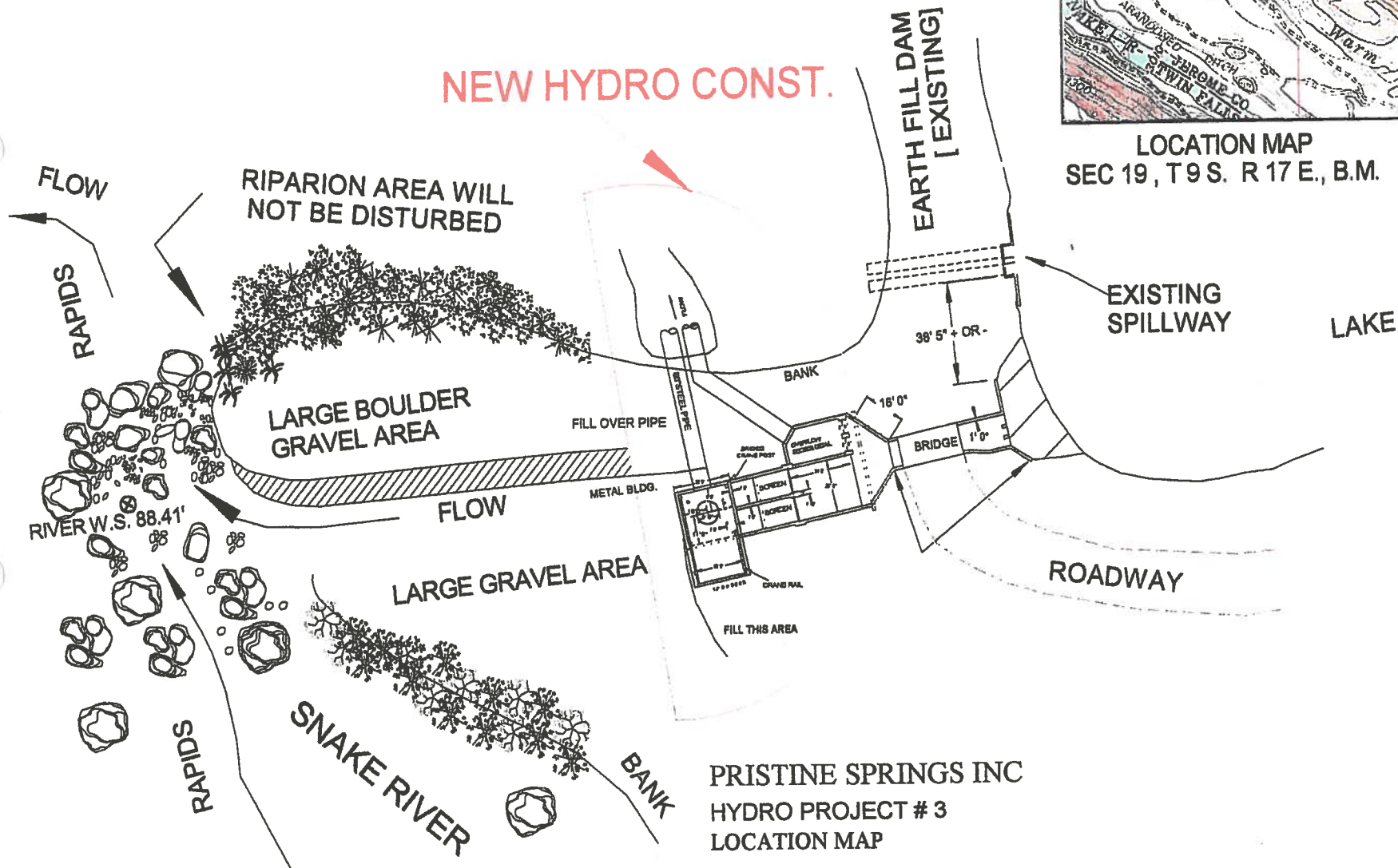
PLOT PLAN OF PROJECT IN RESPECT TO EXISTING FACILITIES AND AREA.
