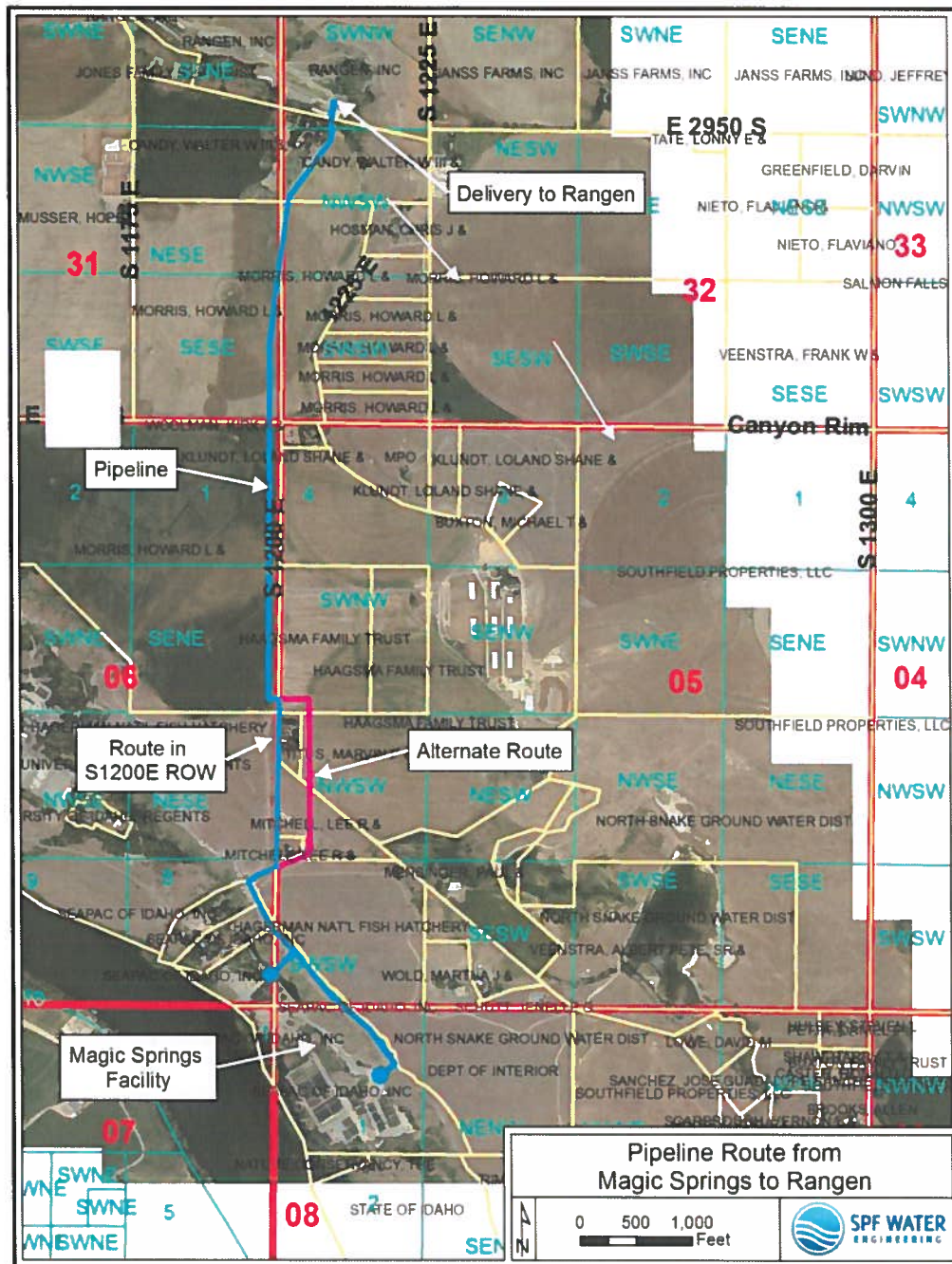
Figure 3. Pipeline Alignment
