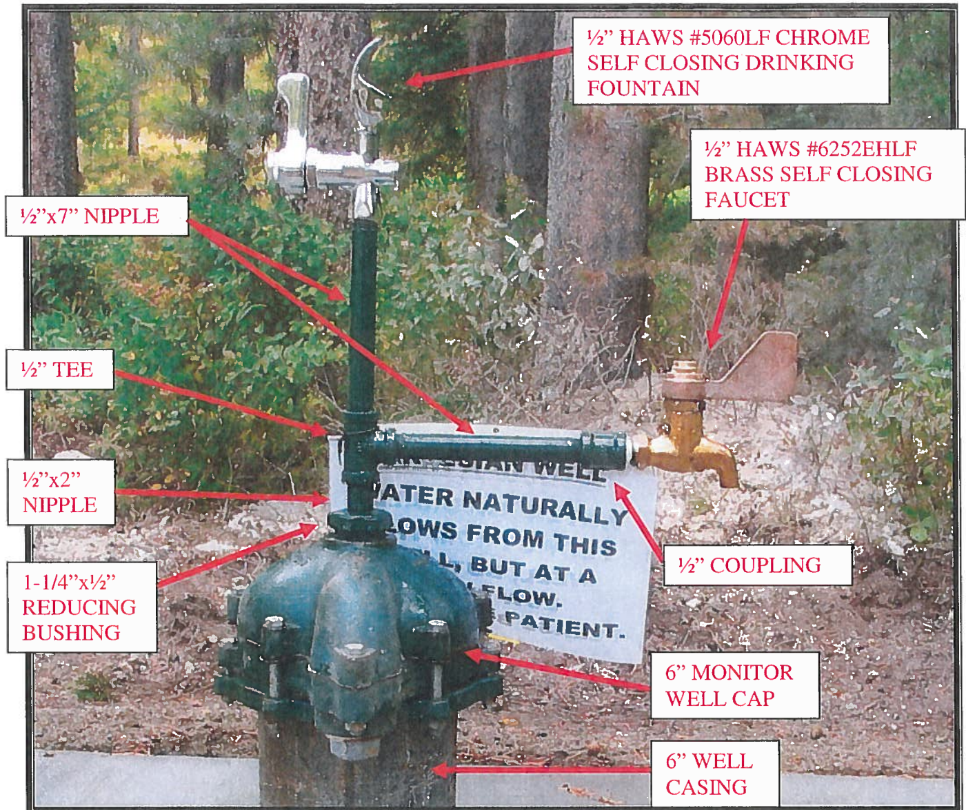
CLOSE-UP OF FAUCET/FOUNTAIN ASSEMBLY
