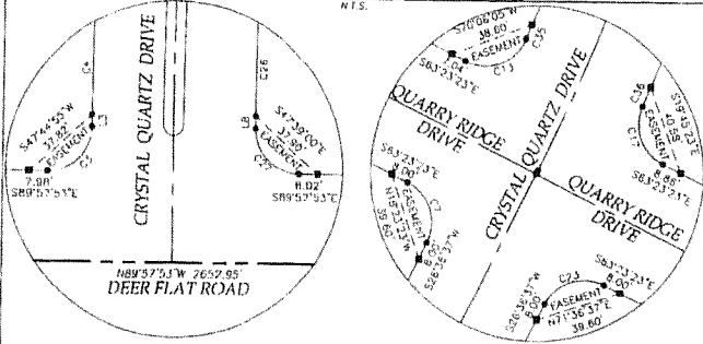
DETAIL 3 SIGHT TRIANGLE EASEMENTS NTS
