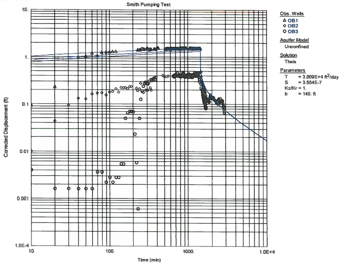
Figure 3-4 Theis unconfined solution matched to OB1
