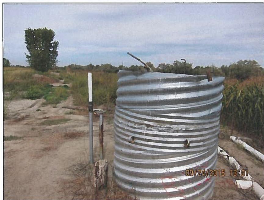
Figure 6: Lower control structure for places of use A & E.
