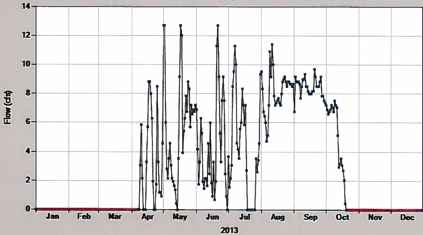
Hydrograph of 370101786 - D - MALAD RESERVOIR
