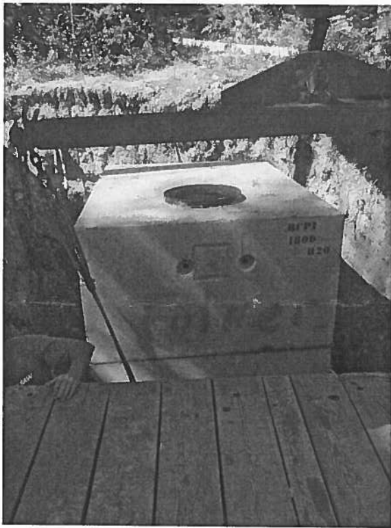
New 1,800 gallon concrete water tank being placed in previous tank location.
