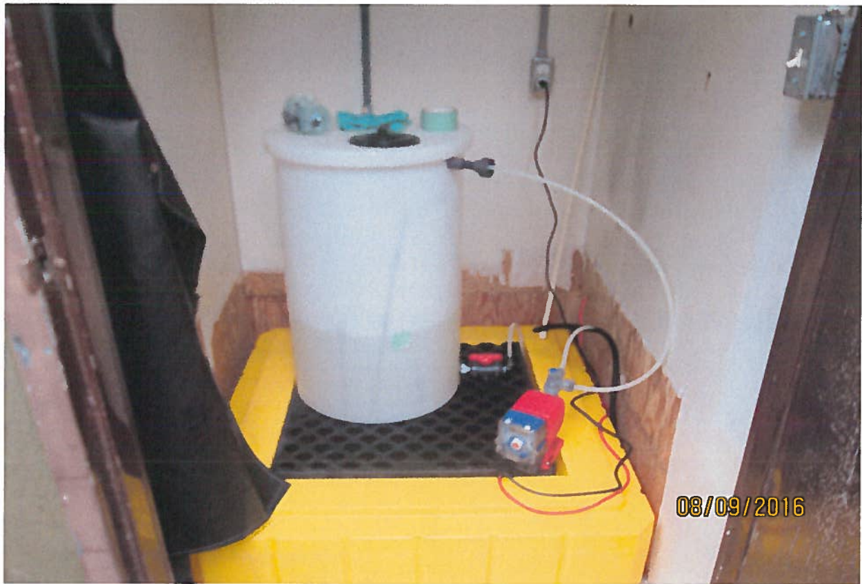
Chlorination system.
