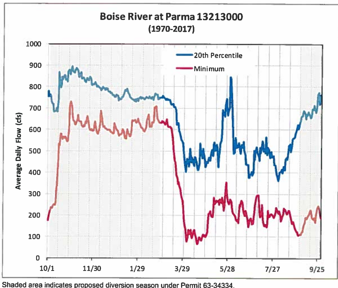
Figure 3. Boise River at Parma minimum streamflows, 1970-2017.
