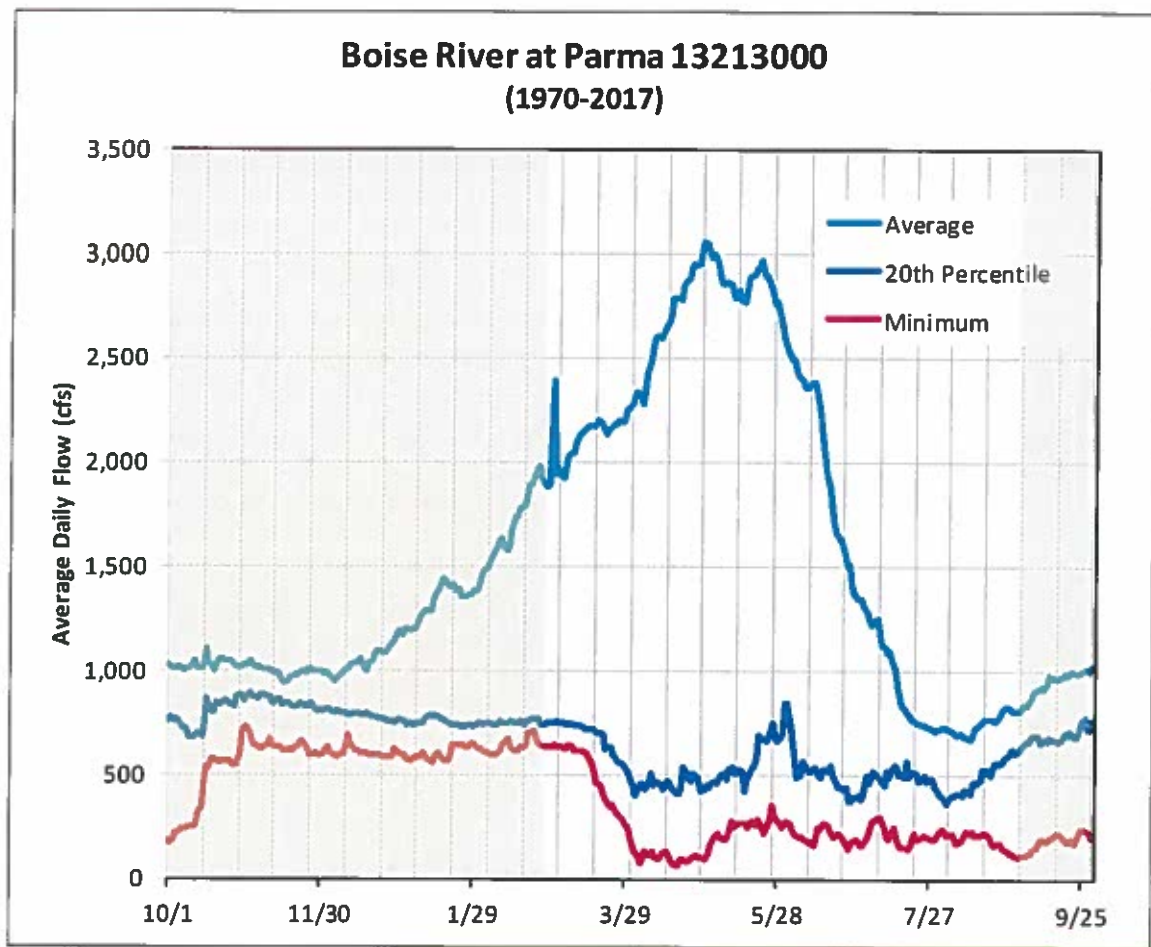
Figure 2. Boise River at Parma streamflow, 1970-2017.
