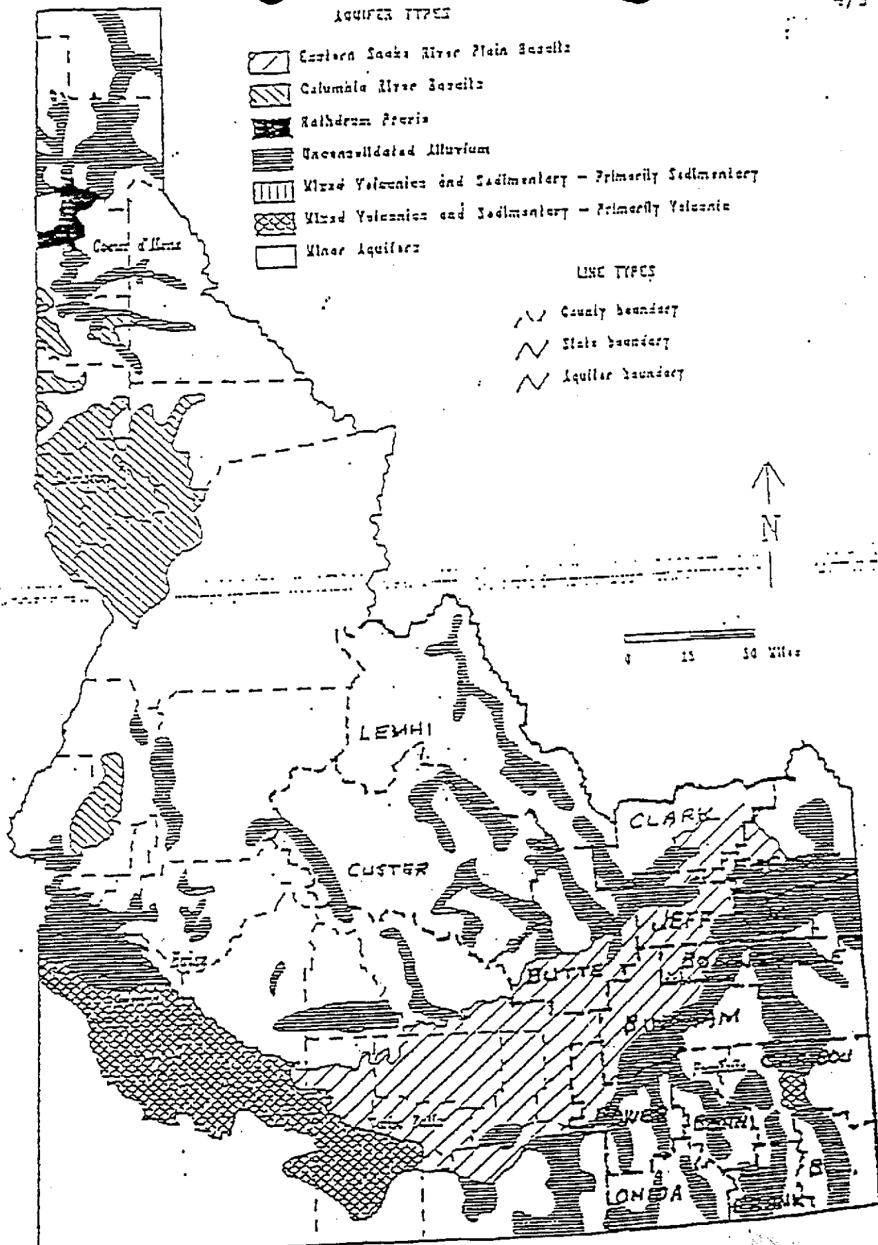
Figure 2.18a. Aquifer types in Idaho. (Copied from Well Head Protection in Idaho ; sponsored by IDHW-DEQ, in cooperation with Idaho Water Resources Institute, Univ. of Idaho.)
