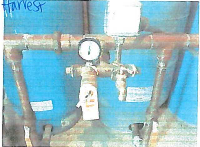
Photograph 12: Pressure gauge, pressure switch, and smooth tap
