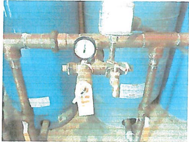
Photograph 12: Pressure gauge, pressure switch, and smooth tap
