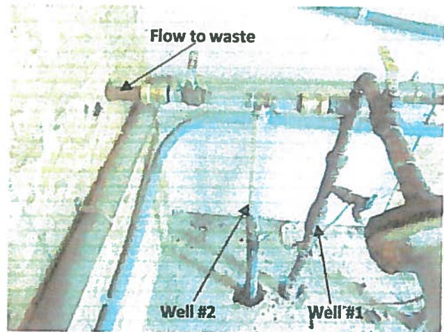
Photograph 8: Well discharge lines and flow to waste line
