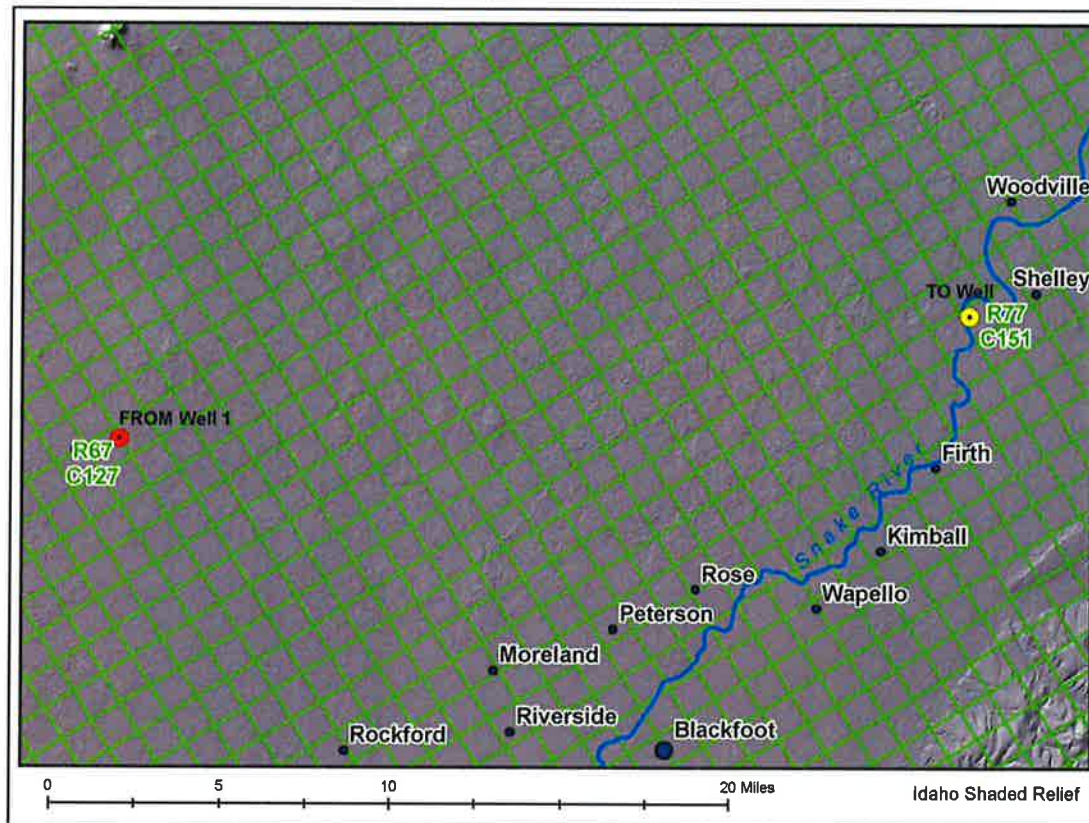
Figure 1. ESPAM Model Grids
