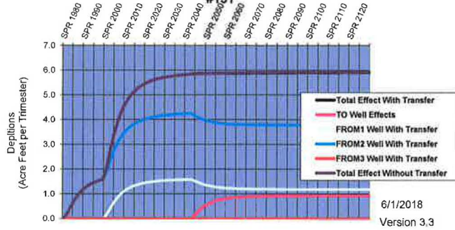
Hydrologic Response--Shelley to Near Blackfoot Customer Name: Cassia SD #151 Transfer No:
