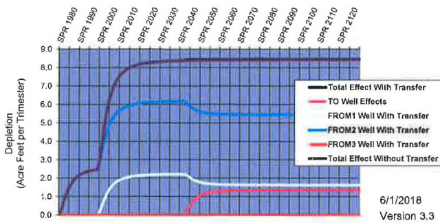
Hydrologic Response--Thousand Springs Customer Name: Cassia SD #151 Transfer No:
