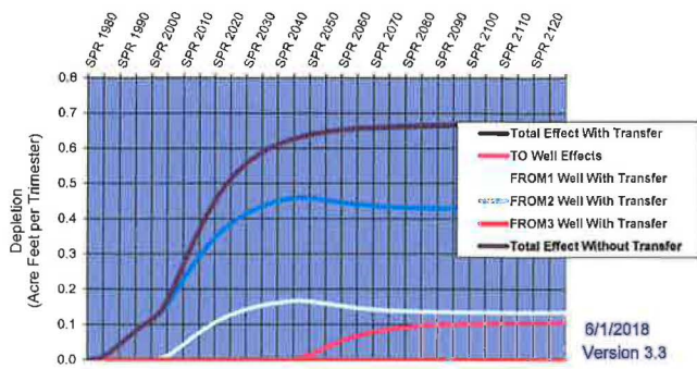
Hydrologic Response--Ashton to Rexburg Customer Name: Cassia SD #151 Transfer No:
