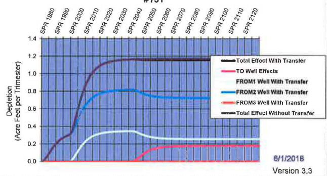
Hydrologic Response-- Neeley to Minidoka Customer Name: Cassia SD #151 Transfer No:
