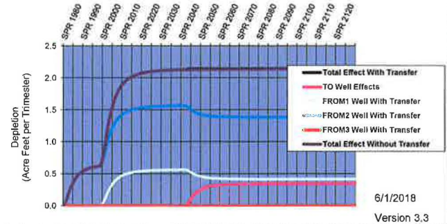
Hydrologic Response-- Malad to Bancroft Customer Name: Cassia SD #151 Transfer No:
