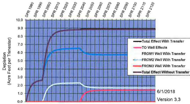
Hydrologic Response--Devil's Washbowl to Buhl Customer Name: Cassia SD #151 Transfer No:
