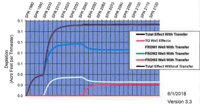
Hydrologic Response-- Malad to Bancroft Customer Name: Cassia SD #151 Transfer No:
