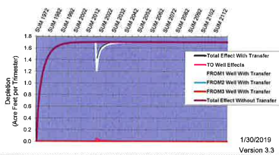
Hydrologic Response-- Neeley to Minidoka Customer Name: Heritage Transfer No: 1216
