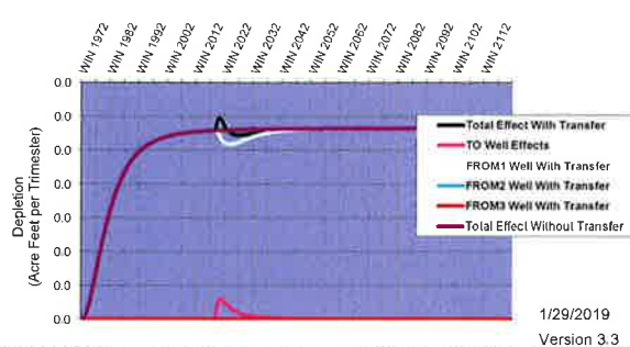
Hydrologic Response-- Malad to Bancroft Customer Name: Heritage Farms Transfer No: 1216 &
