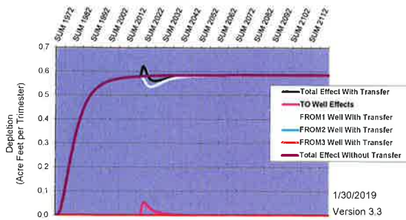
Hydrologic Response--Devil's Washbowl to Buhl Customer Name: Heritage Farms Transfer No: 1216
