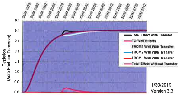
Hydrologic Response--Ashton to Rexburg Customer Name: Heritage Farms Transfer No: 1216
