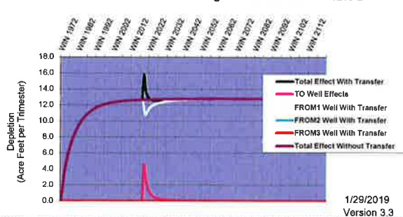
Hydrologic Response--Neeley to Minidoka Customer Name: Heritage Farms Transfer No: 1216 &
