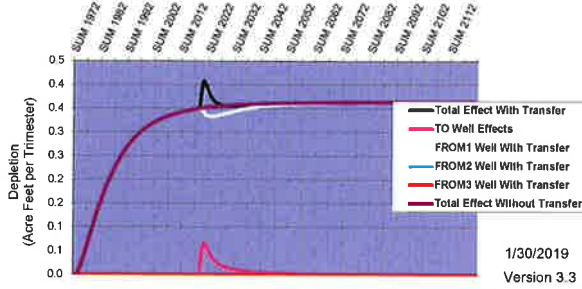
Hydrologic Response--Shelley to Near Blackfoot Customer Name: Heritage Transfer No: 1216
