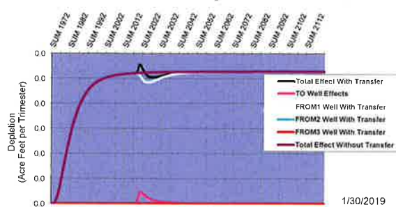
Hydrologic Response-- Malad to Bancroft Customer Name: Heritage Farms Transfer No: 1216
