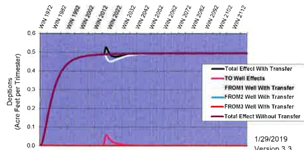
Hydrologic Response--Thousand Springs to Malad Customer Name: Heritage Farms Transfer No: 1216 &
