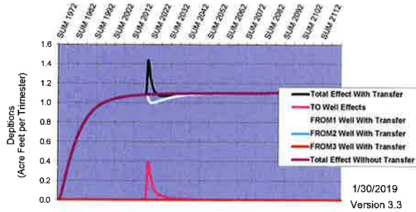
Hydrologic Response--Shelley to Near Blackfoot Customer Name: Heritage Transfer No: 1216
