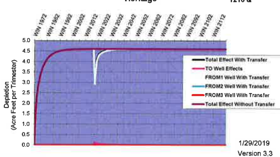
Hydrologic Response--Neeley to Minidoka Customer Name: Heritage Farms Transfer No: 1216 &
