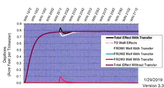
Hydrologic Response--Thousand Springs Customer Name: Heritage Farms Transfer No: 1216 &
