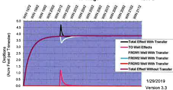
Hydrologic Response--Shelley to Near Blackfoot Customer Name: Heritage Farms Transfer No: 1216 &
