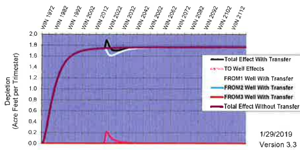
Hydrologic Response--Thousand Springs Customer Name: Heritage Farms Transfer No: 1216 &
