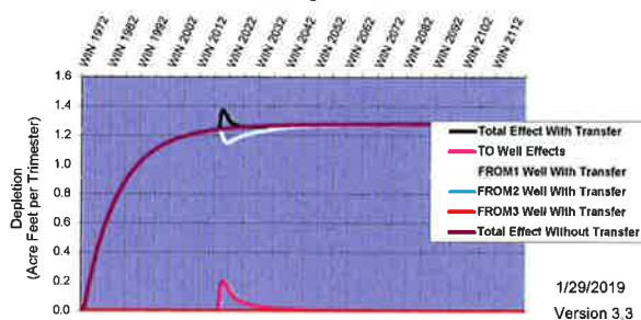
Hydrologic Response--Shelley to Near Blackfoot Customer Name: Heritage Farms Transfer No: 1216 &
