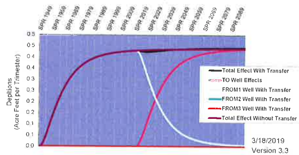
Hydrologic Response-- Malad Customer Name: F&G 2.0 cfs Transfer No:
