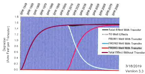
Hydrologic Response--Thousand Springs Customer Name: F&G 2.0 cfs Transfer No:
