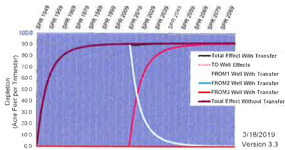
Hydrologic Response--Ashton to Rexburg Customer Name: F&G 2.0 cfs Transfer No:
