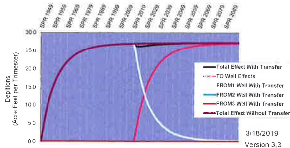
Hydrologic Response--Shelley to Near Blackfoot Customer Name: F&G 2.0 cfs Transfer No:
