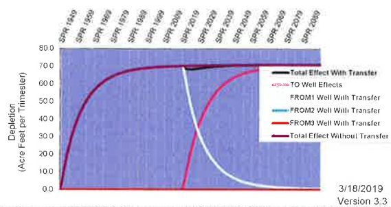
Hydrologic Response--Neeley to Minidoka Customer Name: F&G 2.0 cfs Transfer No:
