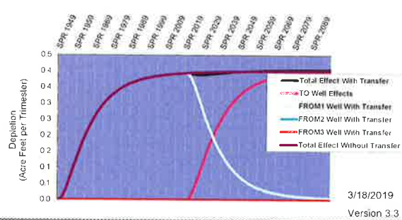
Hydrologic Response-- Malad to Bancroft Customer Name: F&G 2.0 cfs Transfer No:
