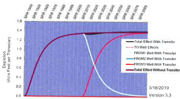
Hydrologic Response--Devil's Washbowl to Buhl Customer Name: F&G 2.0 cfs Transfer No:
