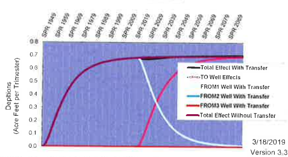
Hydrologic Response--Thousand Springs Customer Name: F&G 2.0 cfs Transfer No:
