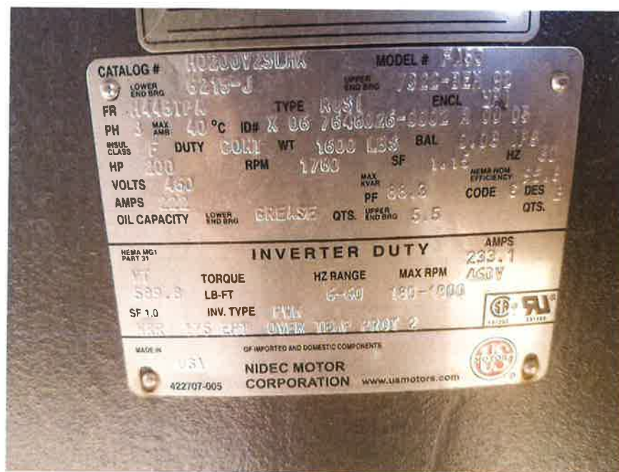
Figure 8: Well 4 motor nameplate.
