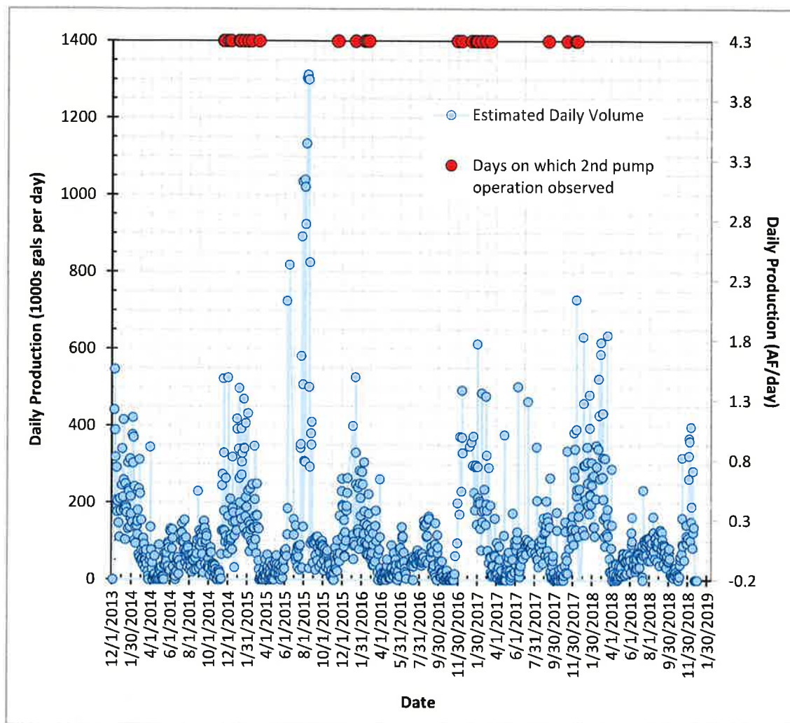
Figure 1. Hailey Fox Acres Campus estimated daily heating/cooling volume, estimated average daily flow, and observed flow (12/5/2013 through 12/30/2018).
