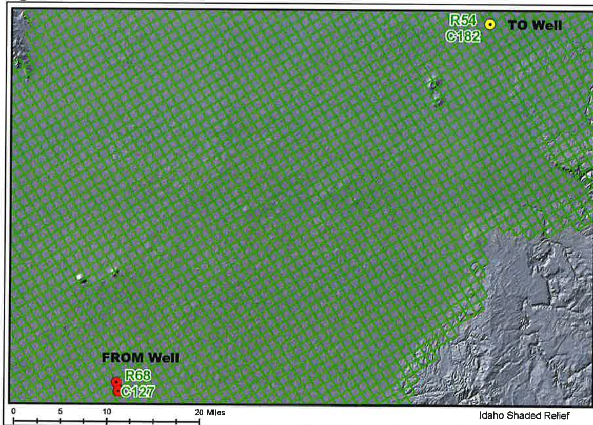
Figure 1. ESPAM Model Grids
