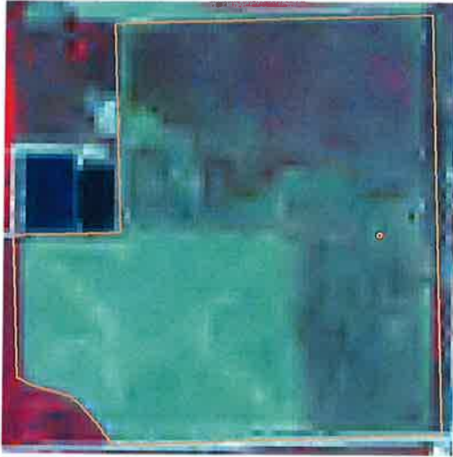
Sentinel – June 25, 2018
