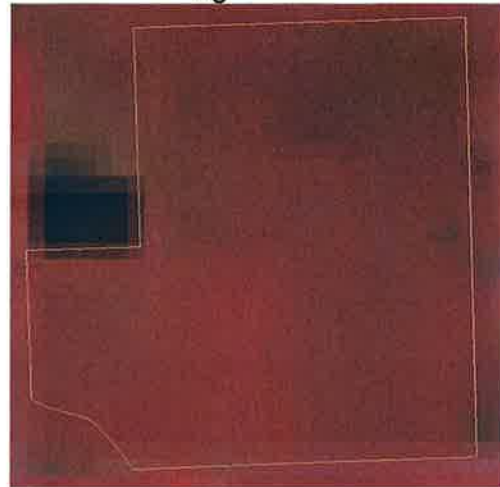
Landsat – April 28, 2015
