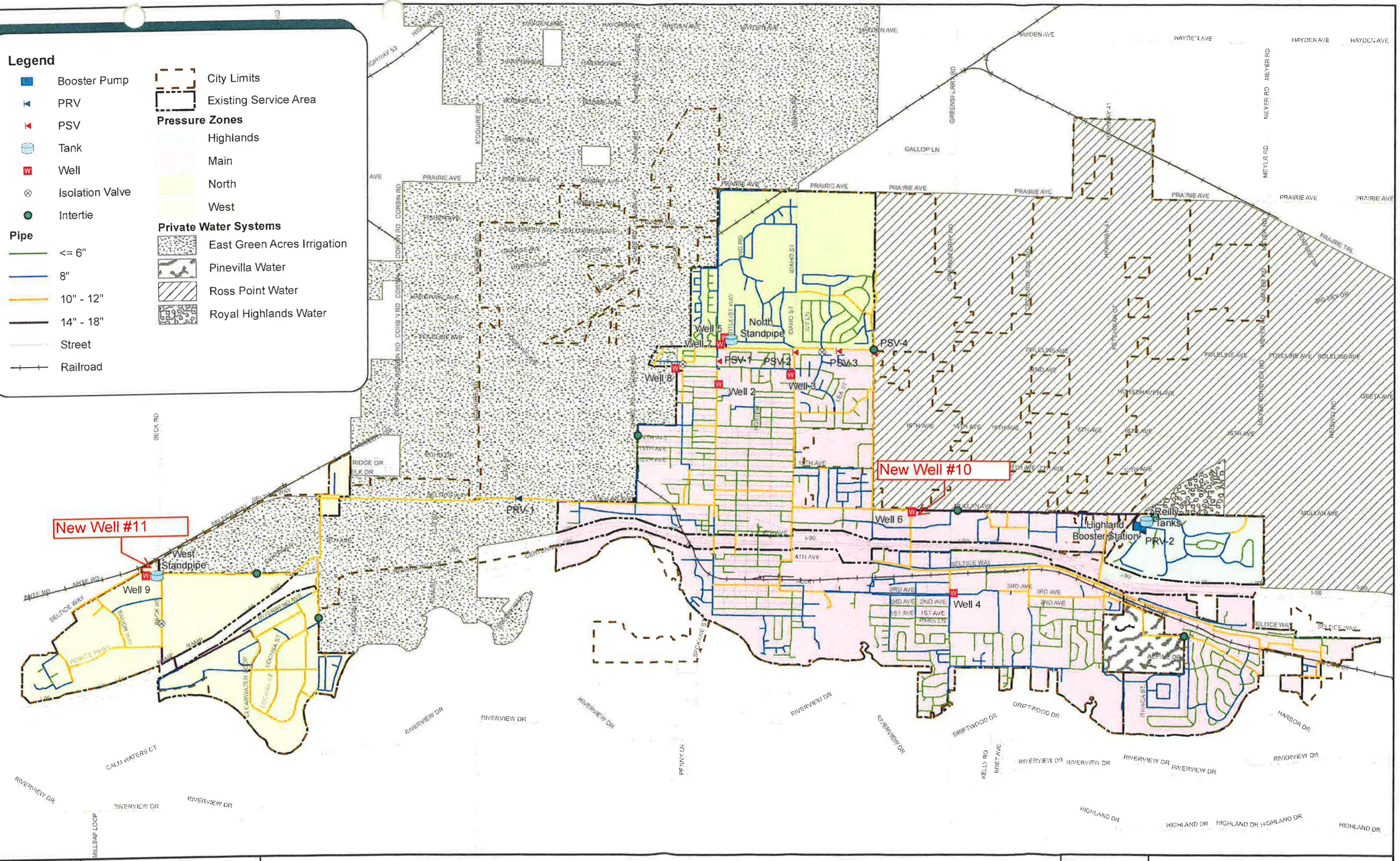
Figure 1-2 Existing System
