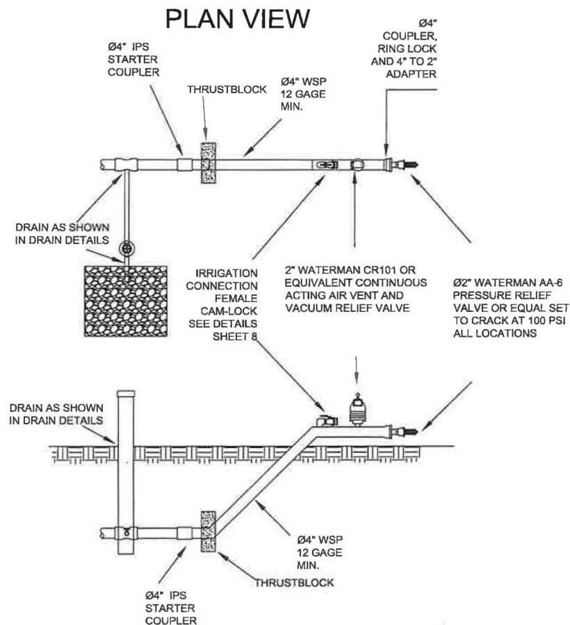
SECTION VIEW
