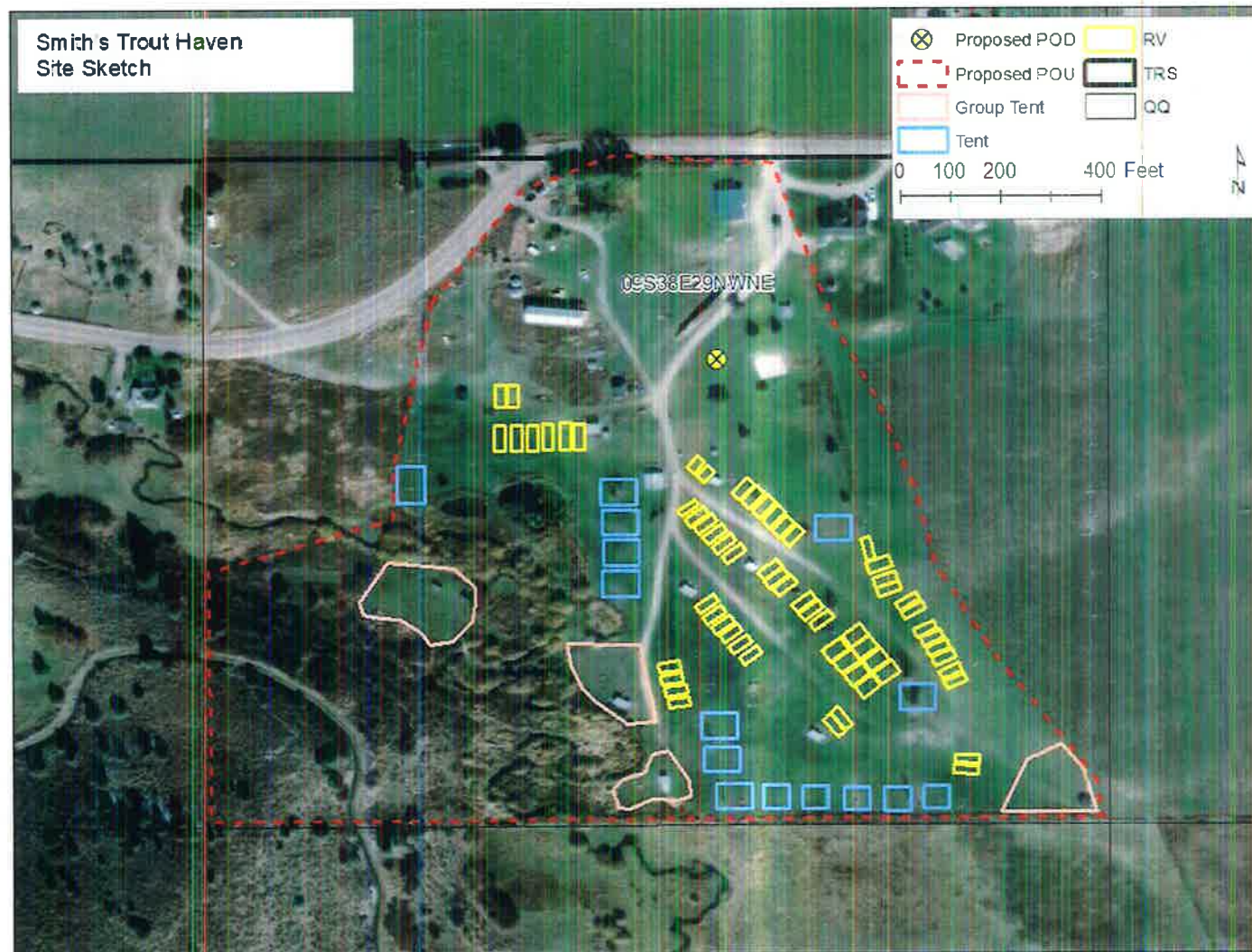
Figure 2: Site Layout and Proposed Well Location
