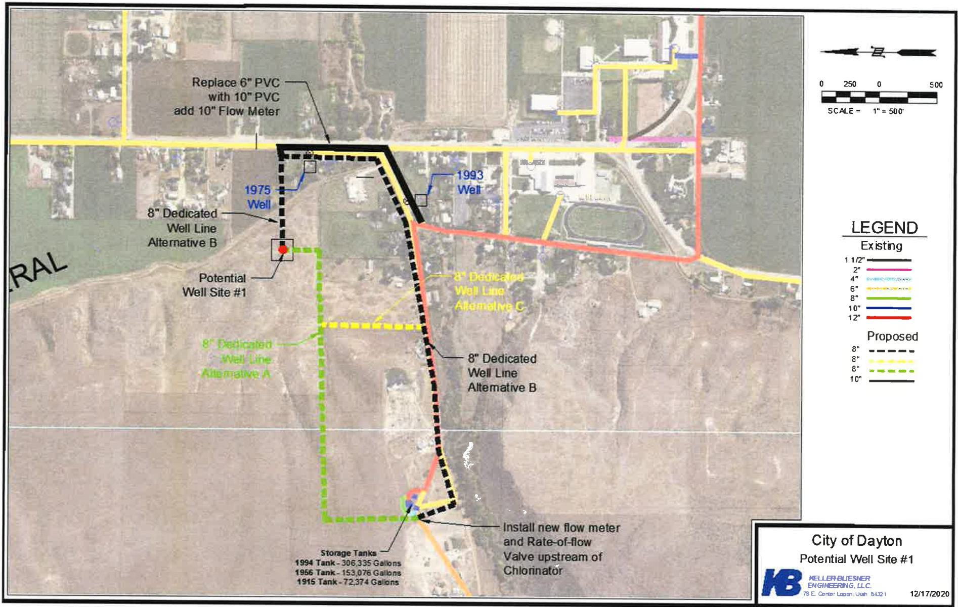
Exhibit 2a Potential Well Site #1 Conceptual Plan showing Proposed Improvement and Plans
