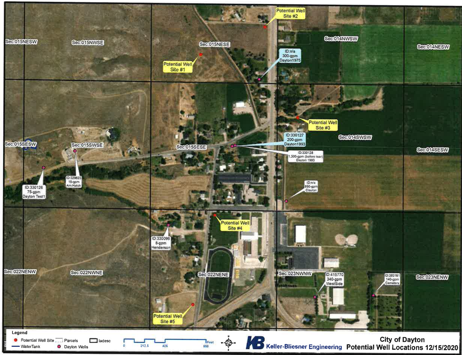
Exhibit 1a Location of Potential Well Sites
