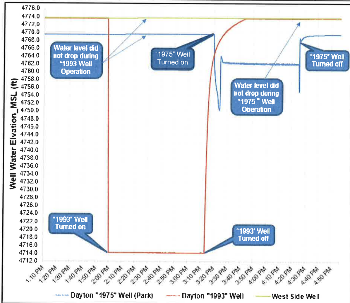
Figure 5.2 Dayton Dynamic Well Drawdown Test Results comparing "1993 Well", "1975 Well, & West Side Well water levels.– 12/18/2020
