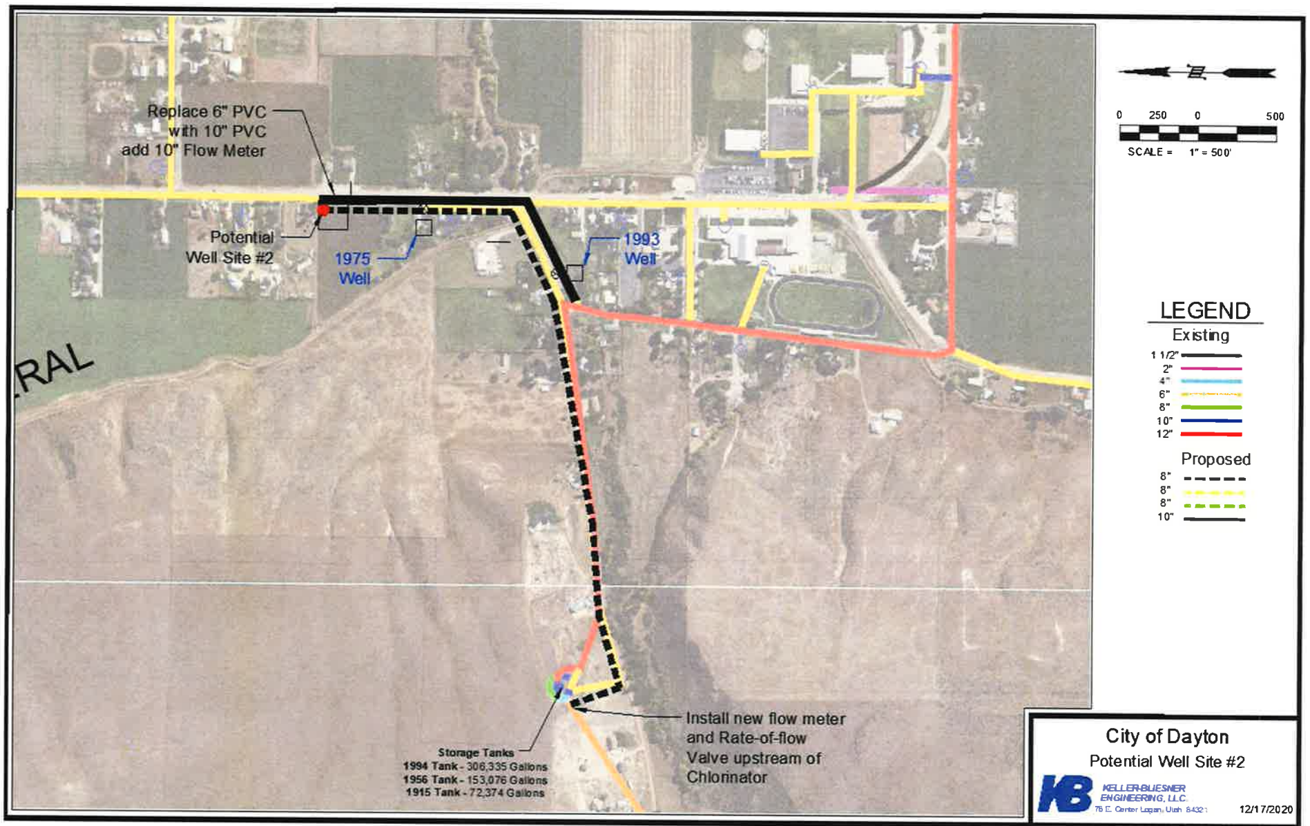
Exhibit 2b Potential Well Site #2 Conceptual Plan showing Proposed Improvement and Plans
