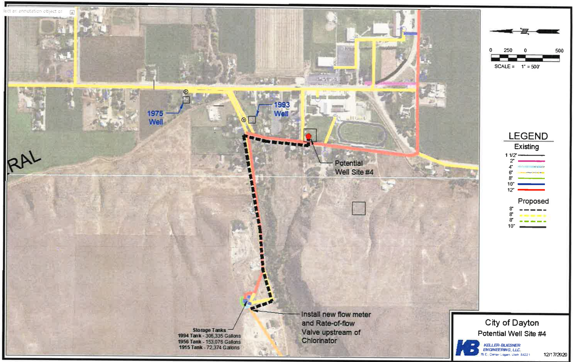
Exhibit 2d Potential Well Site #4 Conceptual Plan showing Proposed Improvement and Plans
