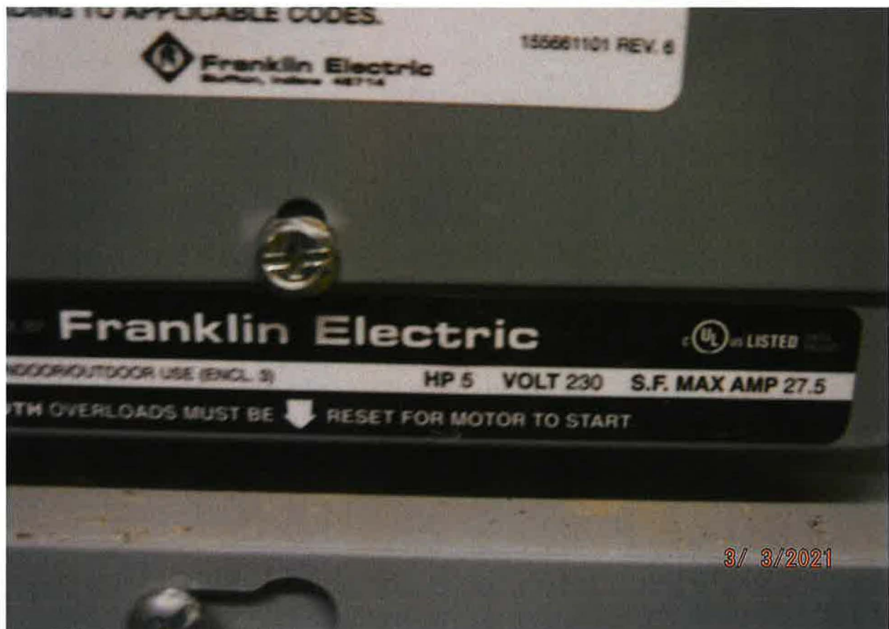
5 HP PUMP MOTOR INSTALLED IN WELL
