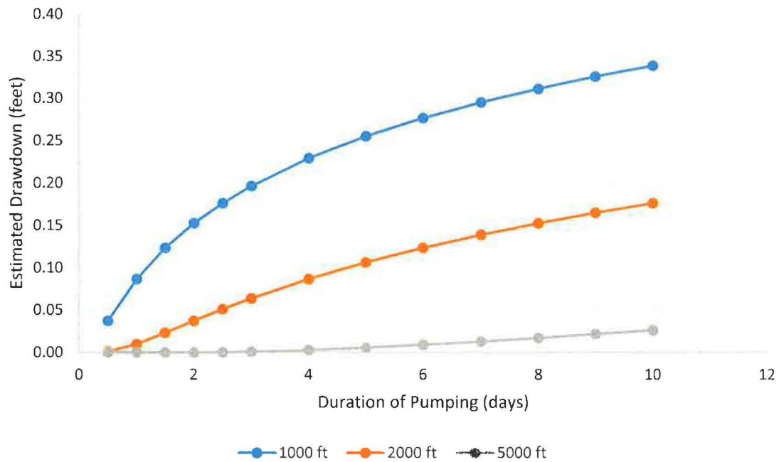
Figure 2. Estimated drawdown with time for select distances from the new point of diversion. Note: Pumping rate: 2.24 cfs; Transmissivity: 120,000 ft 2 /day; Storativity: 0.2.
