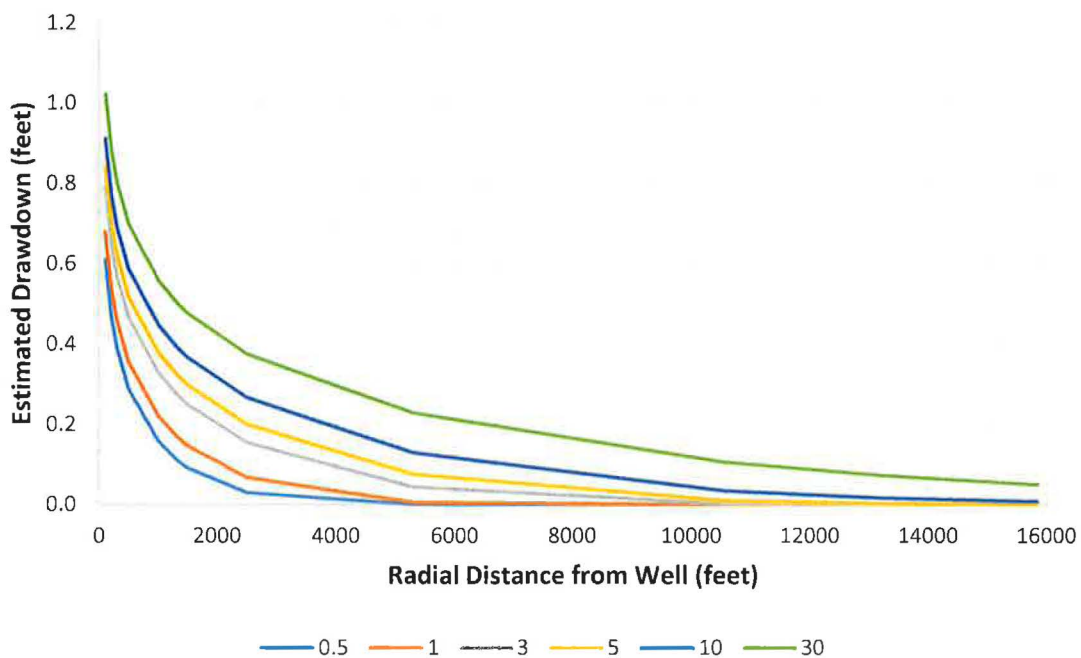
Figure 3. Estimated drawdown with distance from the new point of diversion for select pumping durations (in days). Note: Pumping rate: 5.5 cfs; Transmissivity: 375,000 ft 2 /day; Storativity: 0.1.
