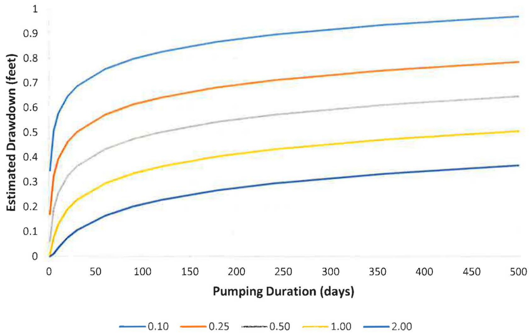
Figure 2. Estimated drawdown with time for select distances from the new point of diversion. Note: Pumping rate: 5.5 cfs; Transmissivity: 375,000 ft 2 /day; Storativity: 0.1.
