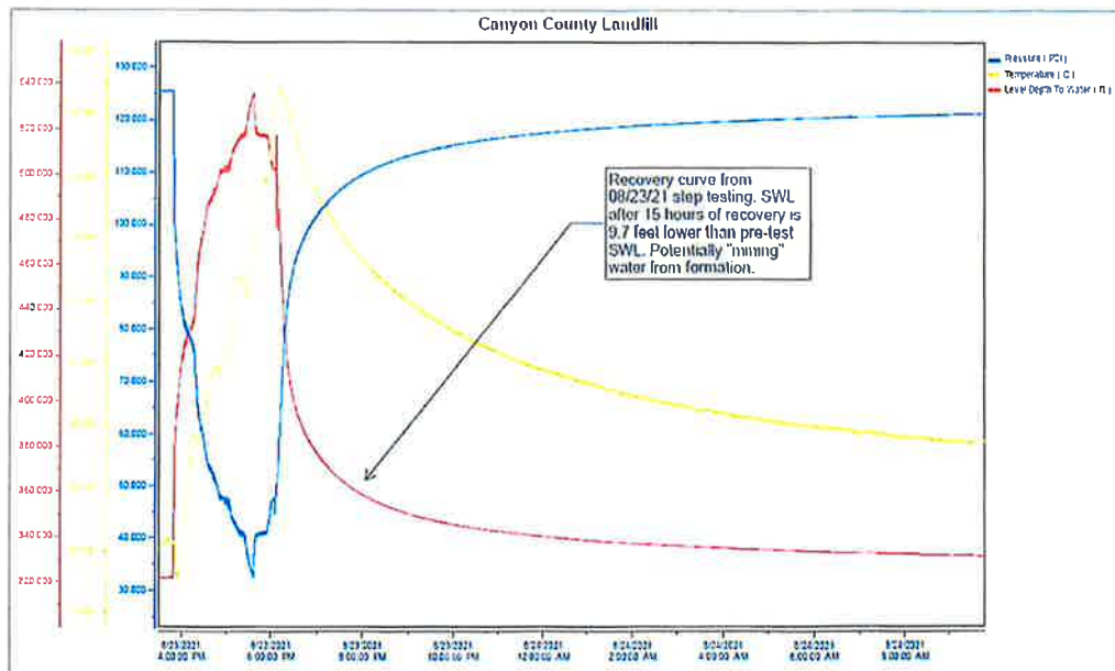
Figure 2: Step-Test Recovery Curve
