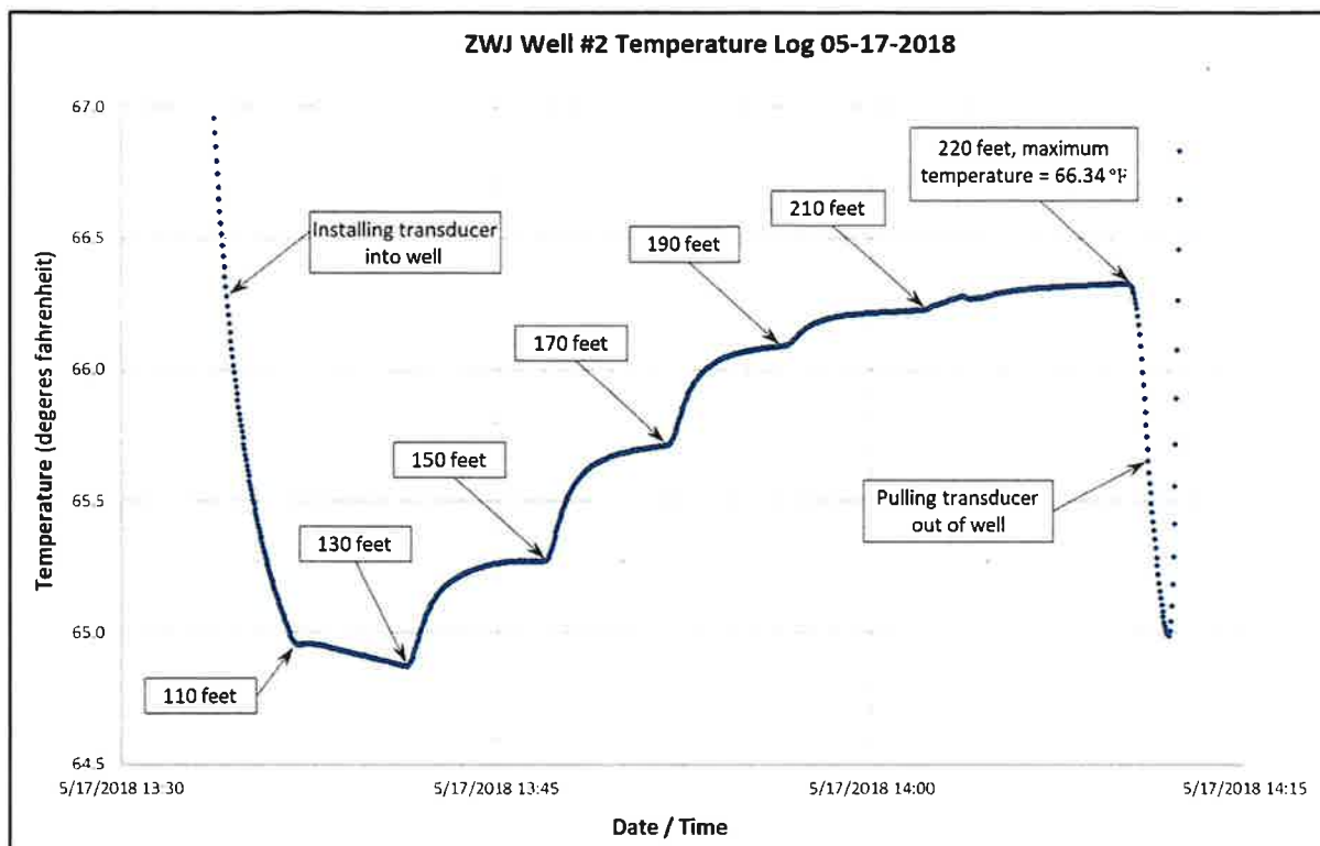
Figure 3. Well Temperature Profile Data
