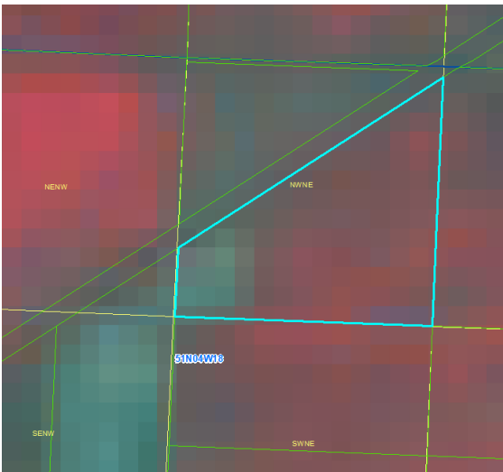
6/18/2015 LandSat
