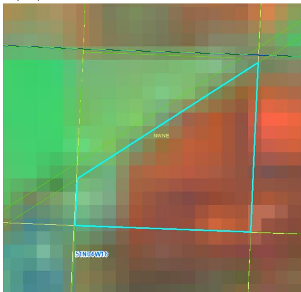
7/17/2014 LandSat
