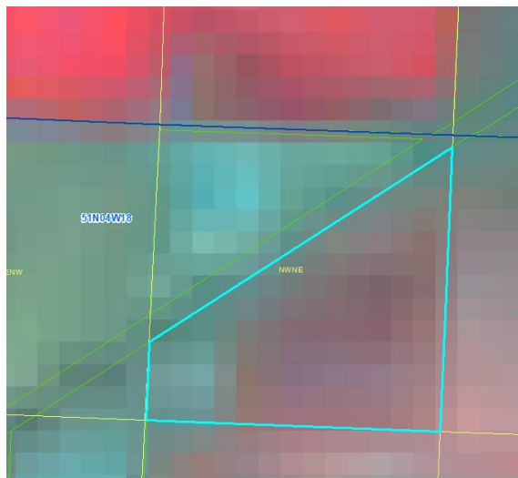
4/28/2020 LandSat
