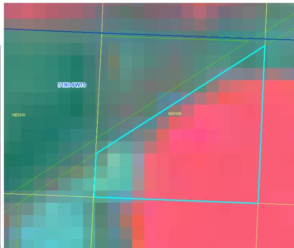
5/22/2017 LandSat
