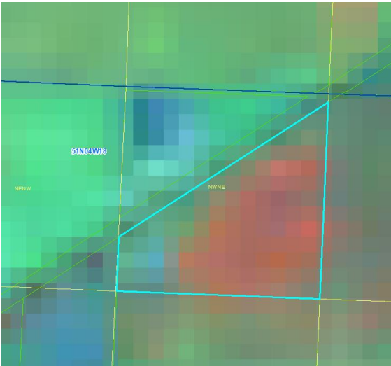
6/13/2019 LandSat
