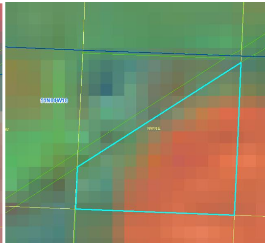
6/26/2018 LandSat
