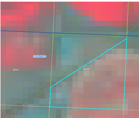
8/13/2018 LandSat
