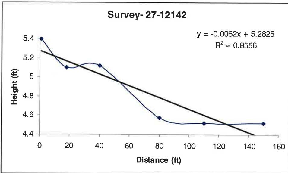
Figure 1: Graph showing the slope of the ditch from the upstream culvert running under road to the downstream end of culvert, through the fence, and out into the irrigated field. (slope = 0.0062)
