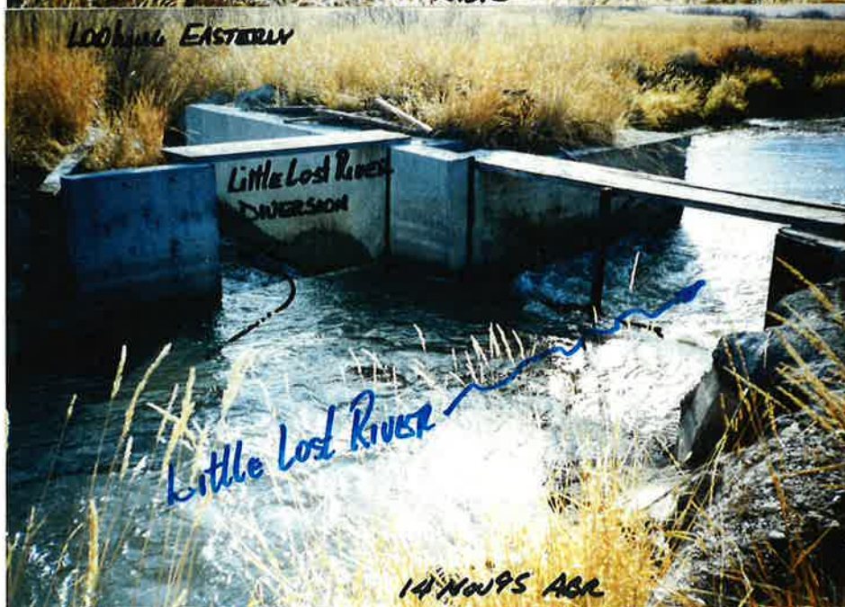
Photo 3. Little Lost River DIVERSION FOR WINTER USE. CONVEYANCE TO THE PLACE OF USE IS BY OPEN DITCH.
