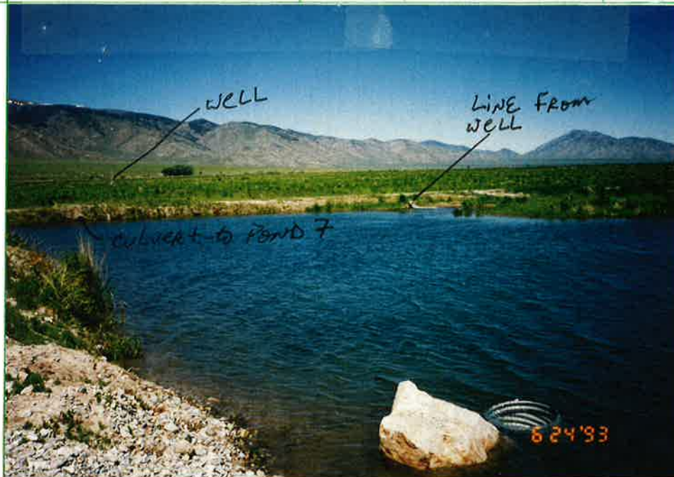
(7) View of Pond 5 From DAM. W/ WELL Discharging water to Pond, culvert to Pond 7, AND stand pipe spilling water to Pond 6.
