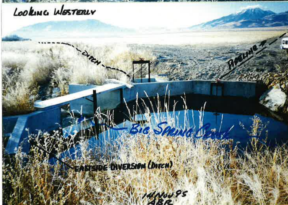
Photo 2. A WESTERLY VIEW OF THE THREE DIVERSIONS IN Photo 1. NOTE THE BURIED PIPELINE TRACE. THERE ARE NO OUTLETS OR DIVERSIONS FROM THIS PIPELINE.
